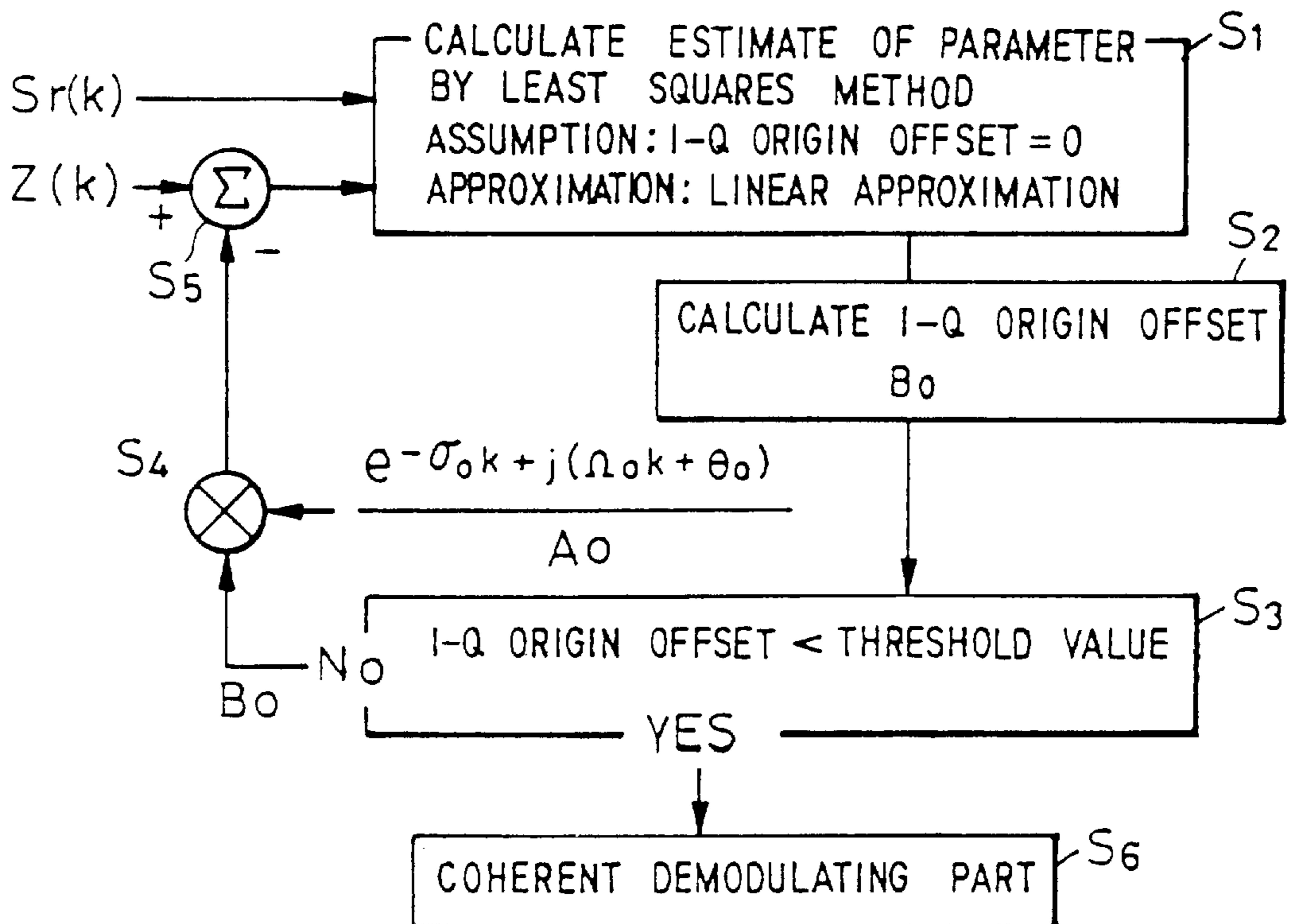
FIG. 3 PRIOR ART
