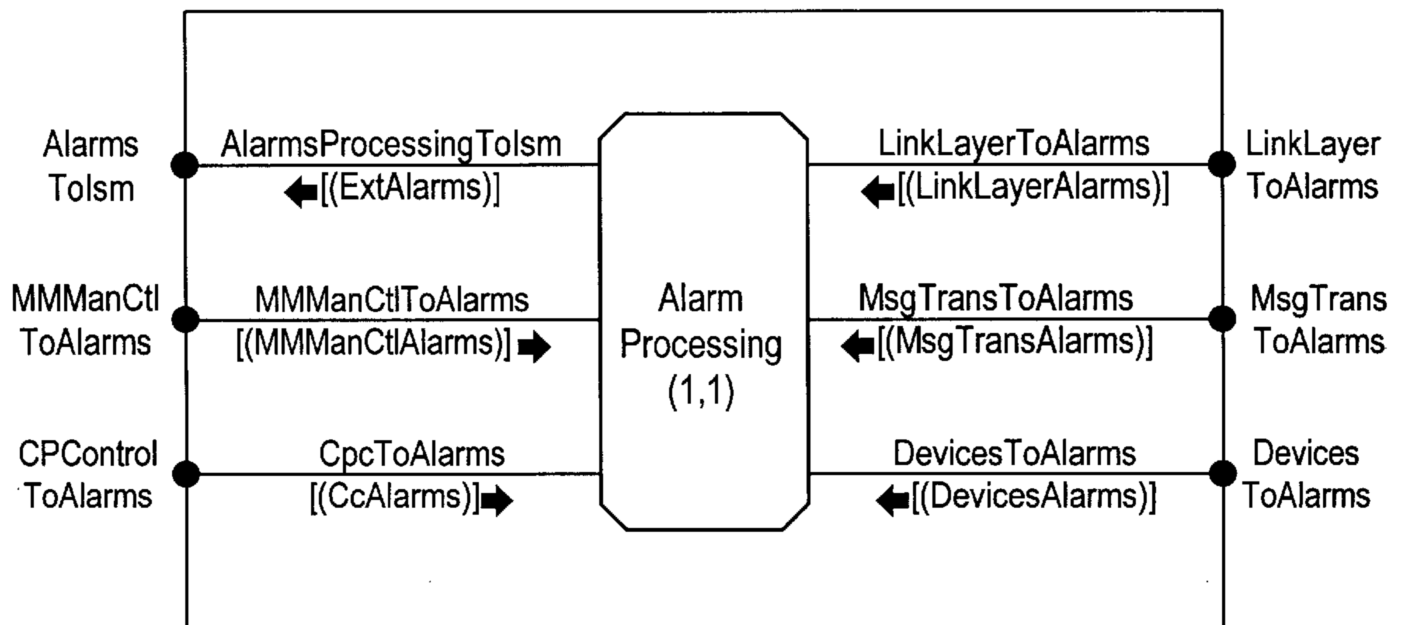
BLOCK MMMan/Admin/Alarms
