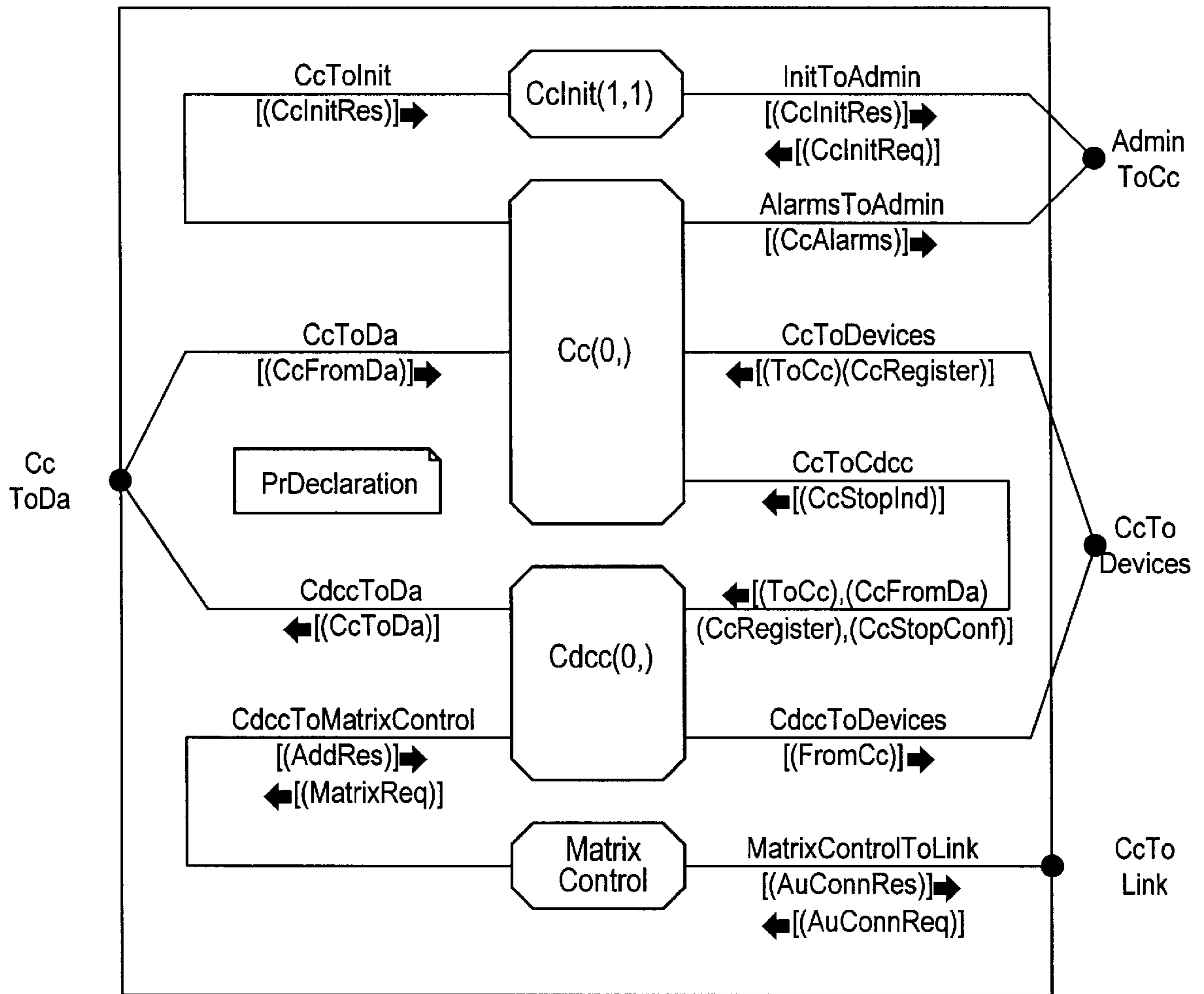
BLOCK MMMan/CPControl/CallControl
