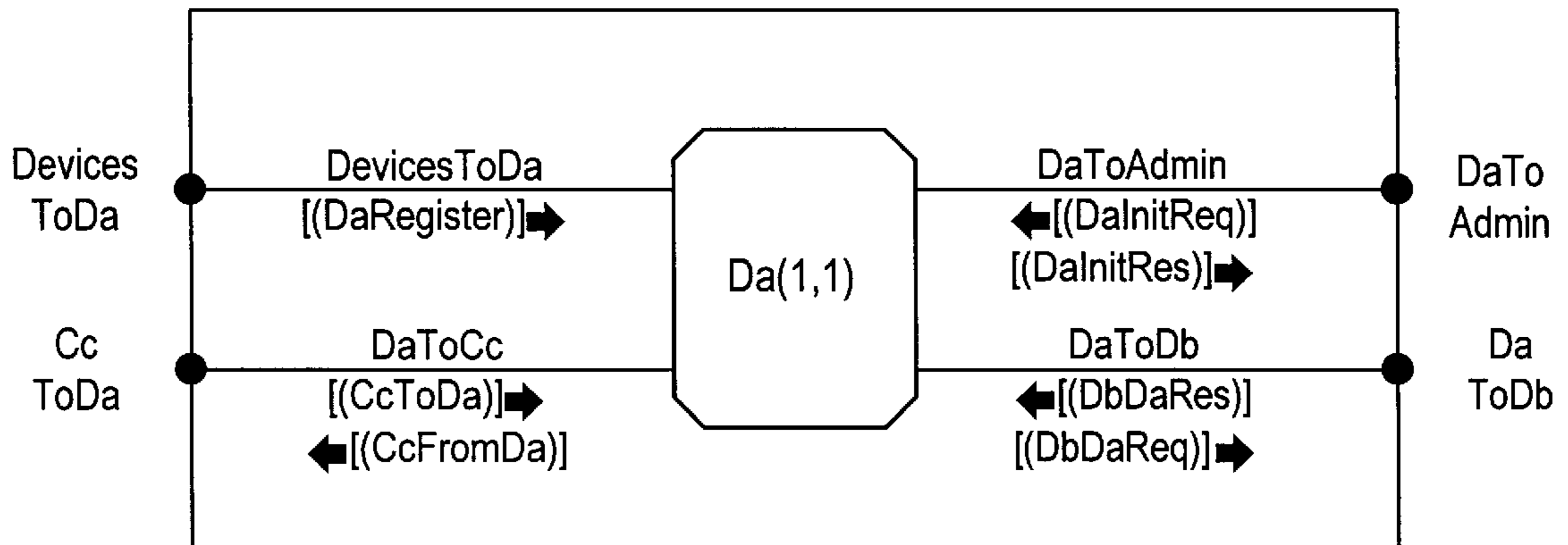
BLOCK MMMan/CPControl/DigitAnalysisTest
