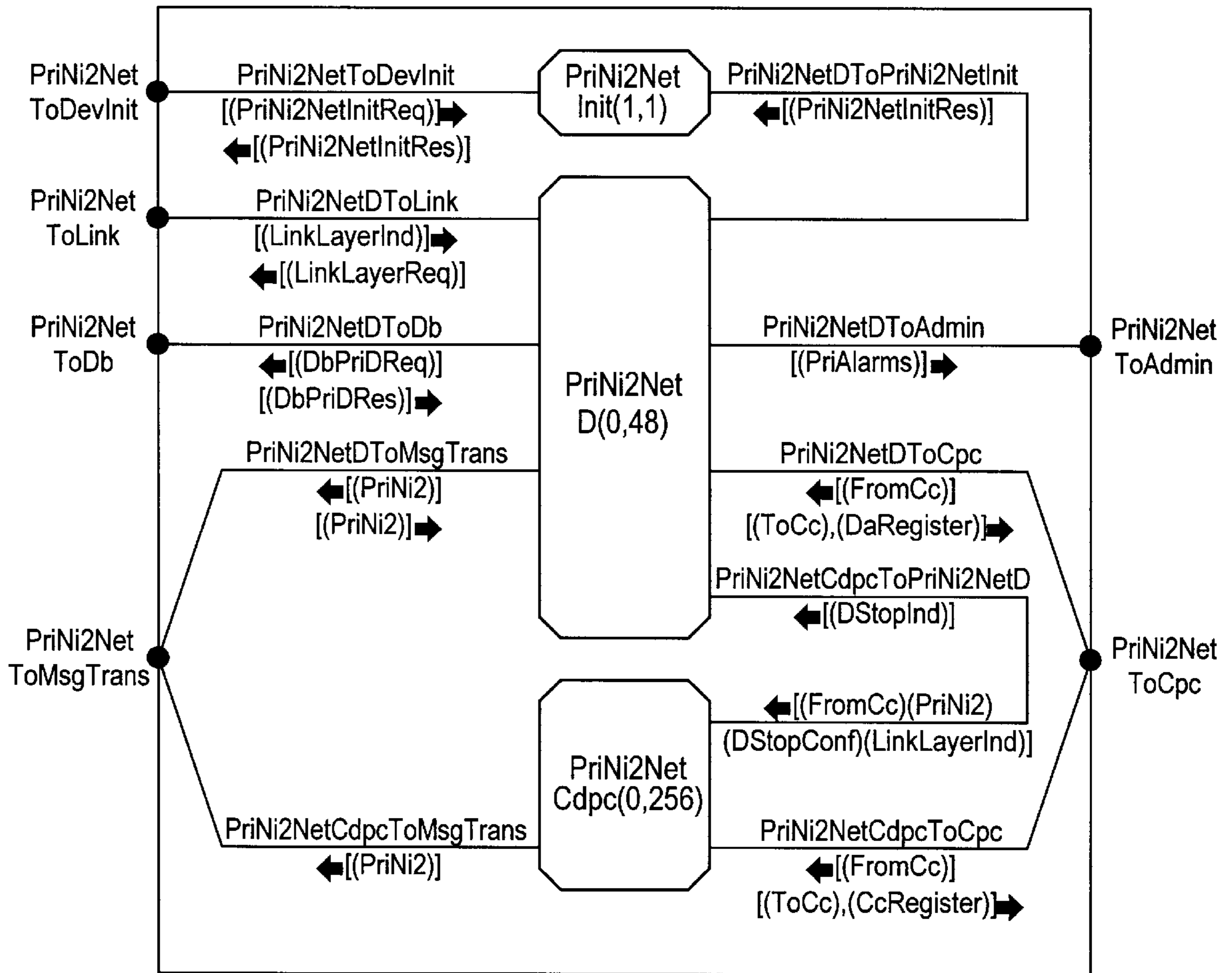
BLOCK MMan/Devices/Devices/Pri/PriNi2/PriNi2Net
