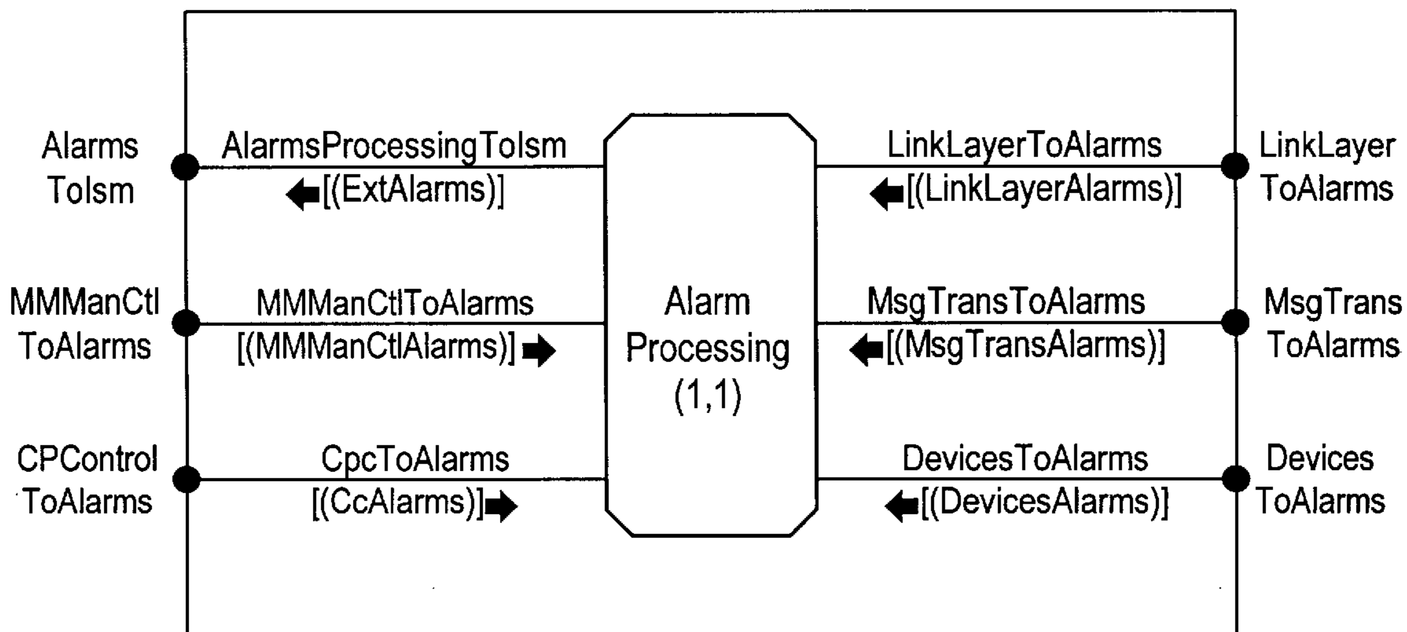
BLOCK MMMan/Admin/Alarms
