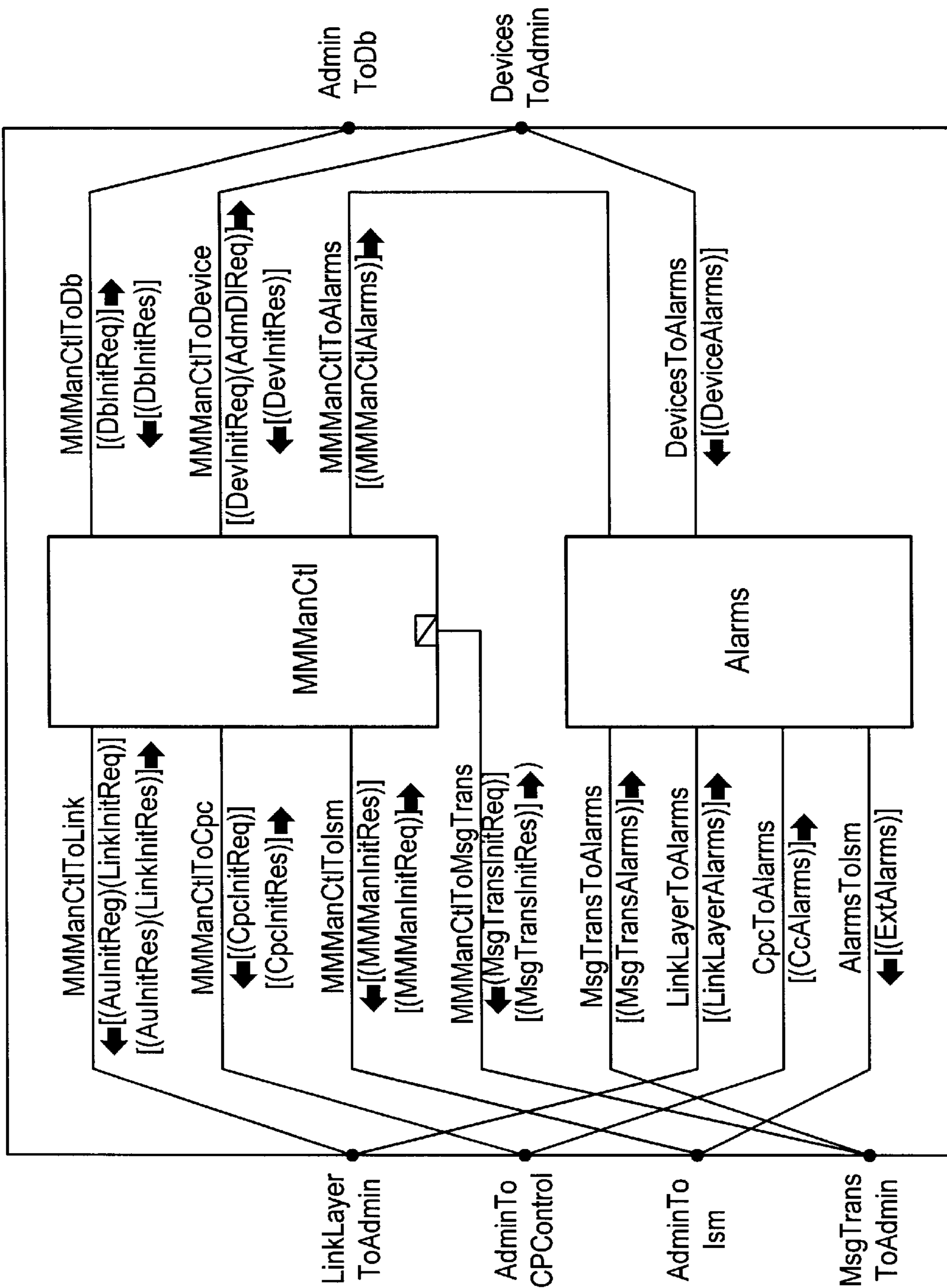
BLOCK MMMan/Admin
