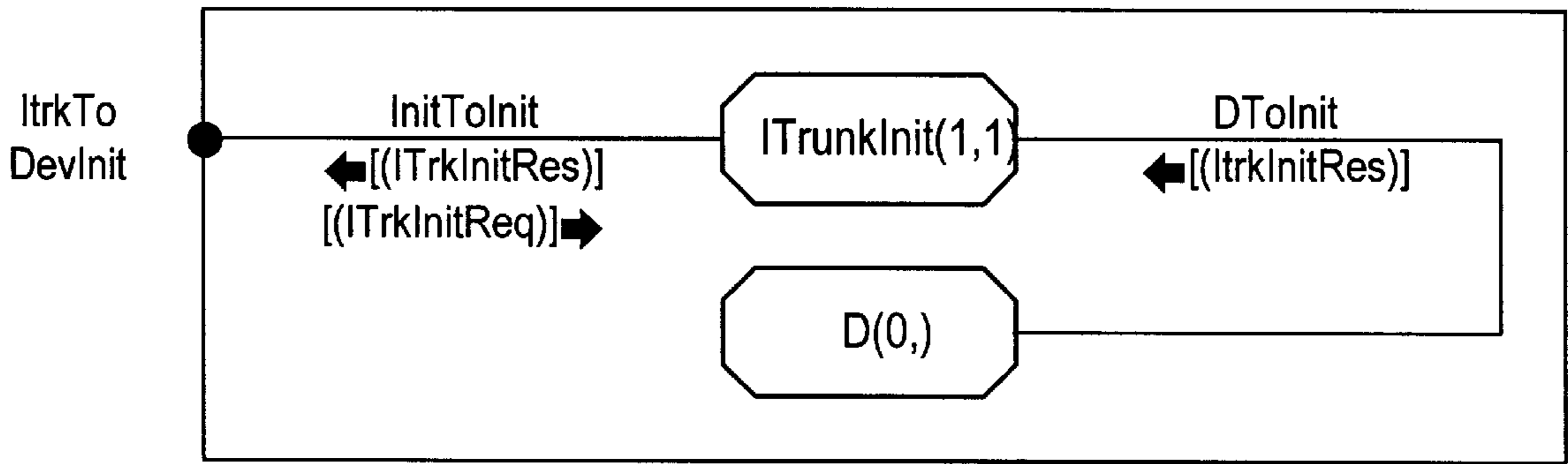
BLOCK MMan/Devices/Devices/ITrunk
