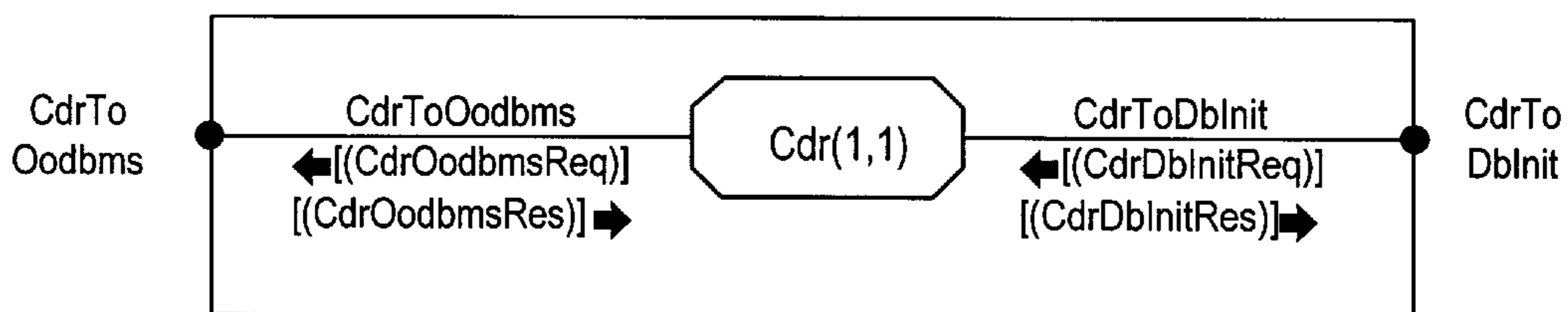
BLOCK MMMan/Db/DbAccess/Cdr
