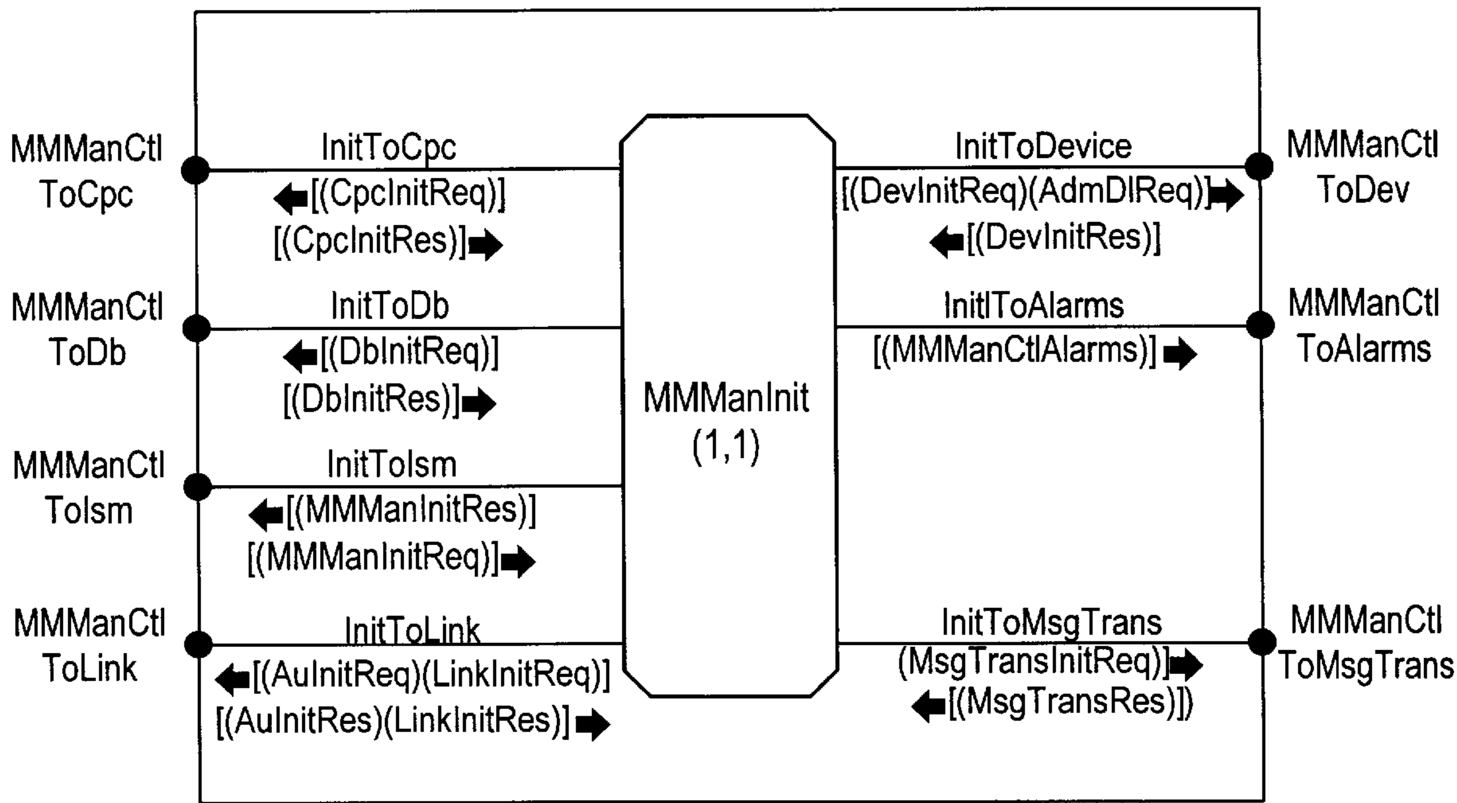
BLOCK MMMan/Admin/MMManCtl
