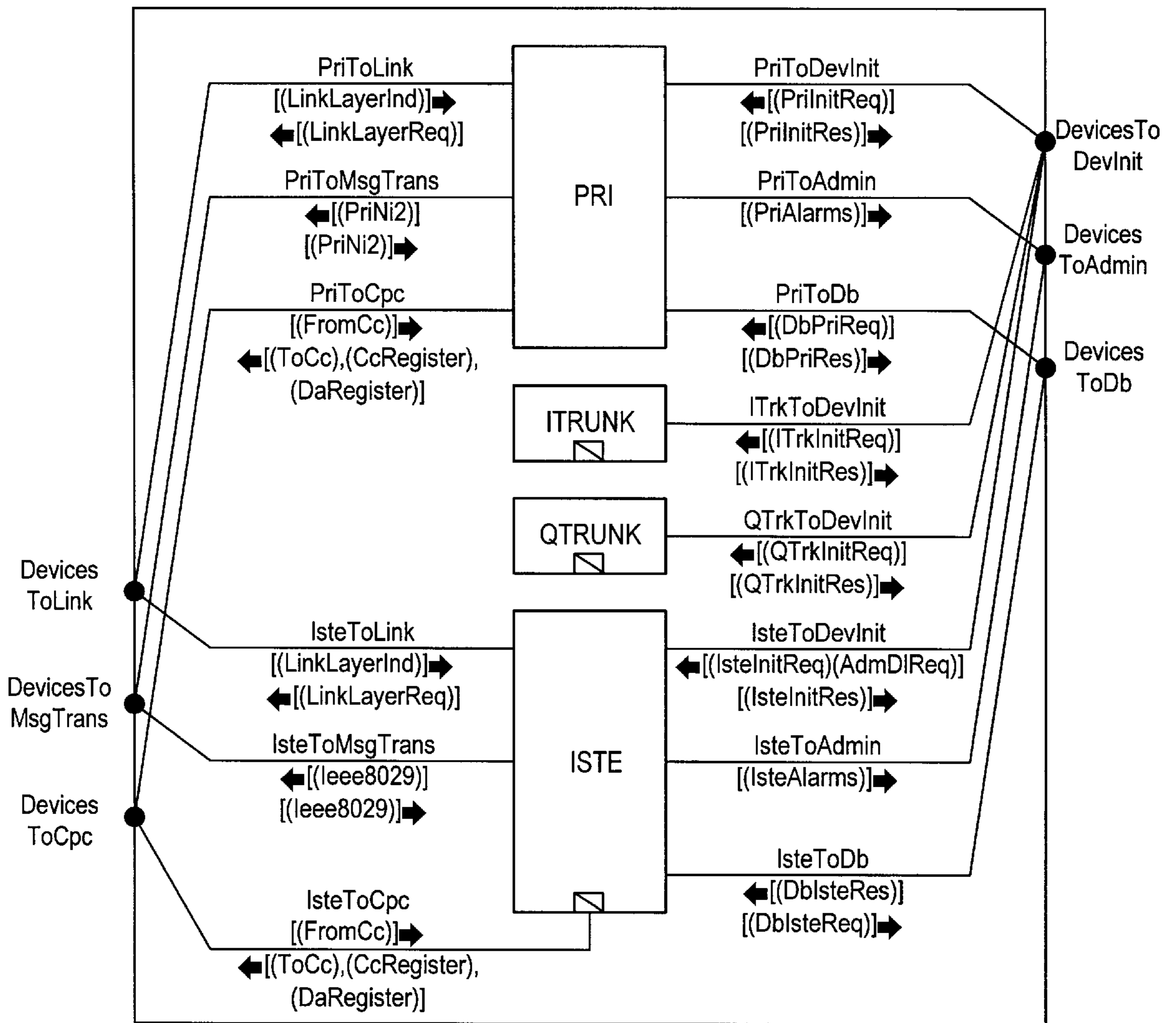
BLOCK MMan/Devices/Devices
