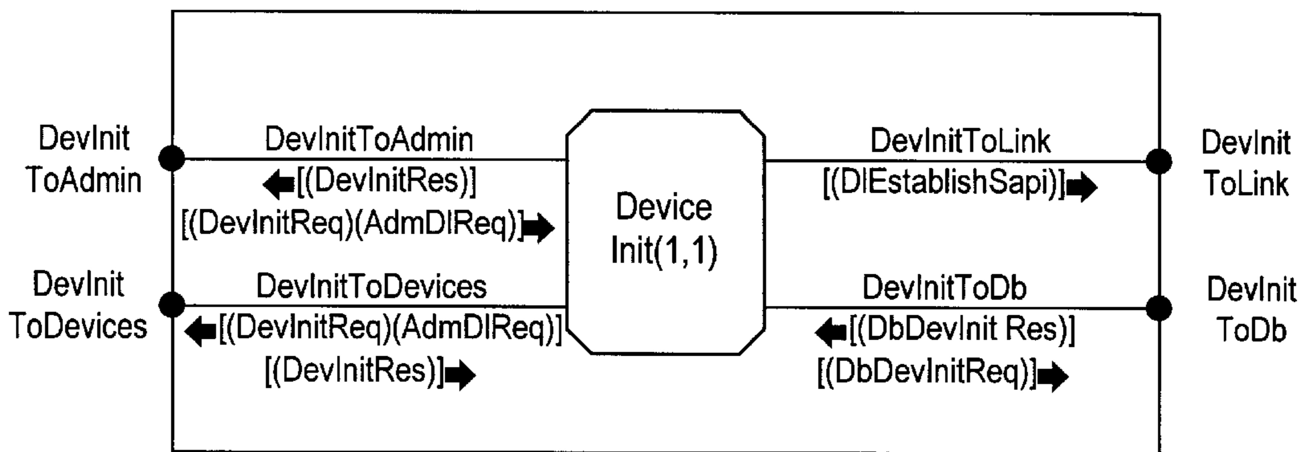
BLOCK MMan/Devices/DeviceInit Figure 2N
