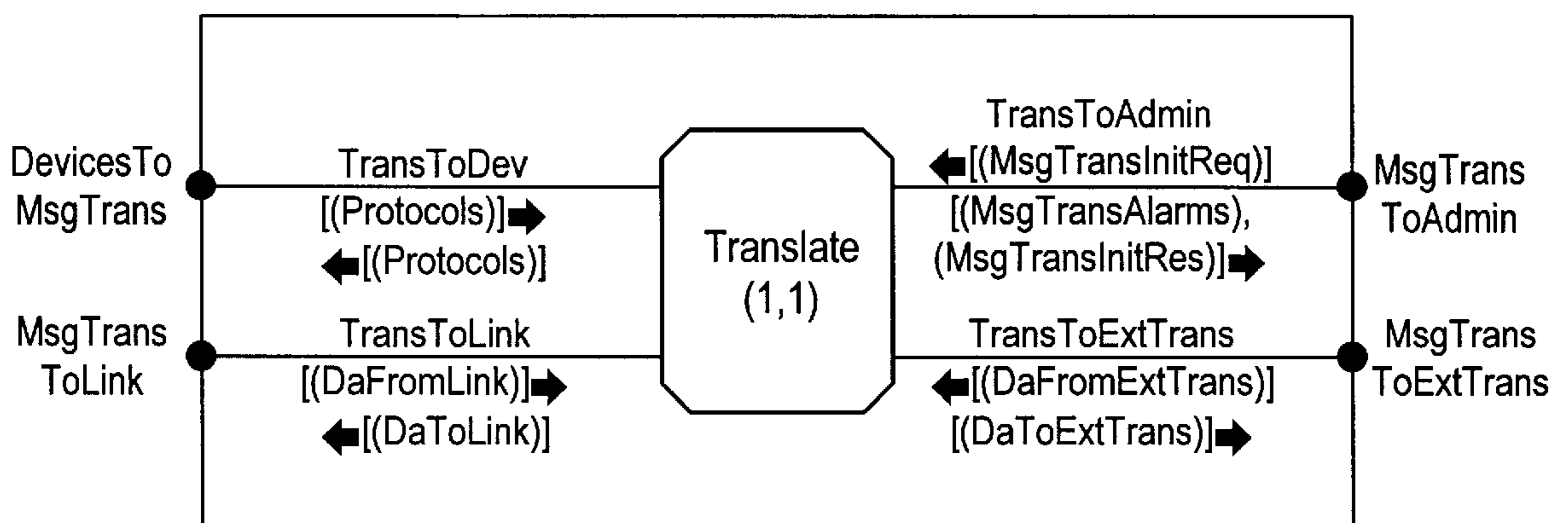
BLOCK MMMan/MsgTrans
