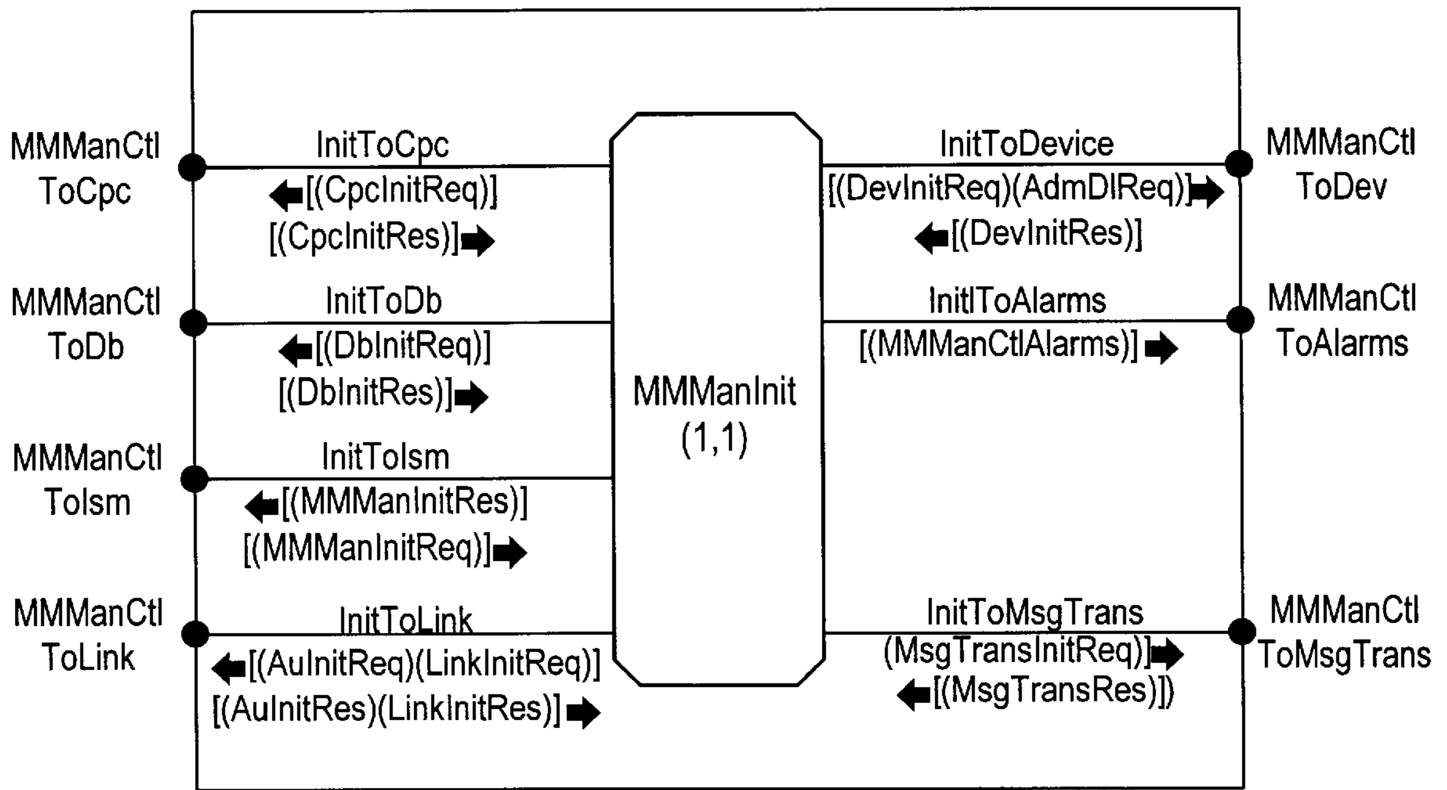
BLOCK MMMan/Admin/MMManCtl
