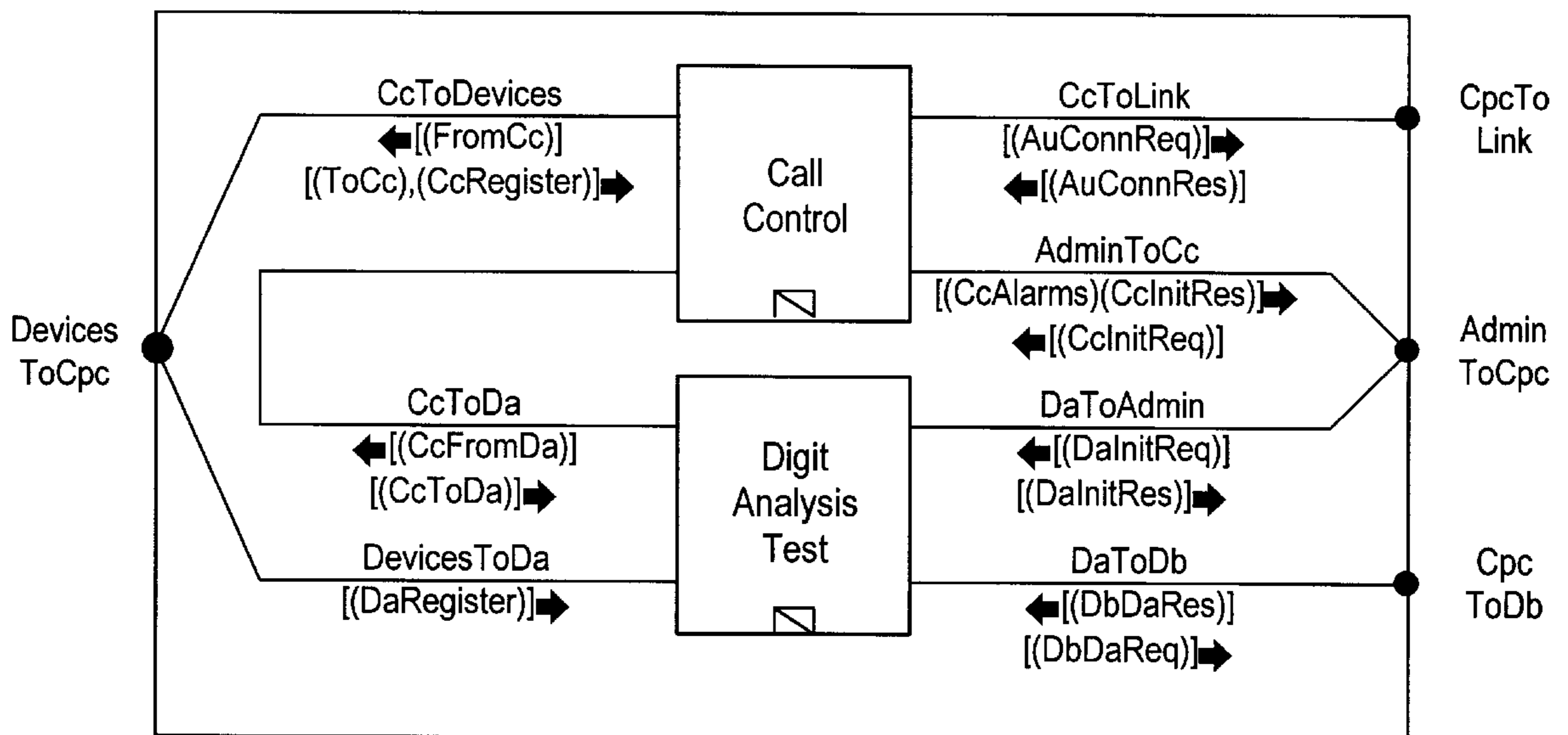
BLOCK MMan/CPControl Figure 2O
