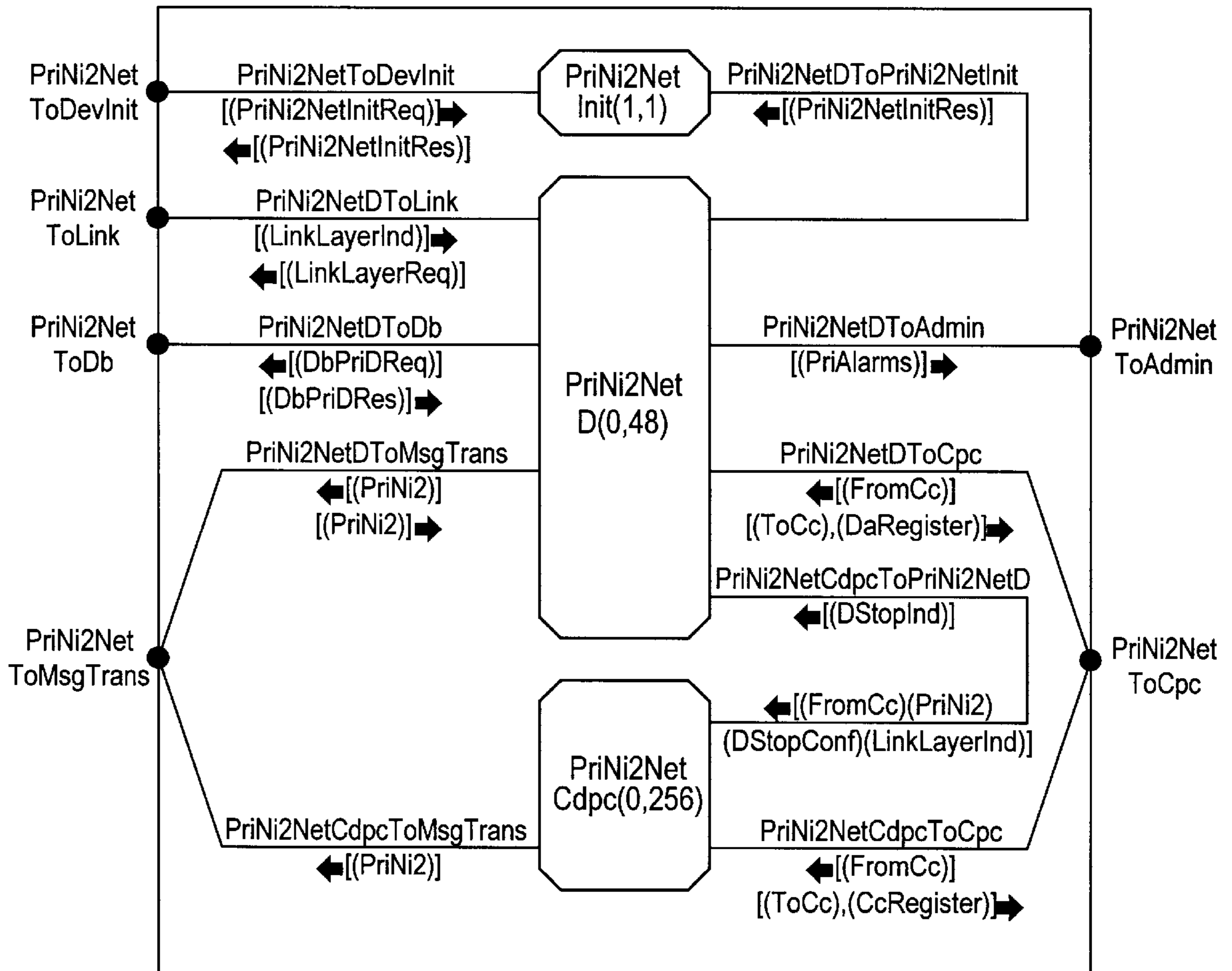
BLOCK MMan/Devices/Devices/Pri/PriNi2/PriNi2Net
