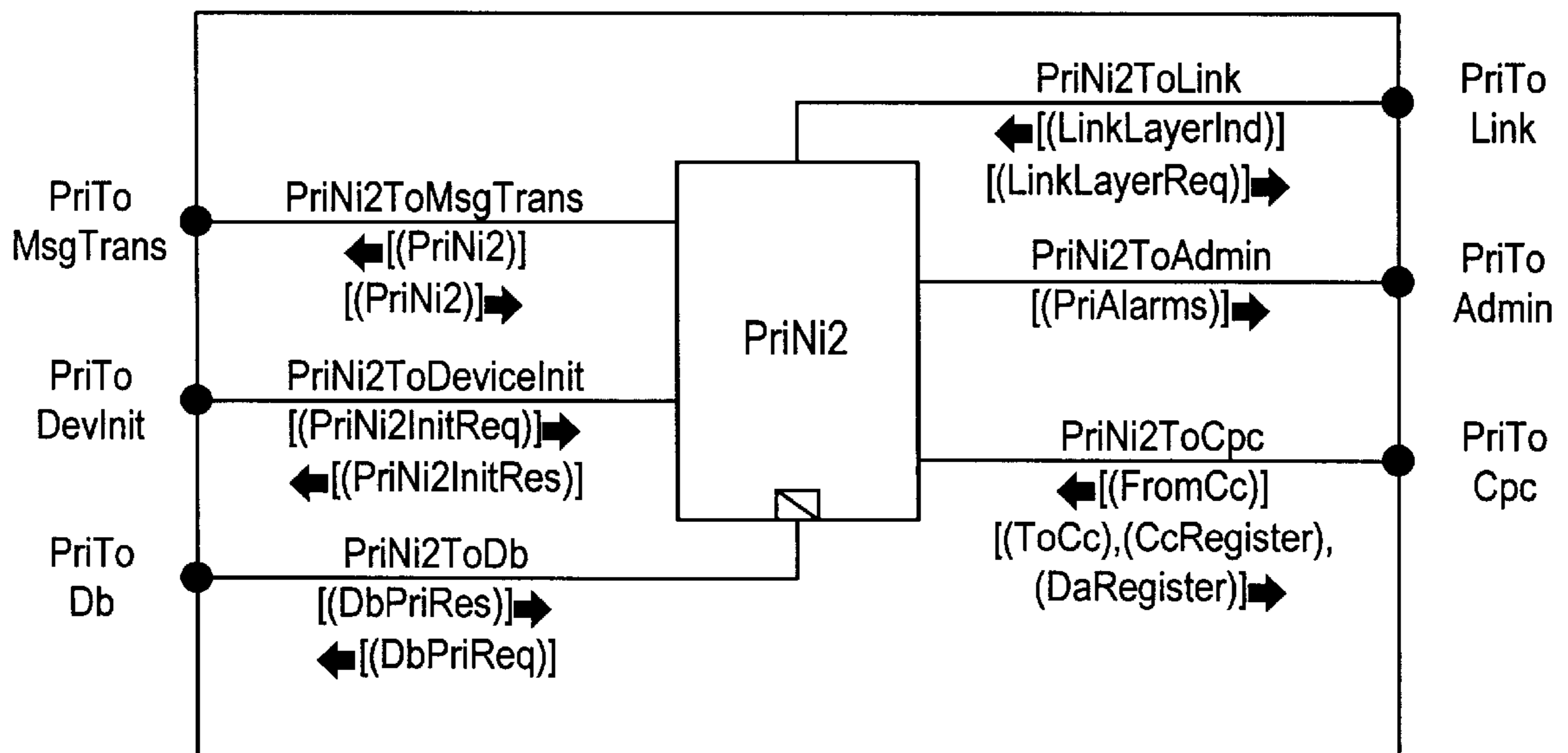
BLOCK MMan/Devices/Devices/Pri
