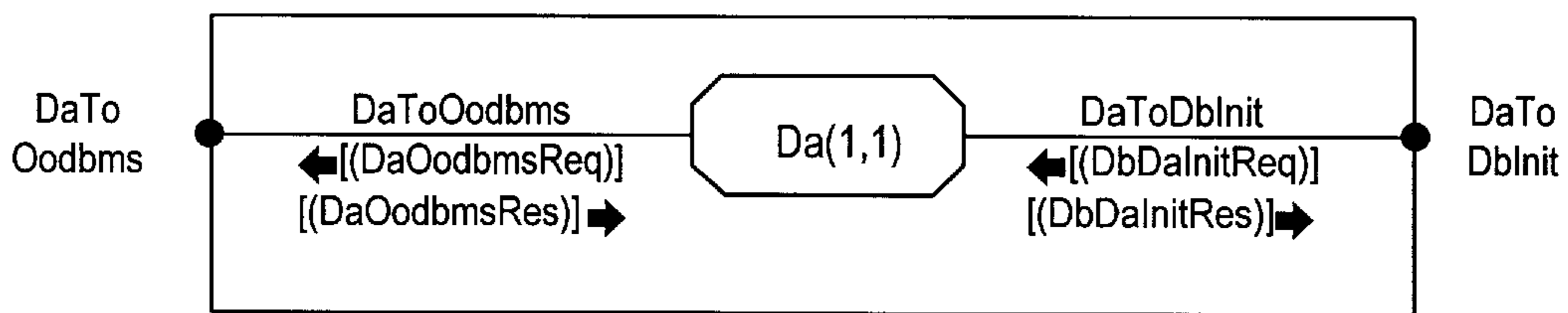
BLOCK MMMan/Db/DbAccess/DigitAnalysis
