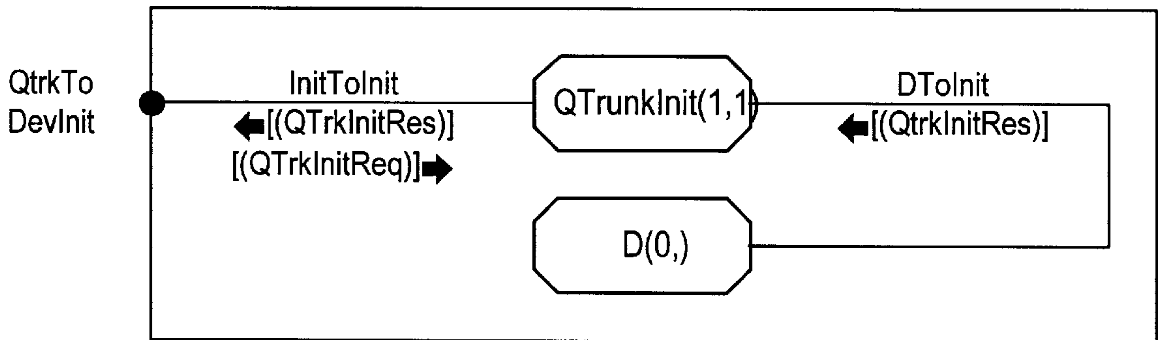
BLOCK MMan/Devices/Devices/QTrunk
