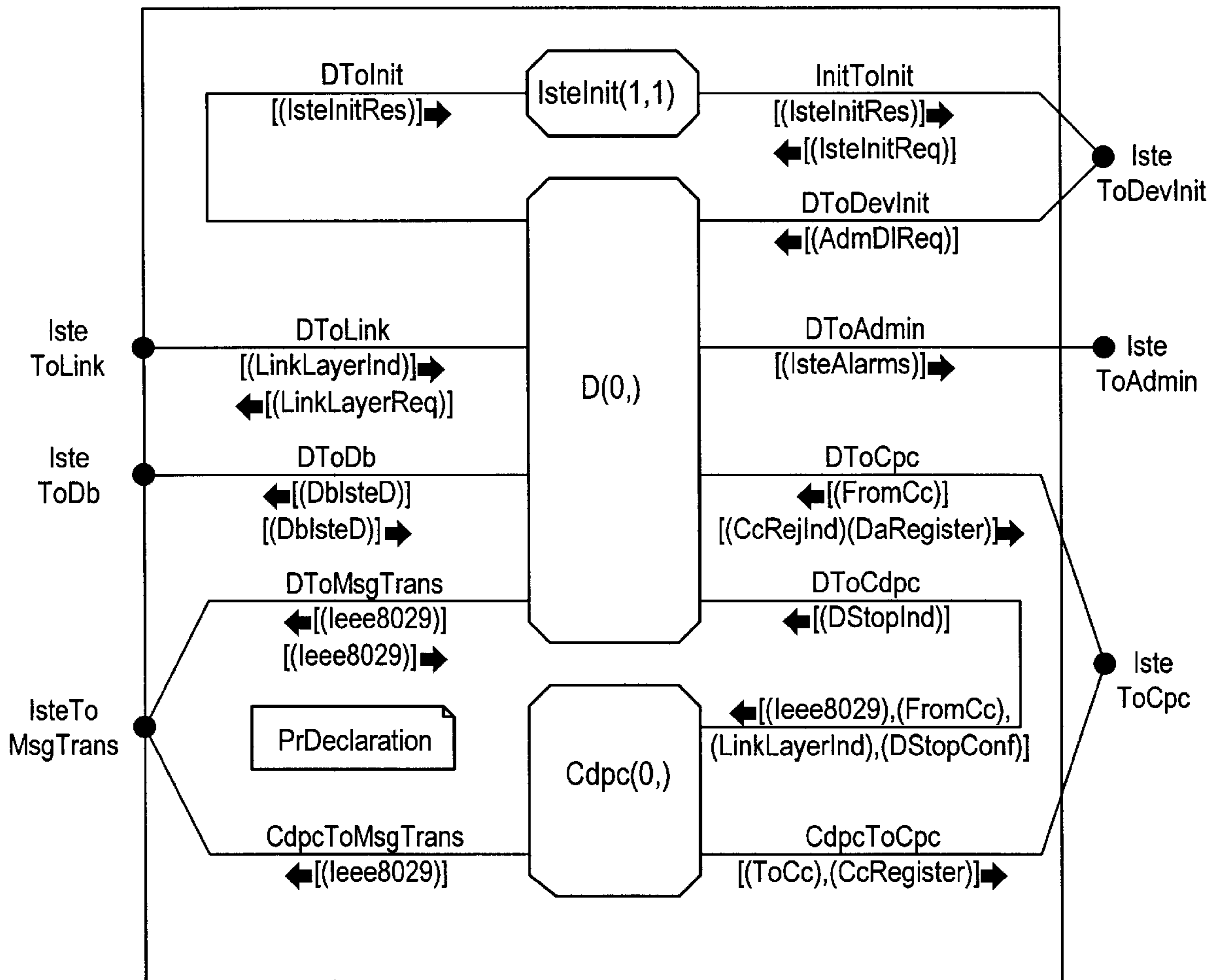
BLOCK MMan/Devices/Devices/ISTE
