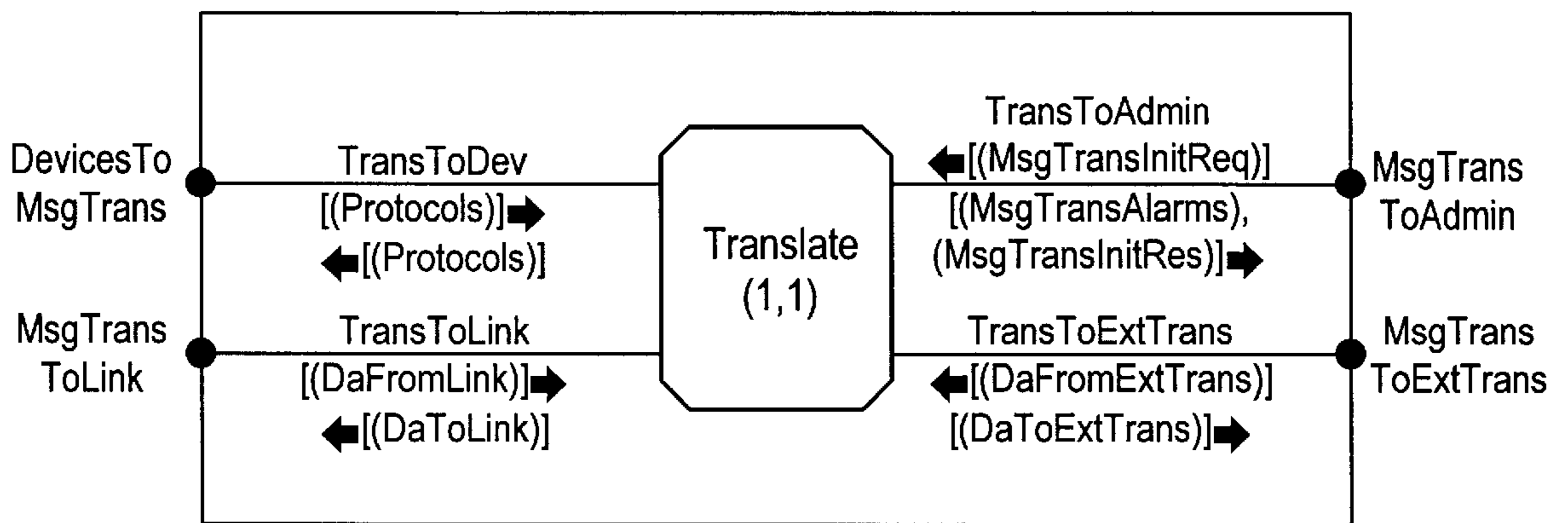
BLOCK MMMan/MsgTrans
