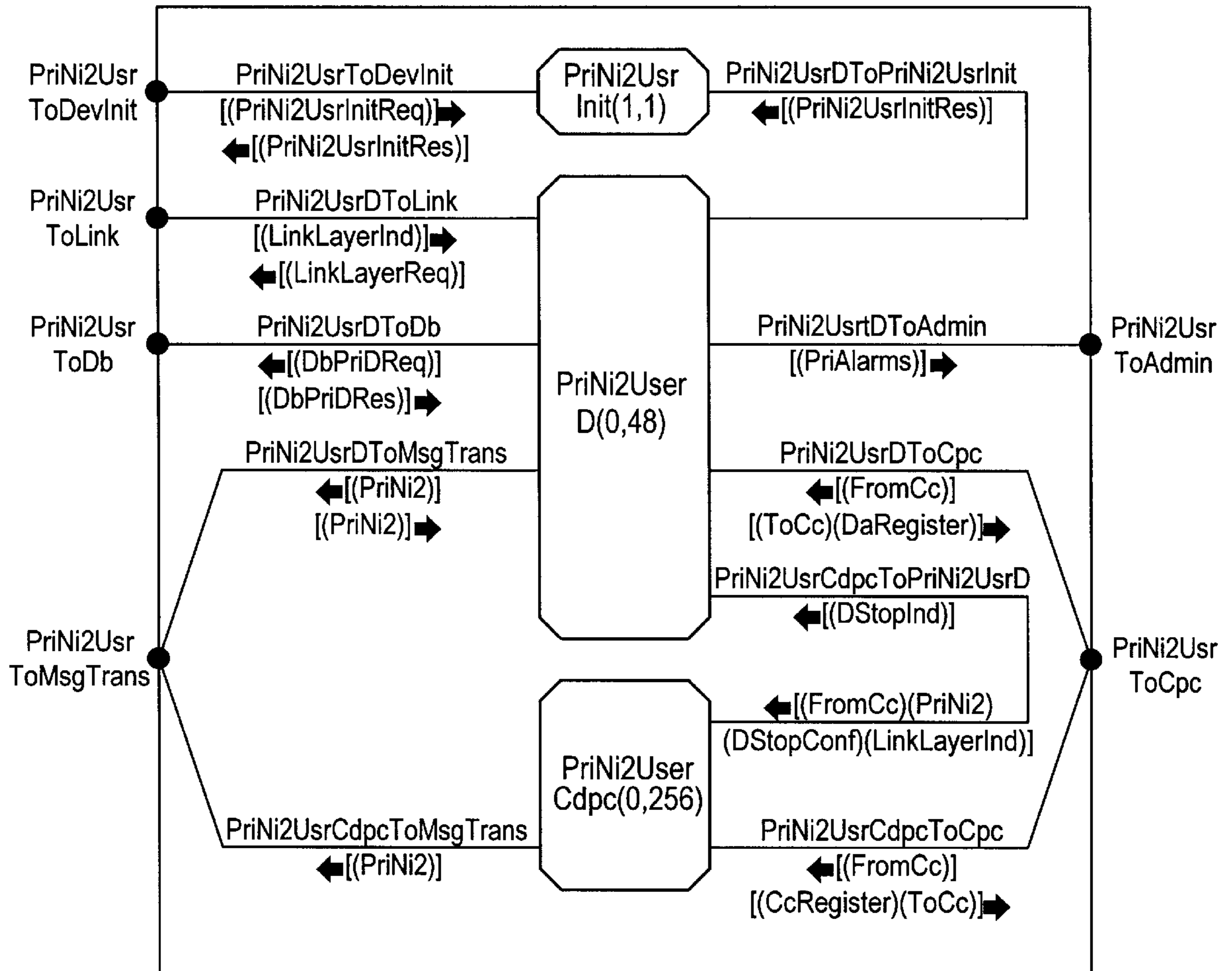
BLOCK MMan/Devices/Devices/Pri/PriNi2/PriNi2User
