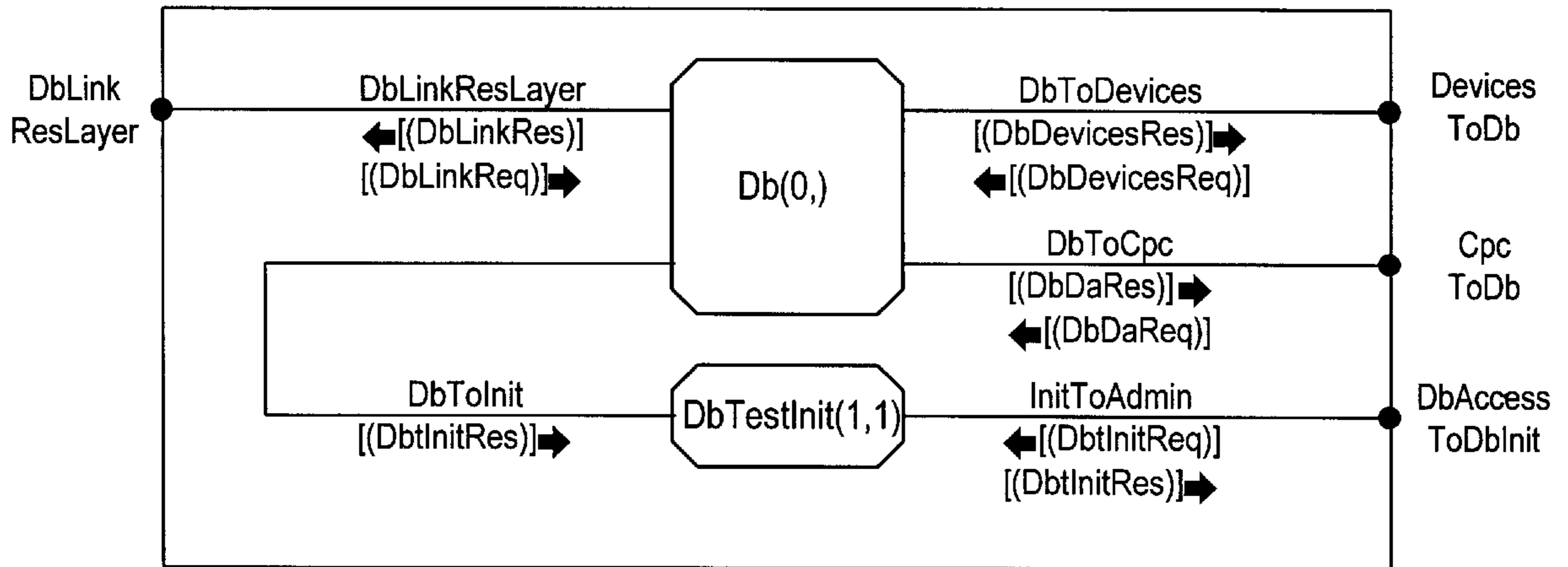
BLOCK MMMan/Db/DbAccess/DbTest
