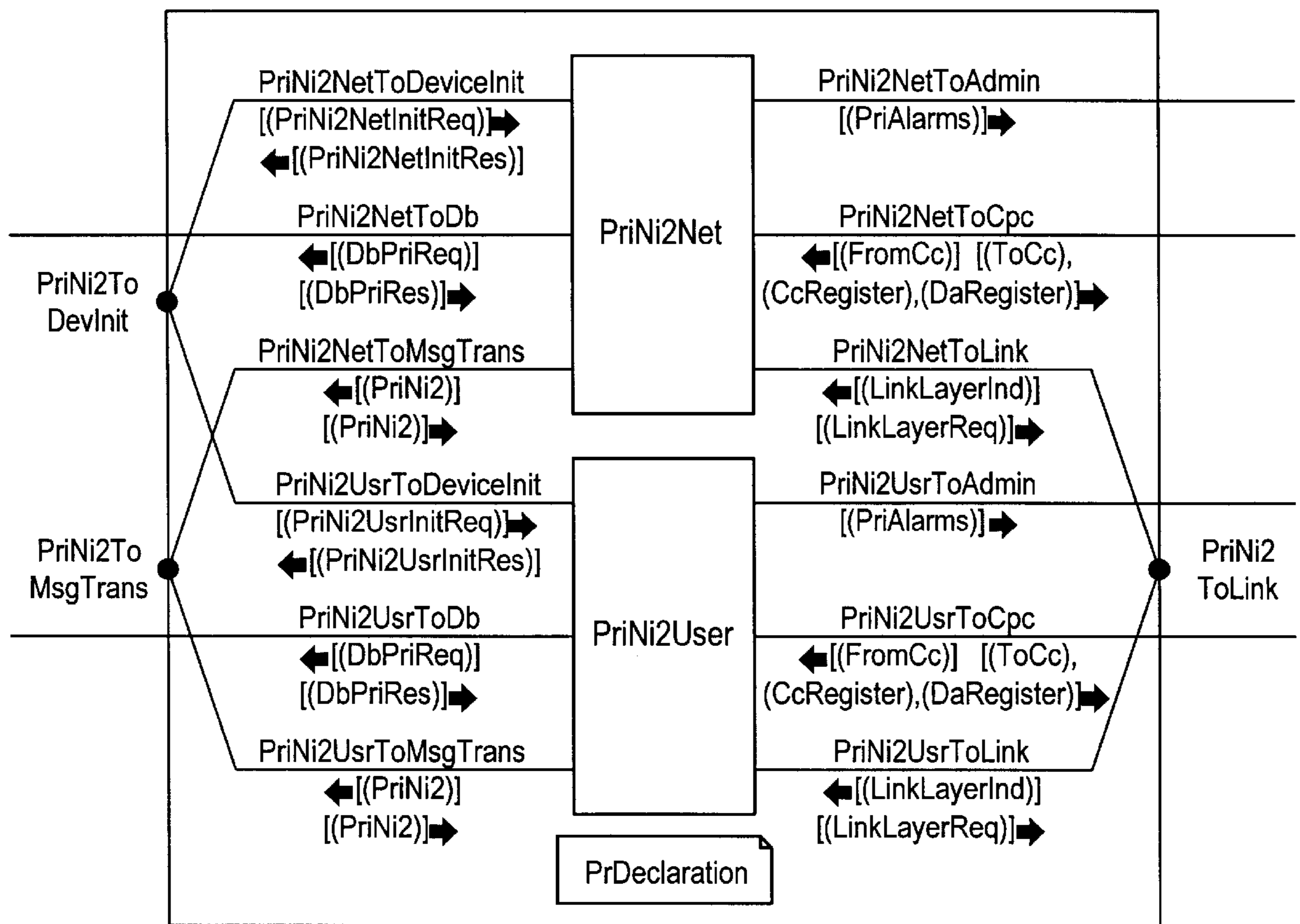
BLOCK MMan/Devices/Devices/Pri/PriNi2
