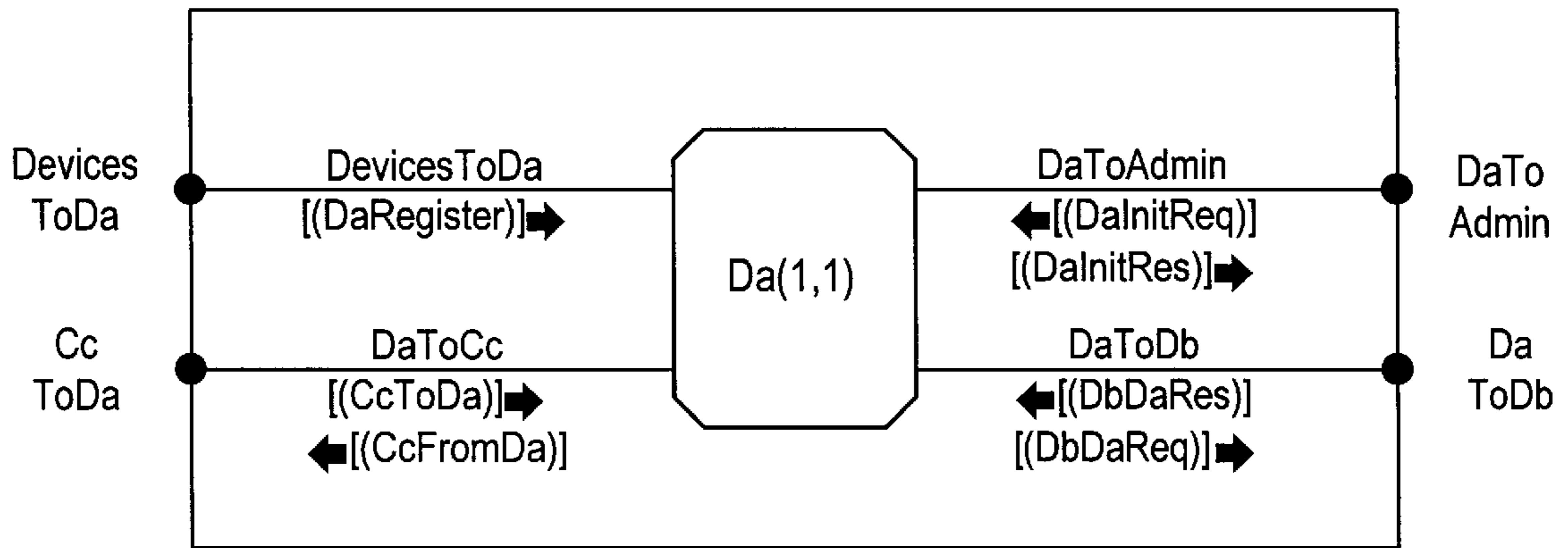
BLOCK MMMan/CPControl/DigitAnalysisTest
