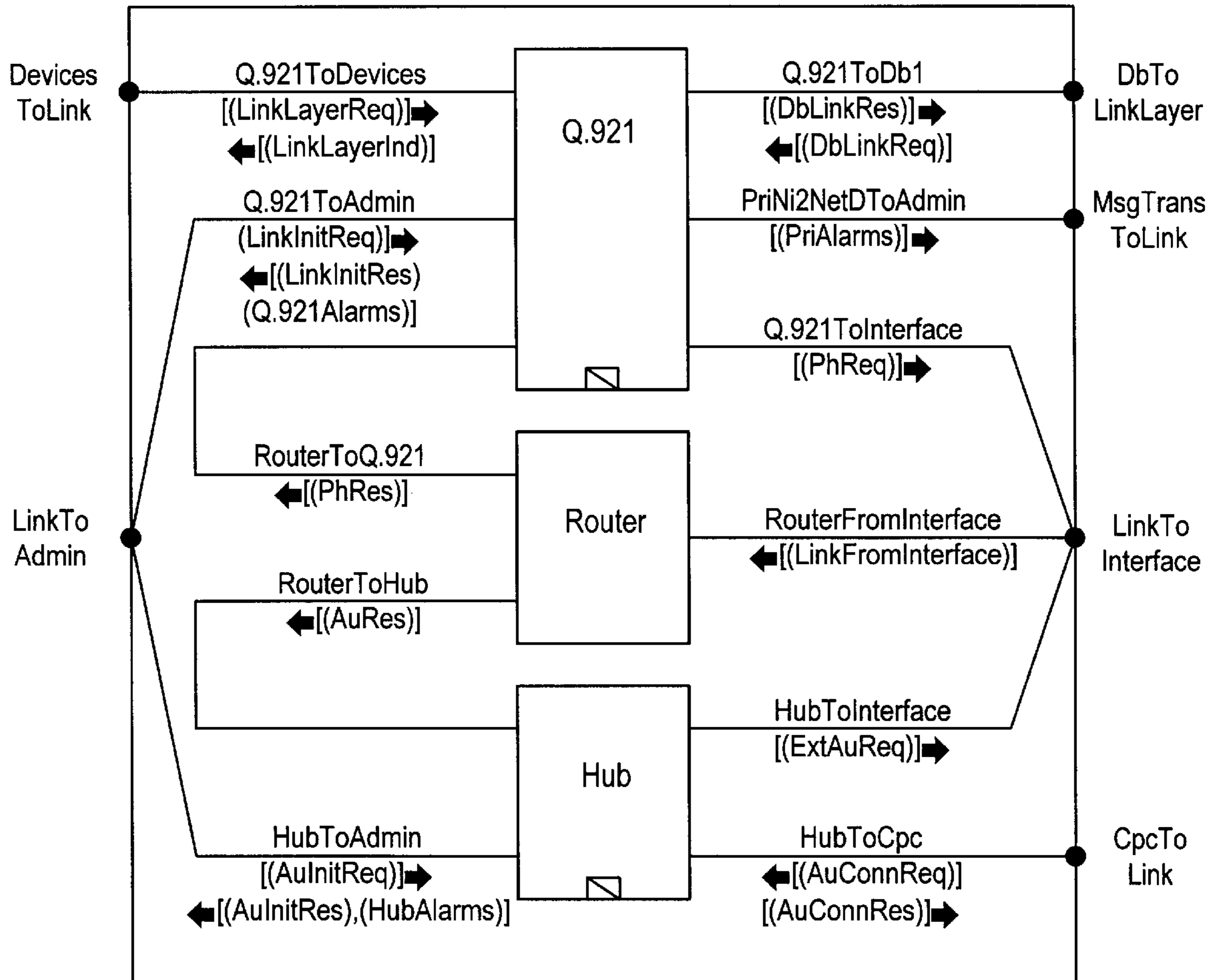
BLOCK MMan/LinkLayer
