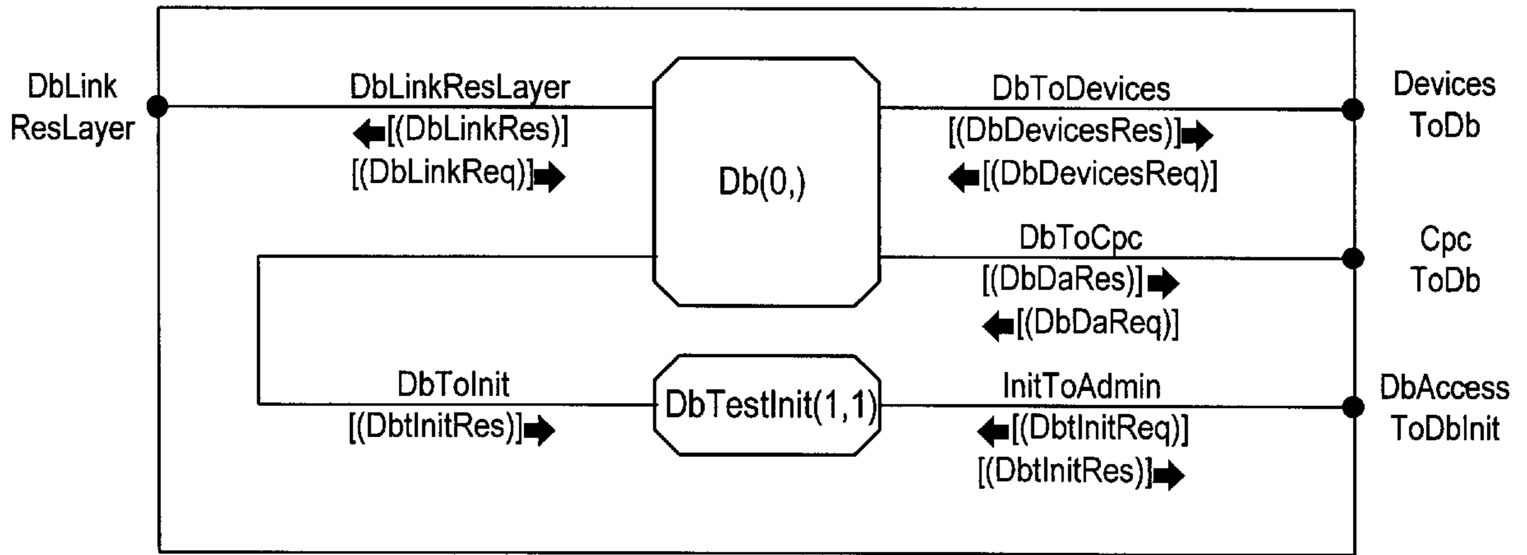
BLOCK MMMan/Db/DbAccess/DbTest
