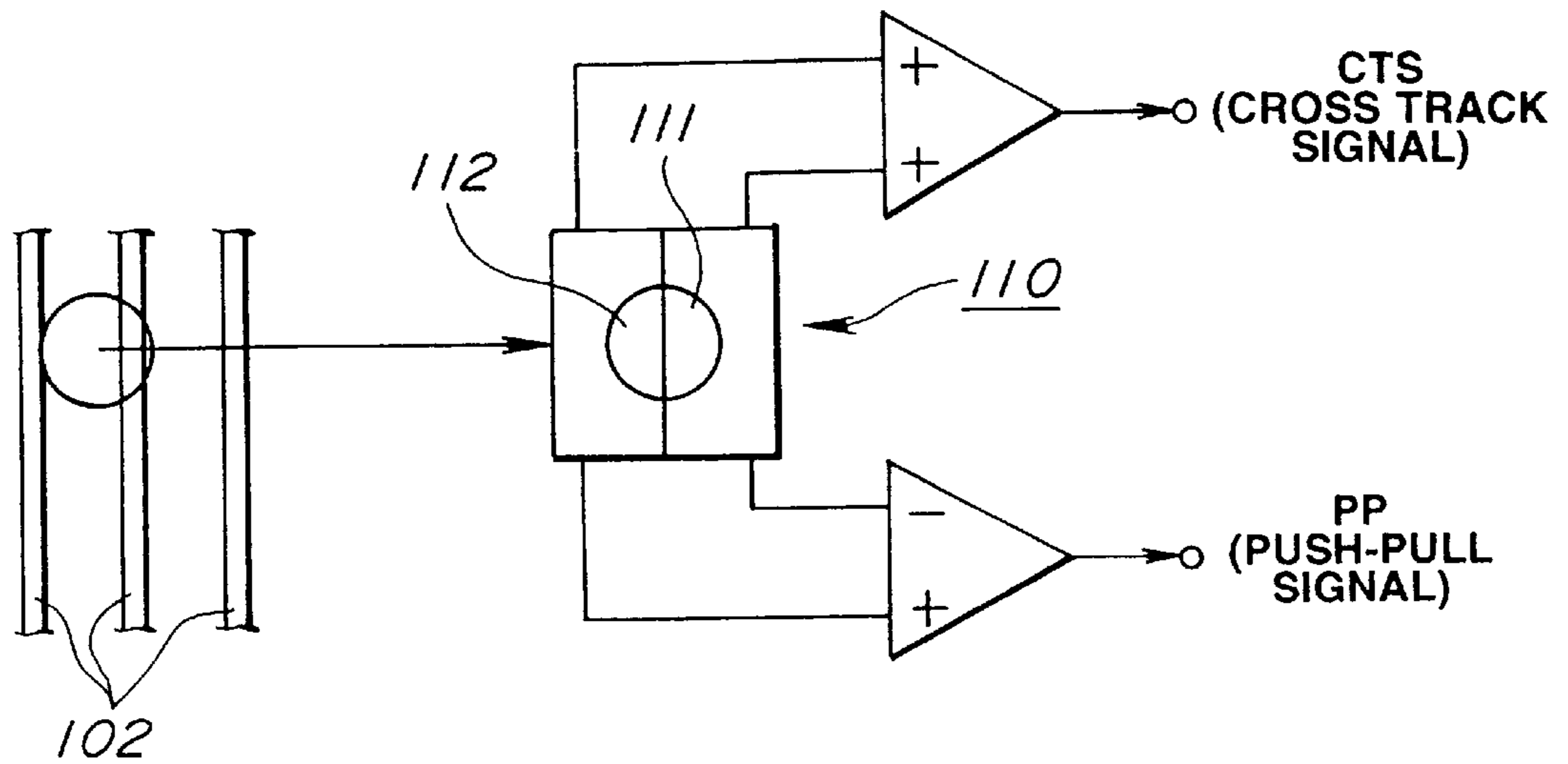
FIG.4 ( PRIOR ART )
