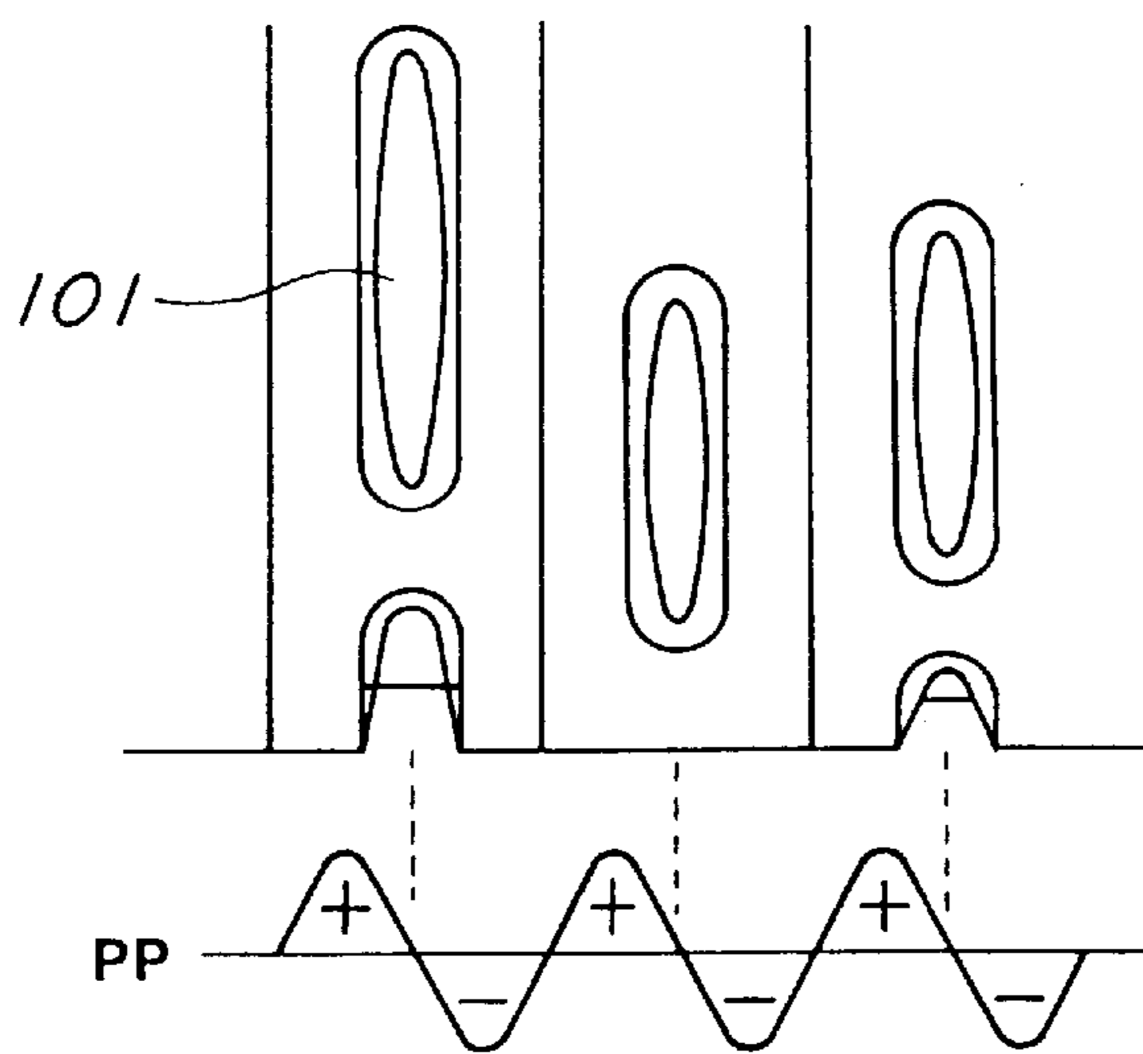
FIG.6 ( PRIOR ART )
