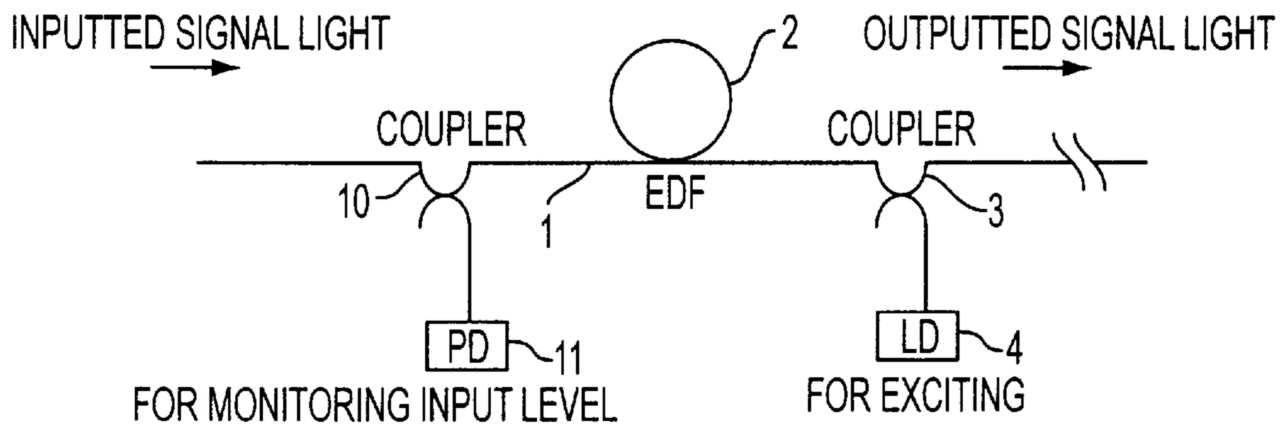
FIG. 15 PRIOR ART
