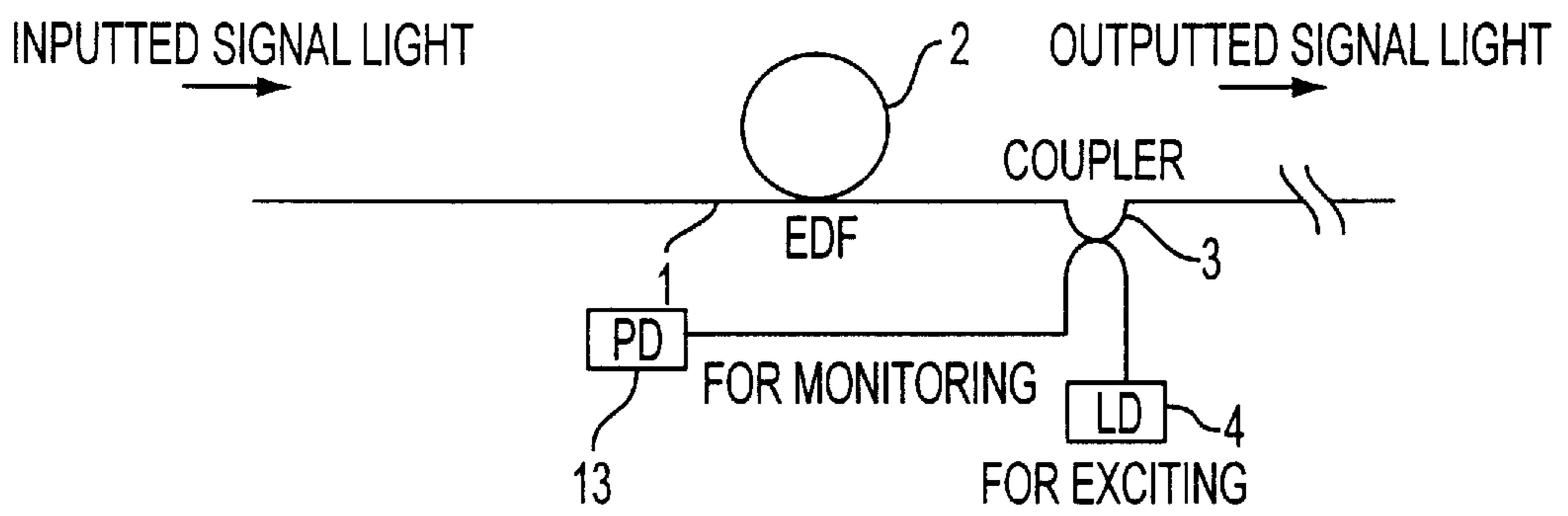
FIG. 16 PRIOR ART
