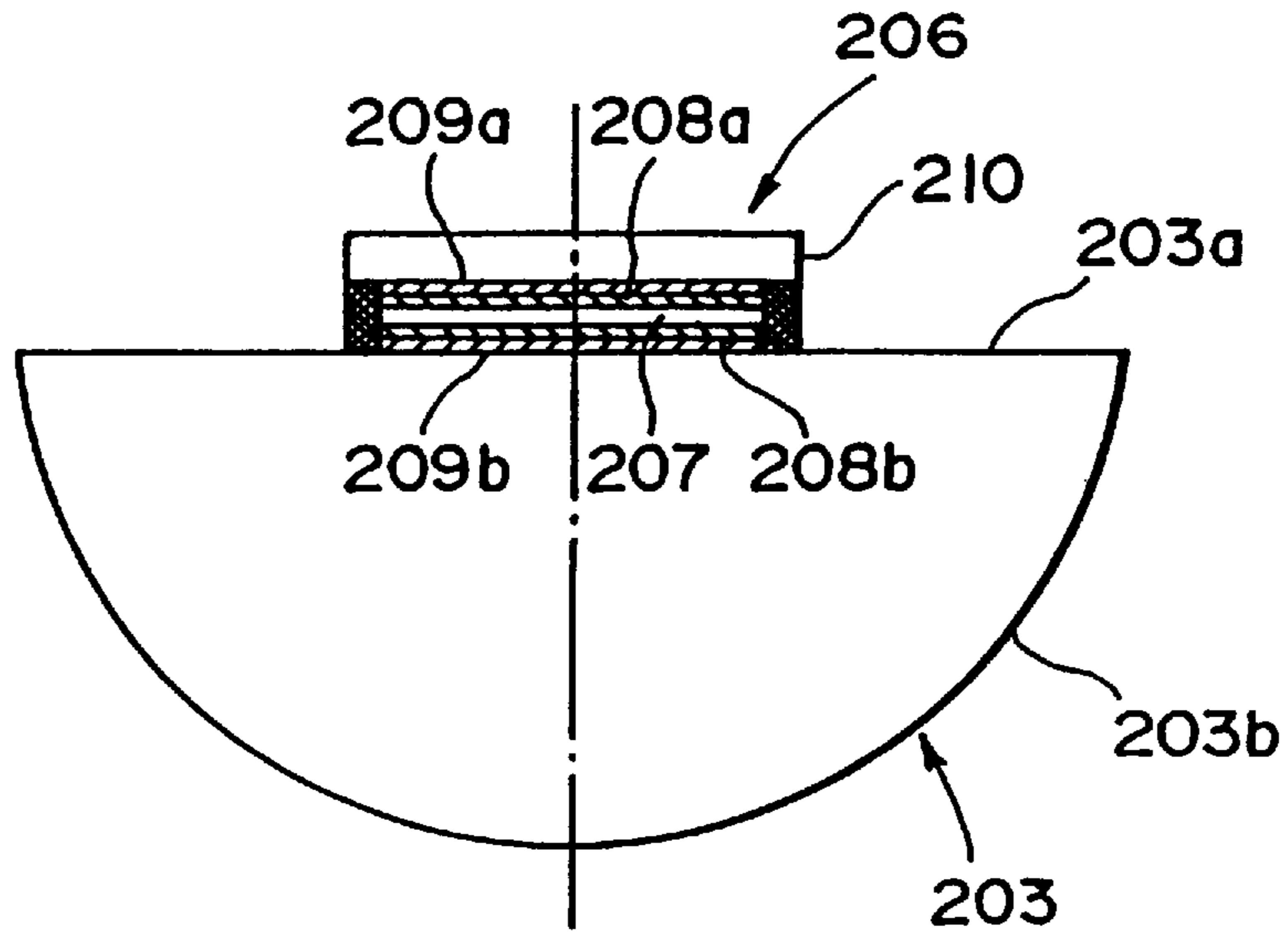
FIG. 13 PRIOR ART
