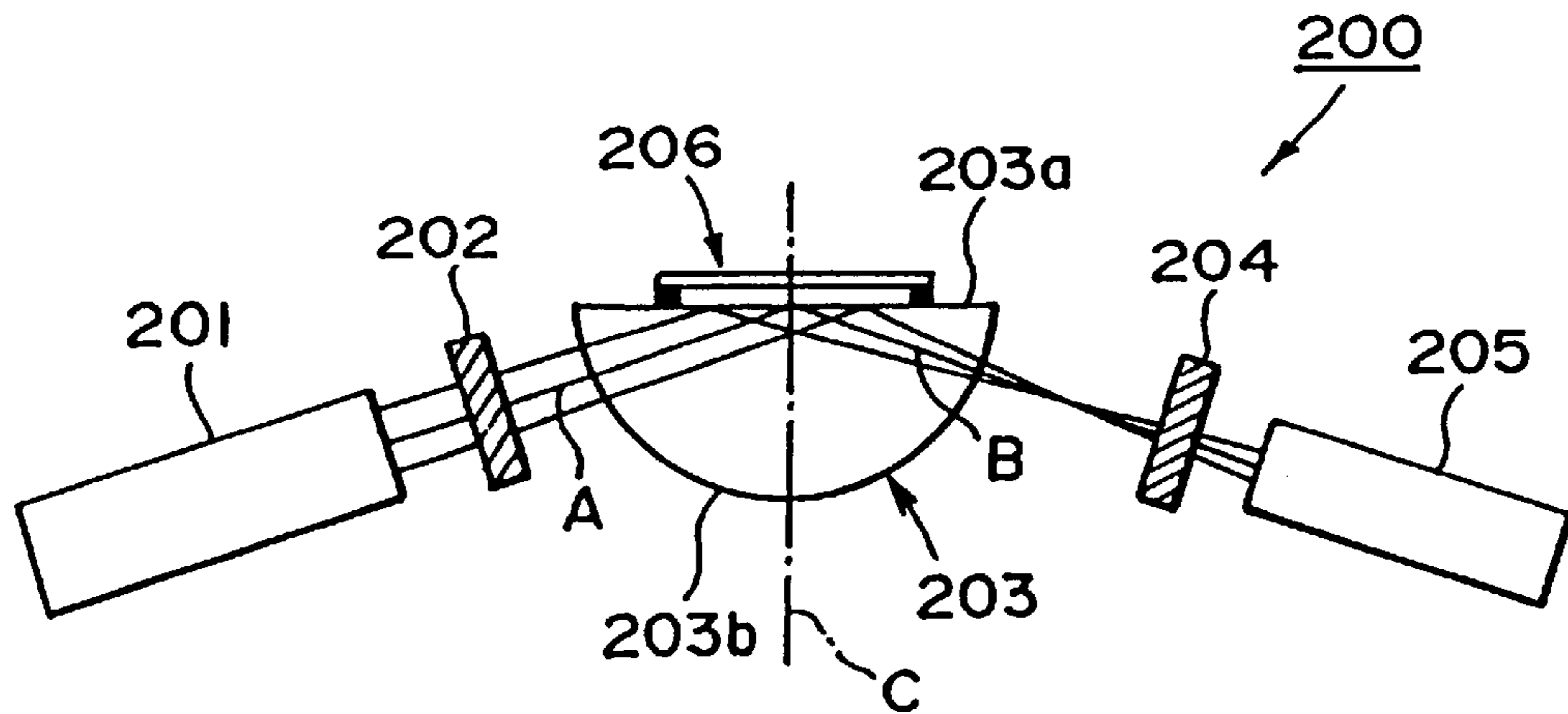
FIG. 12 PRIOR ART
