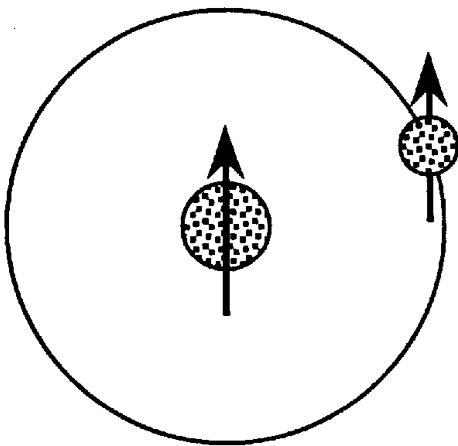
|++\rangle FIG. 10(a)
