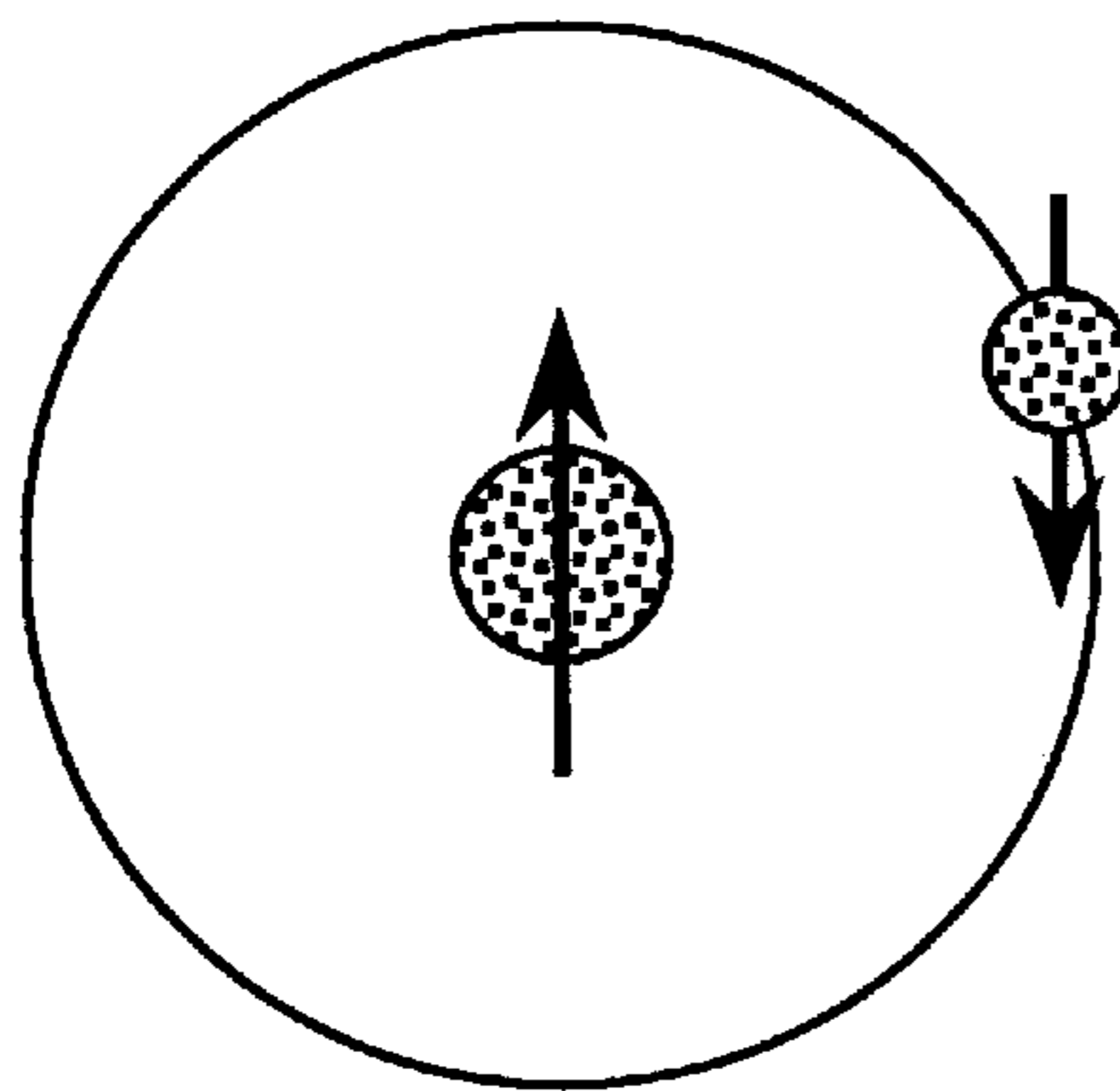
| - +\rangle FIG. 10(c)
