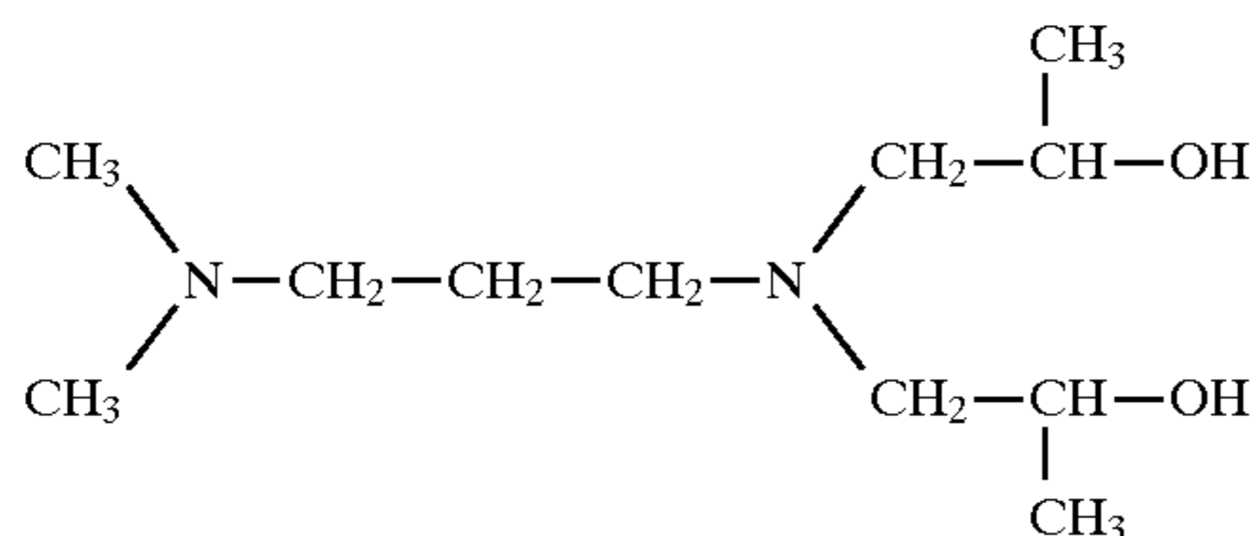
N,N-dimethyl-N',N'-di(2-hydroxypropyl)-1,3-propane diamine
