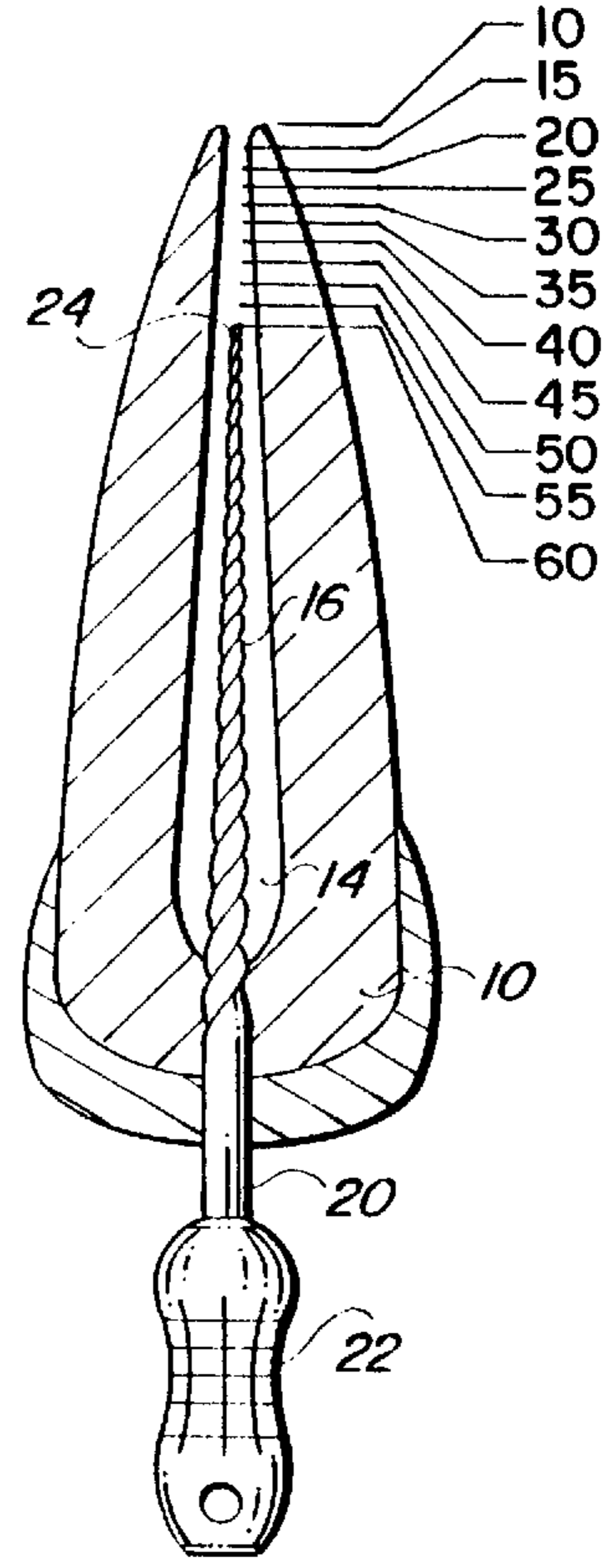
FIG. 2 (PRIOR ART)
