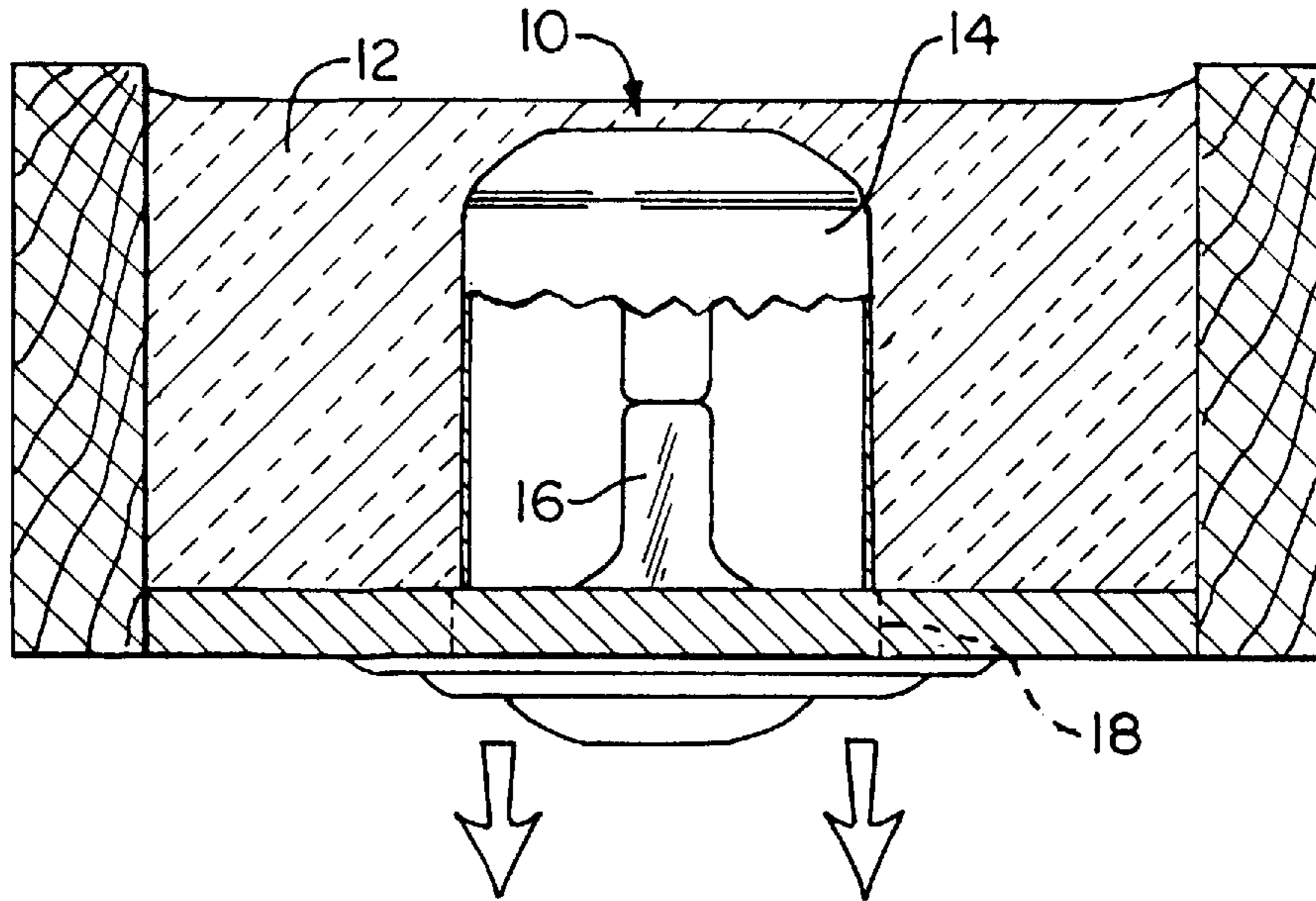
FIG. 1 PRIOR ART
