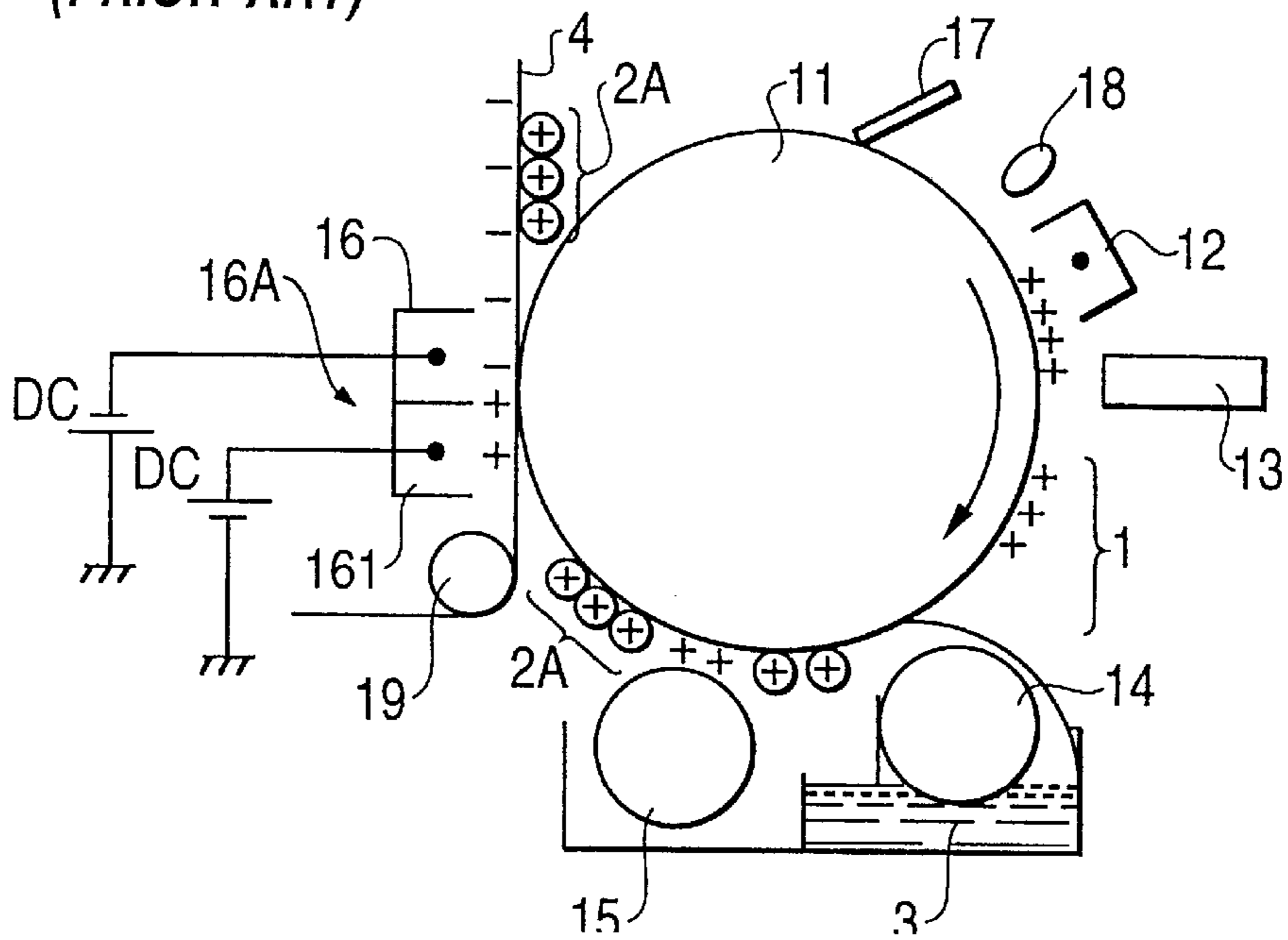
FIG. 13 (PRIOR ART)
