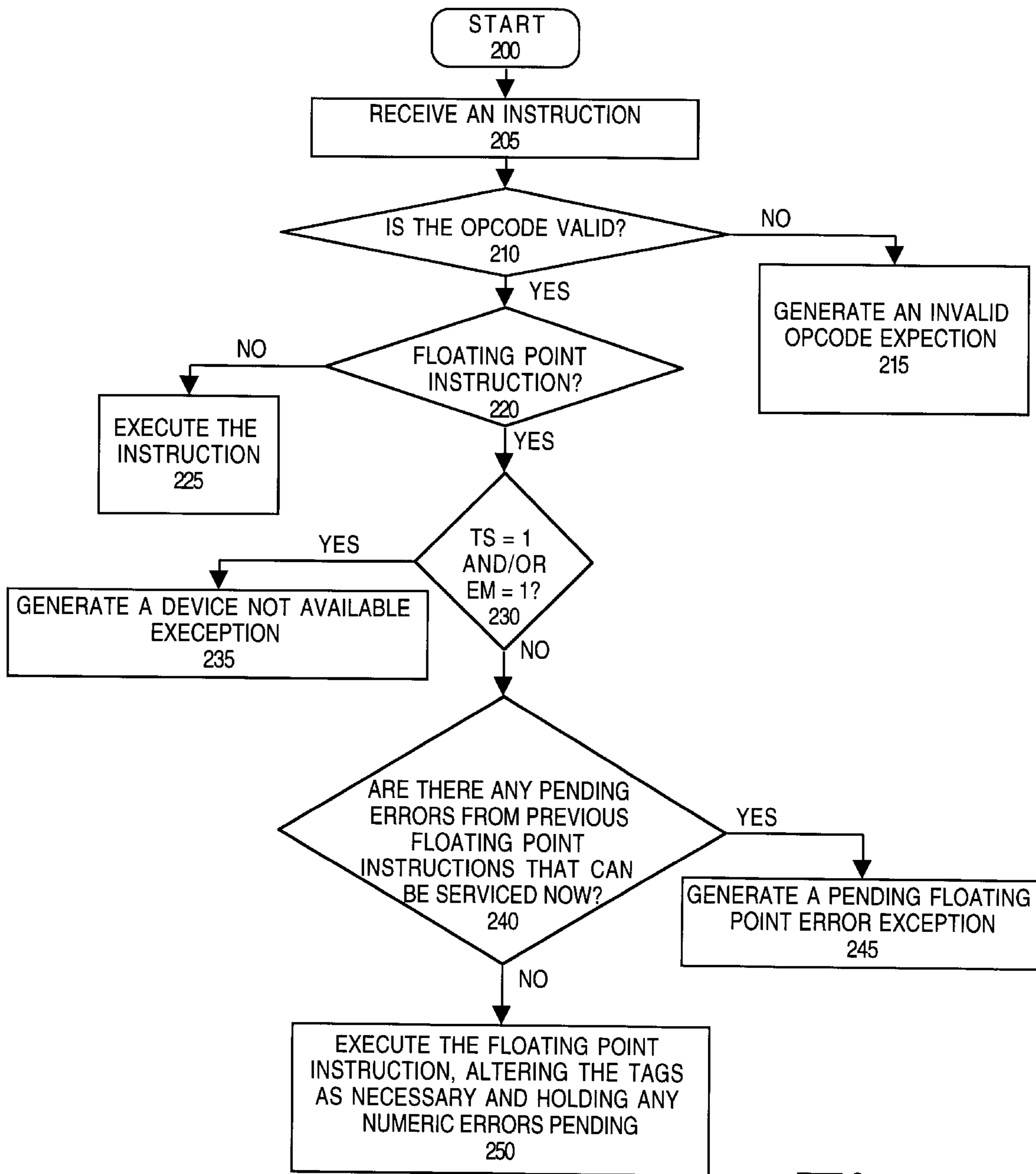
Fig. 2 (Prior Art)
