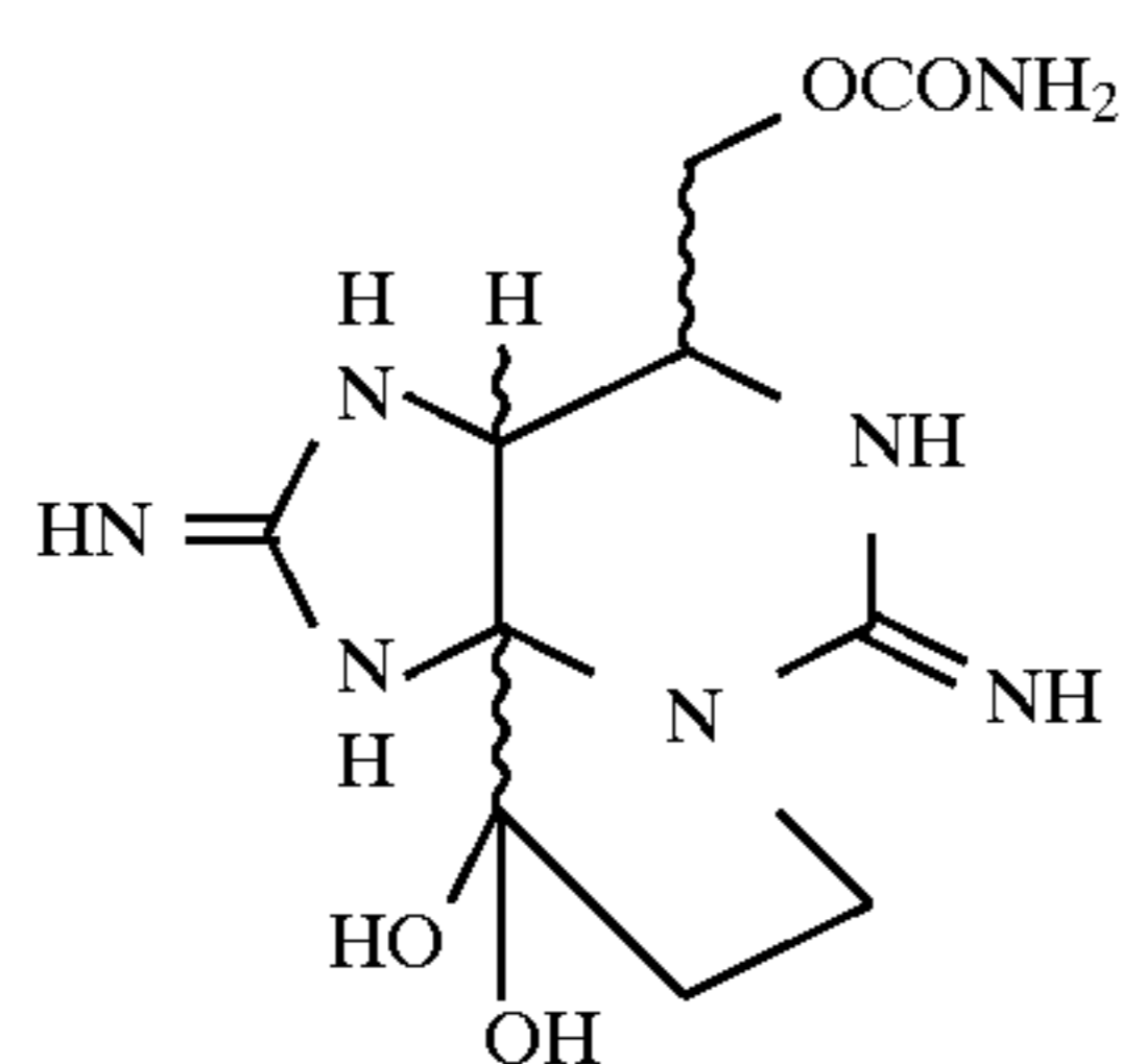
SAXITOXIN
