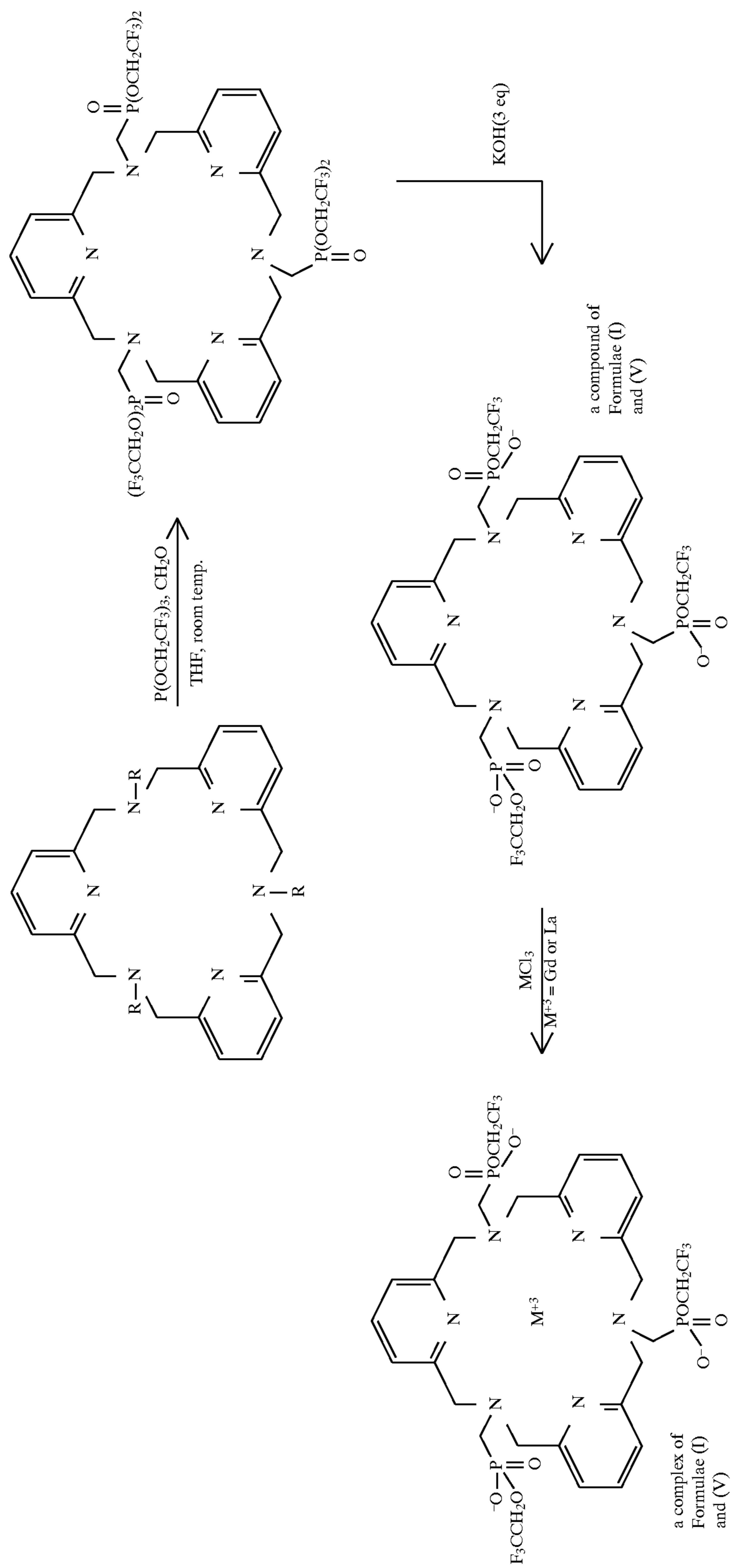
Scheme 4
