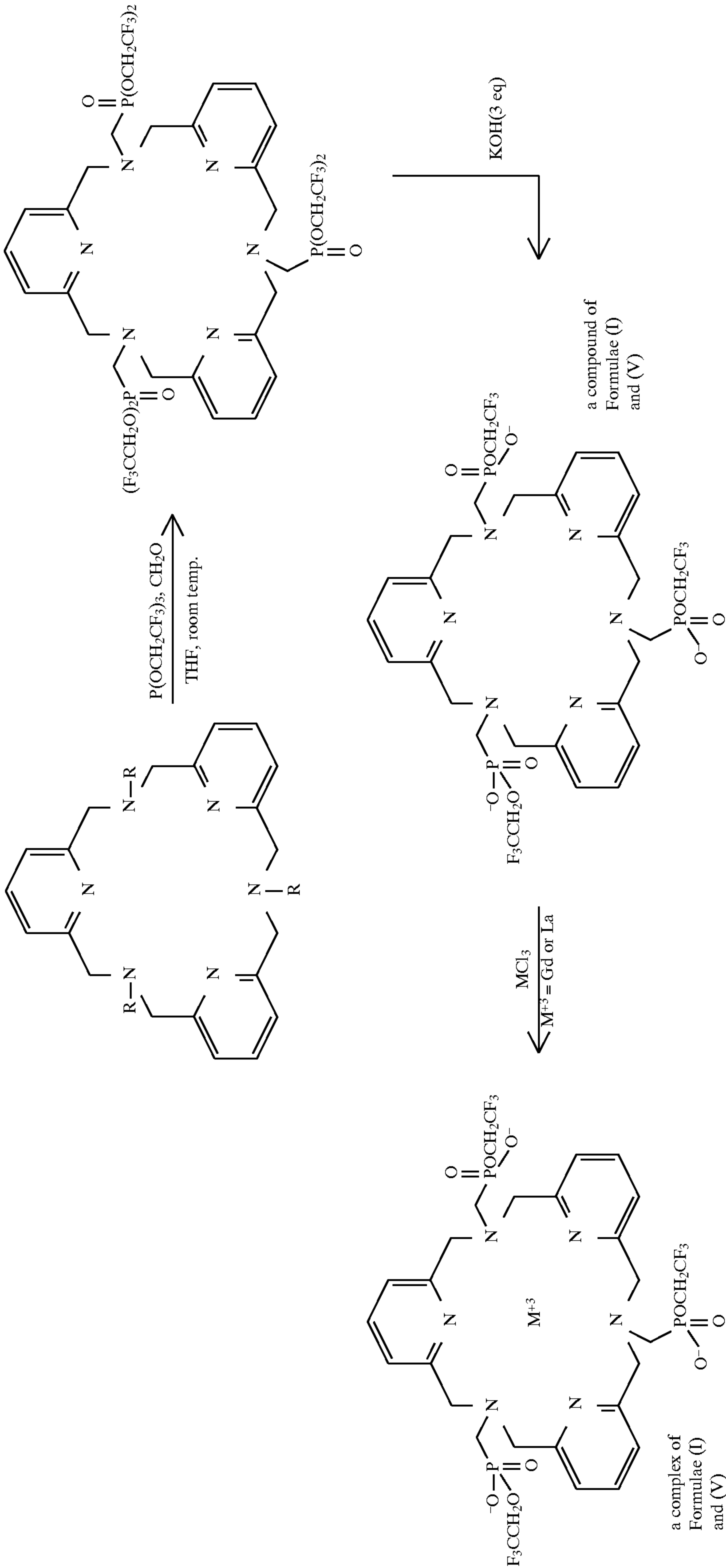
Scheme 4
