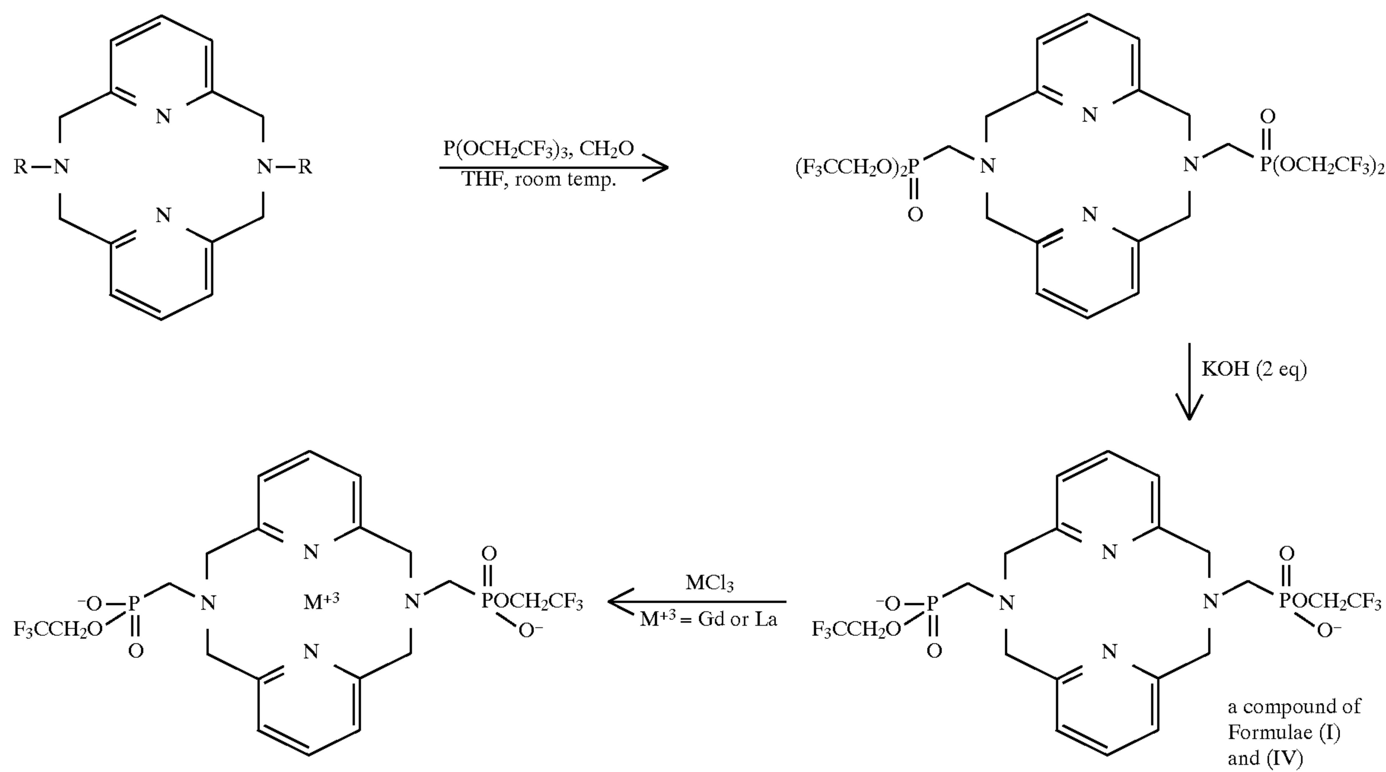
Scheme 3
