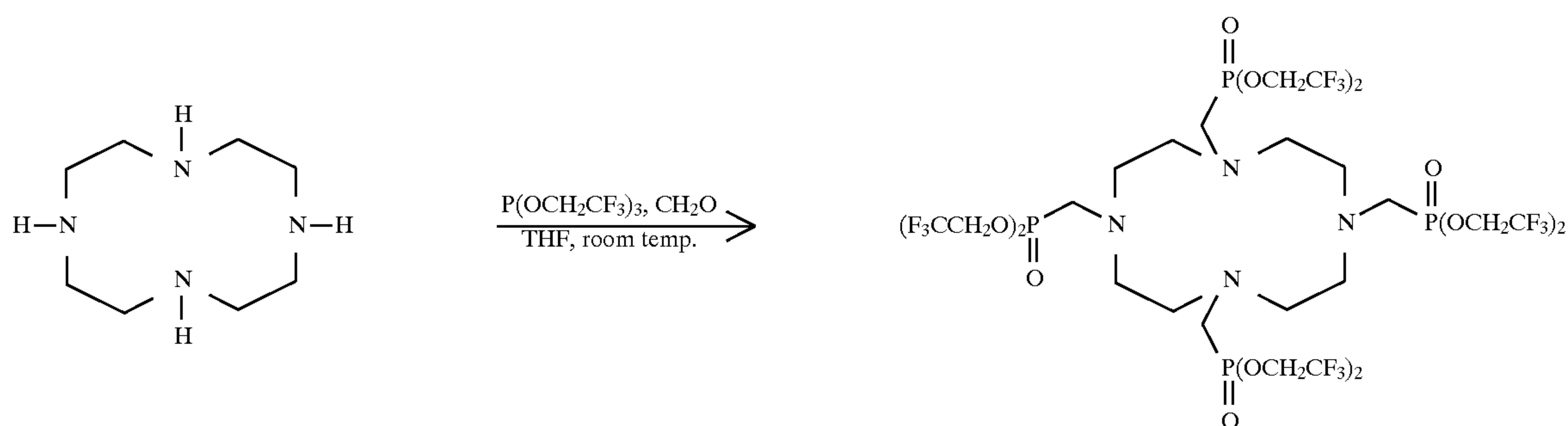
Scheme 1
