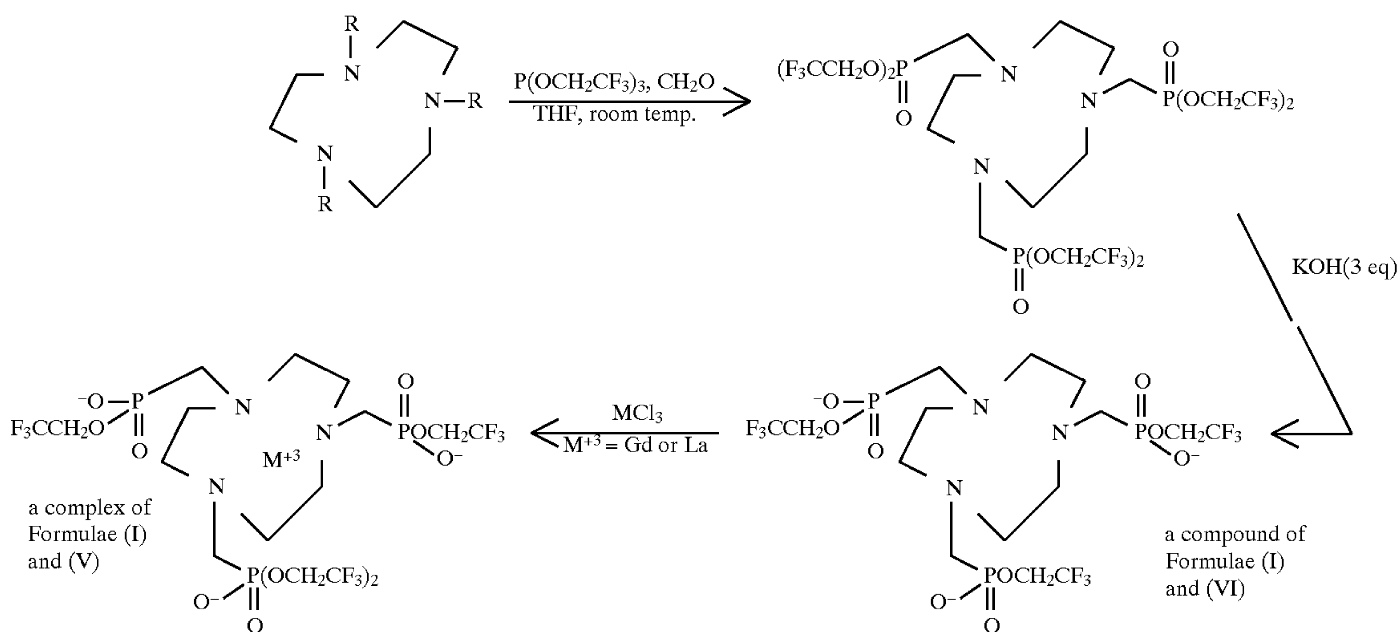
Scheme 5
