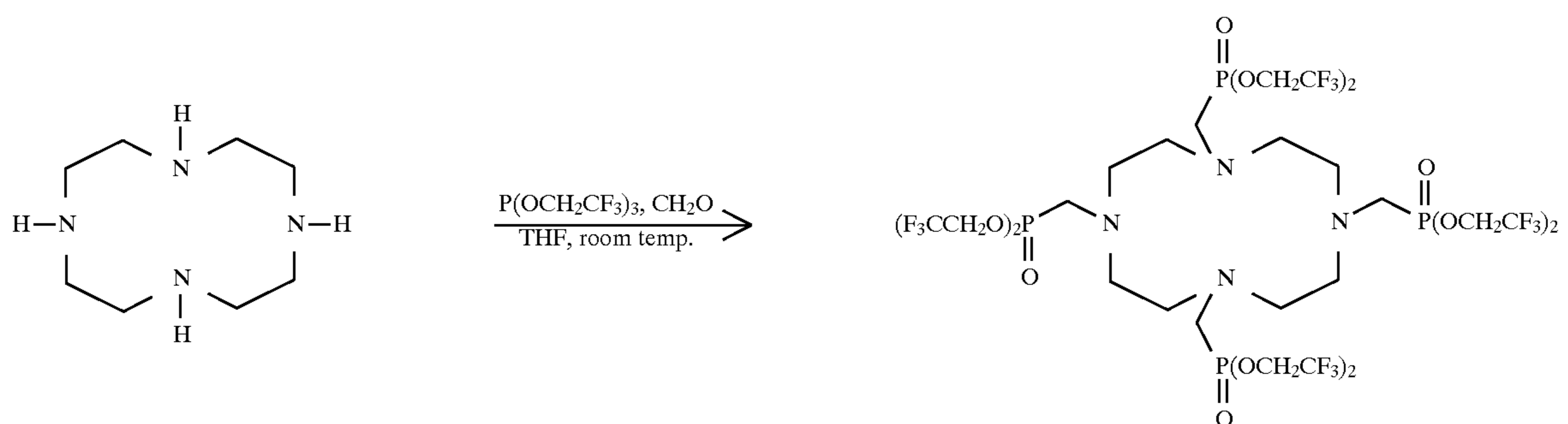
Scheme 1
