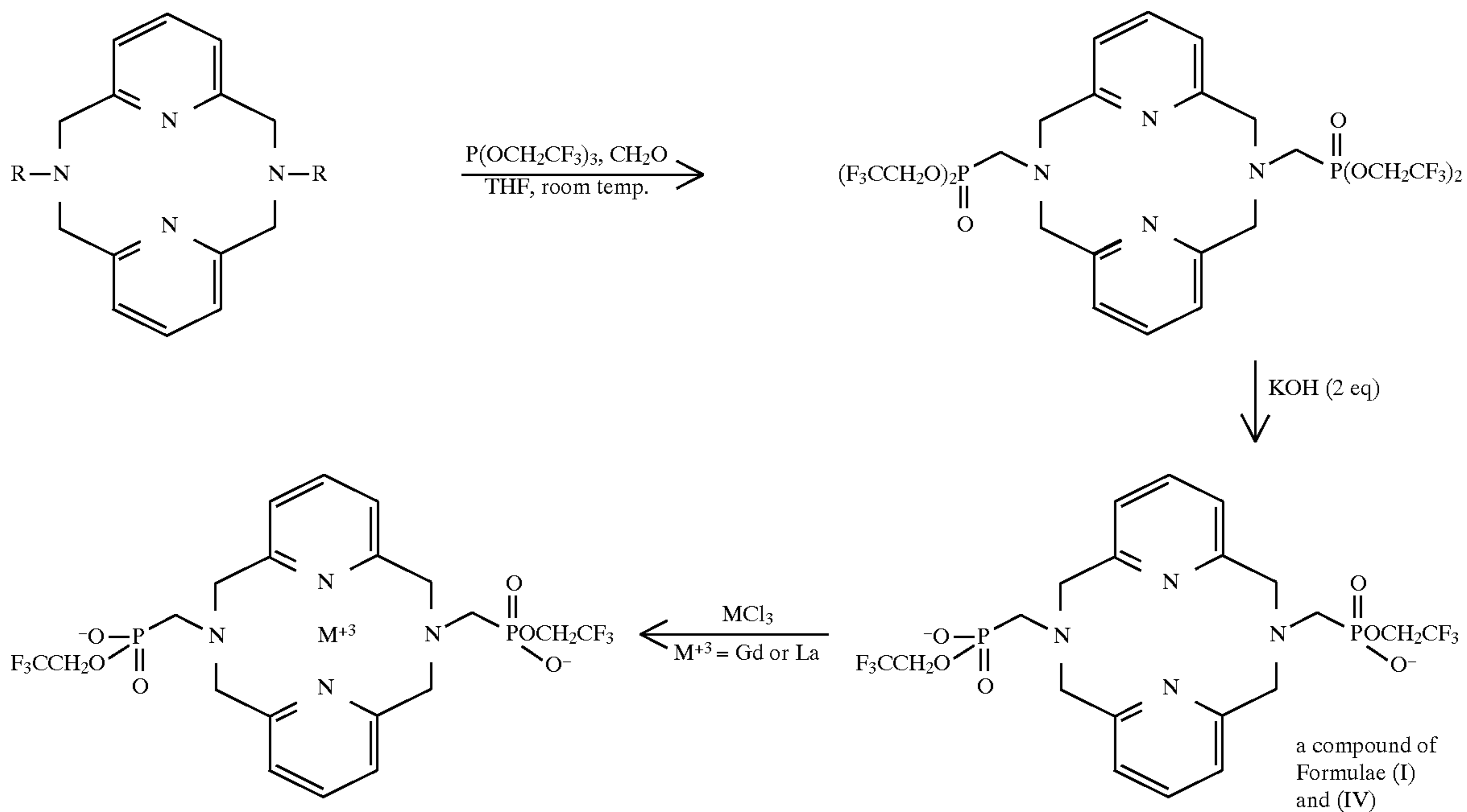
Scheme 3
