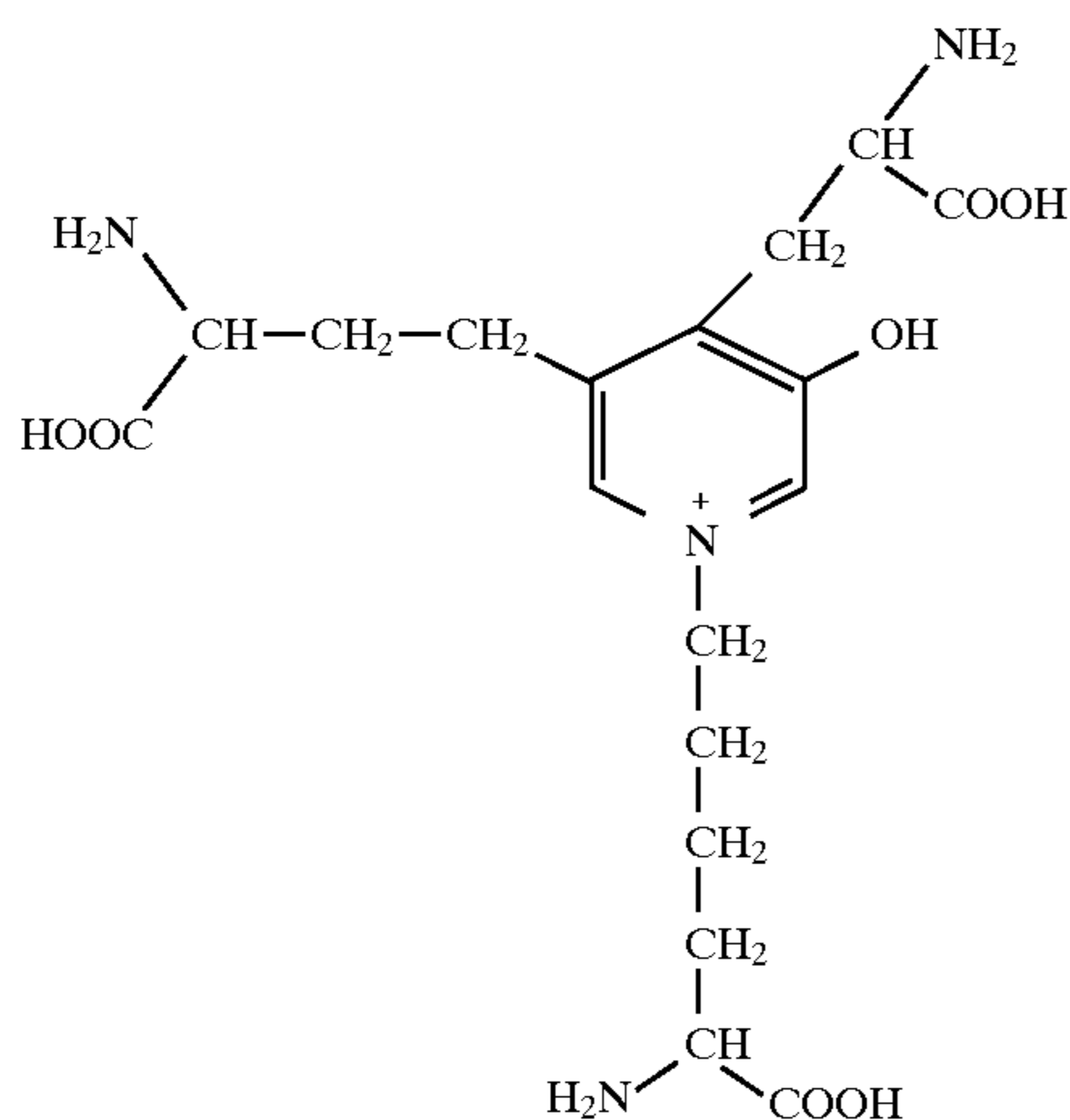
lysyl pyridinoline (LP)
