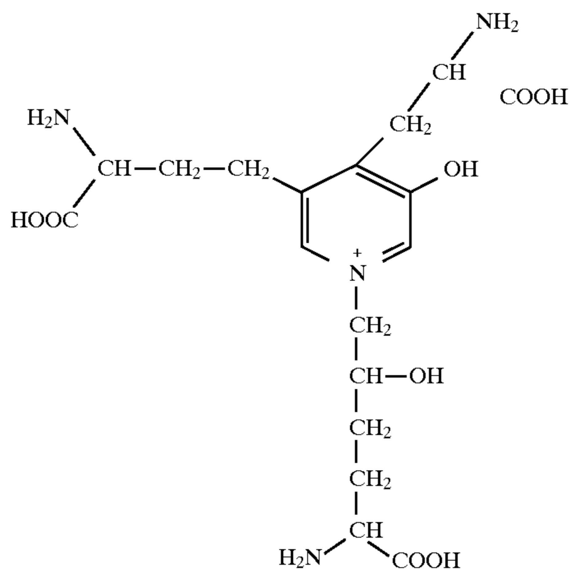
hydroxylysyl pyridinoline (HP)
