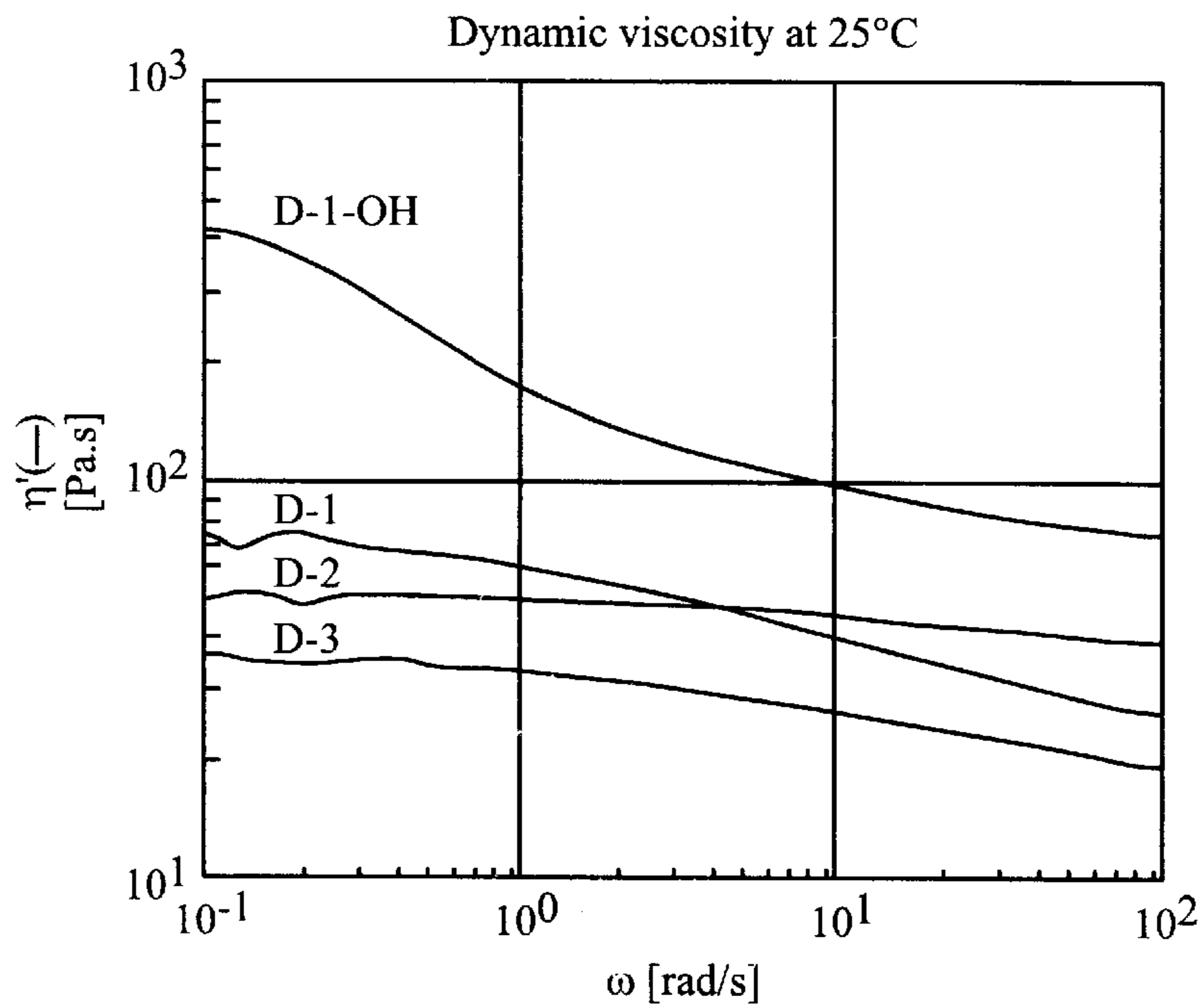
Dynamic viscosity of the hyperbranched (meth)acrylated polyesters.
