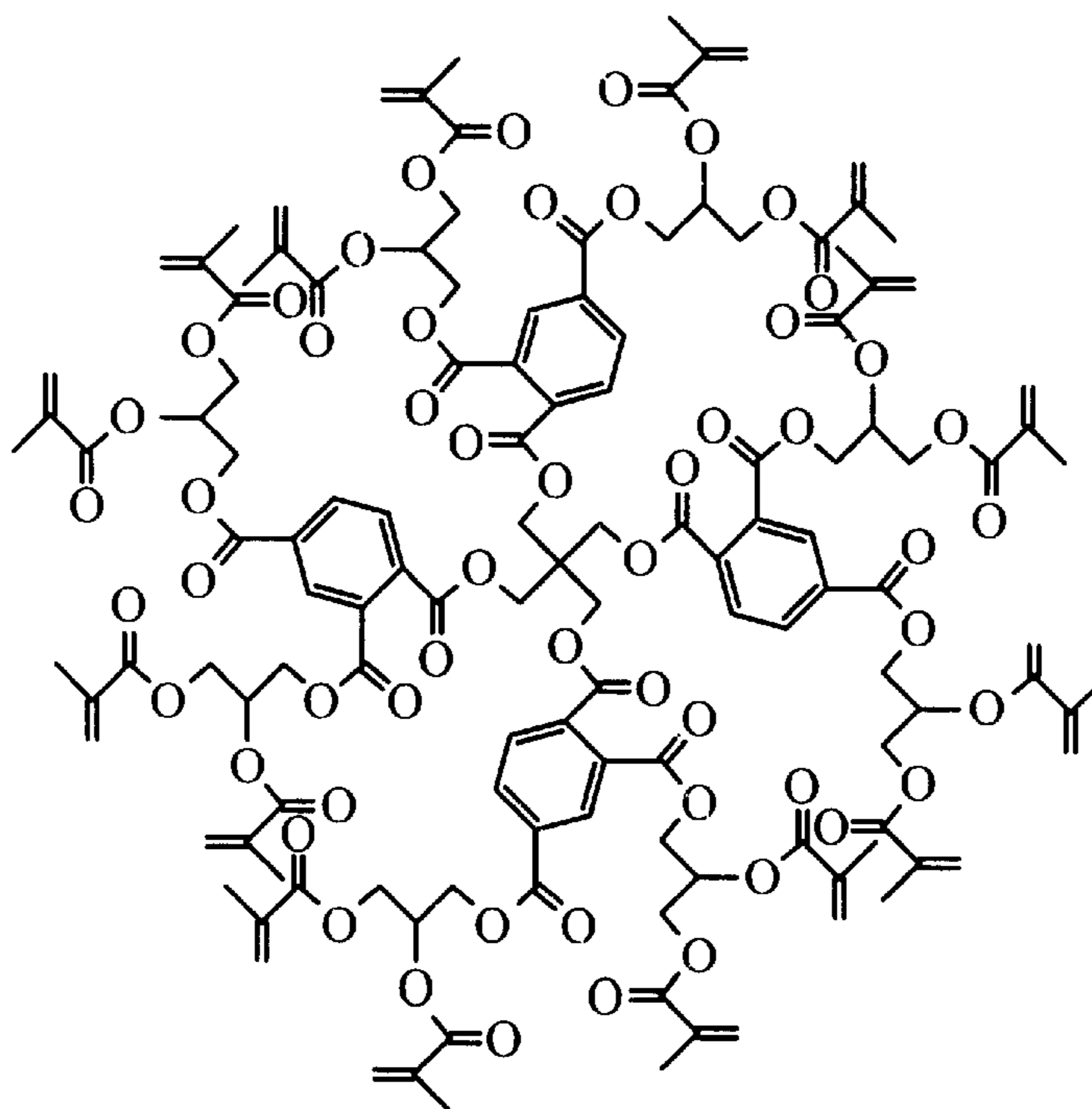
Idealized formula of the hyperbranched methacrylated polyester with 16 double bonds.
