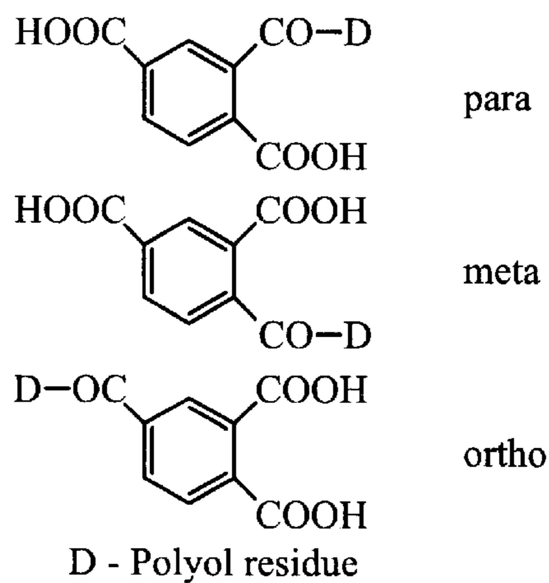
Molecular structure of the three polyolester isomers.
