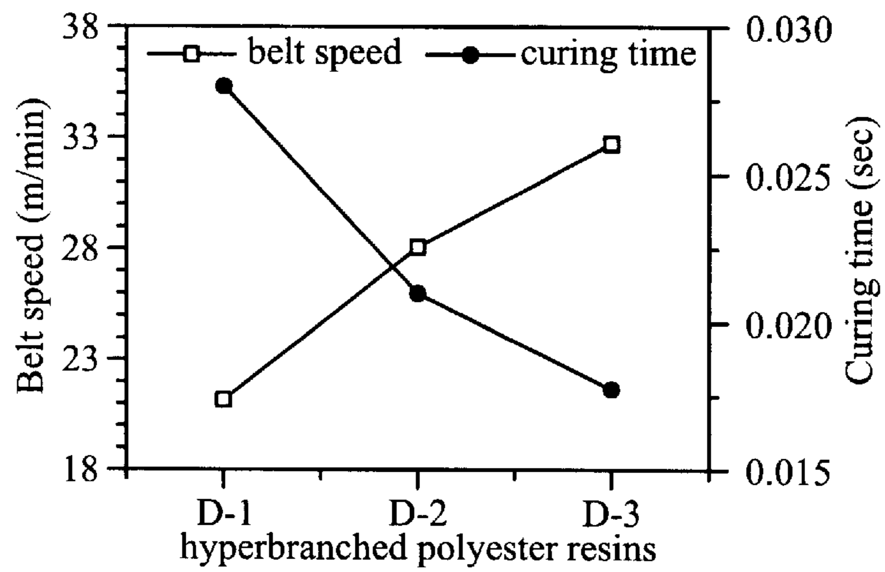
Curing time and belt speed to tack-free state for UV cured polyester films
