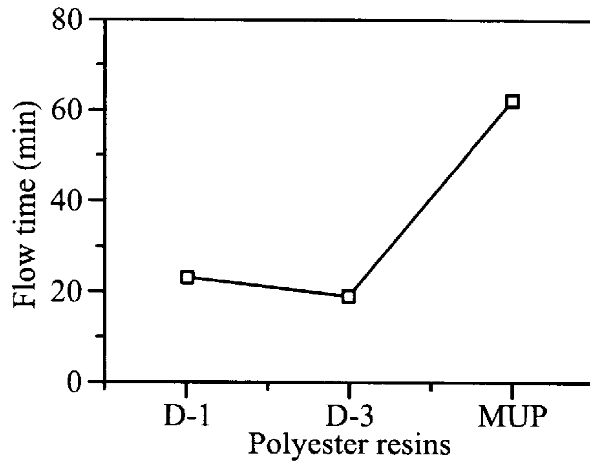
Flow time of hyperbranched polyesters and MUP using viscometric cup
