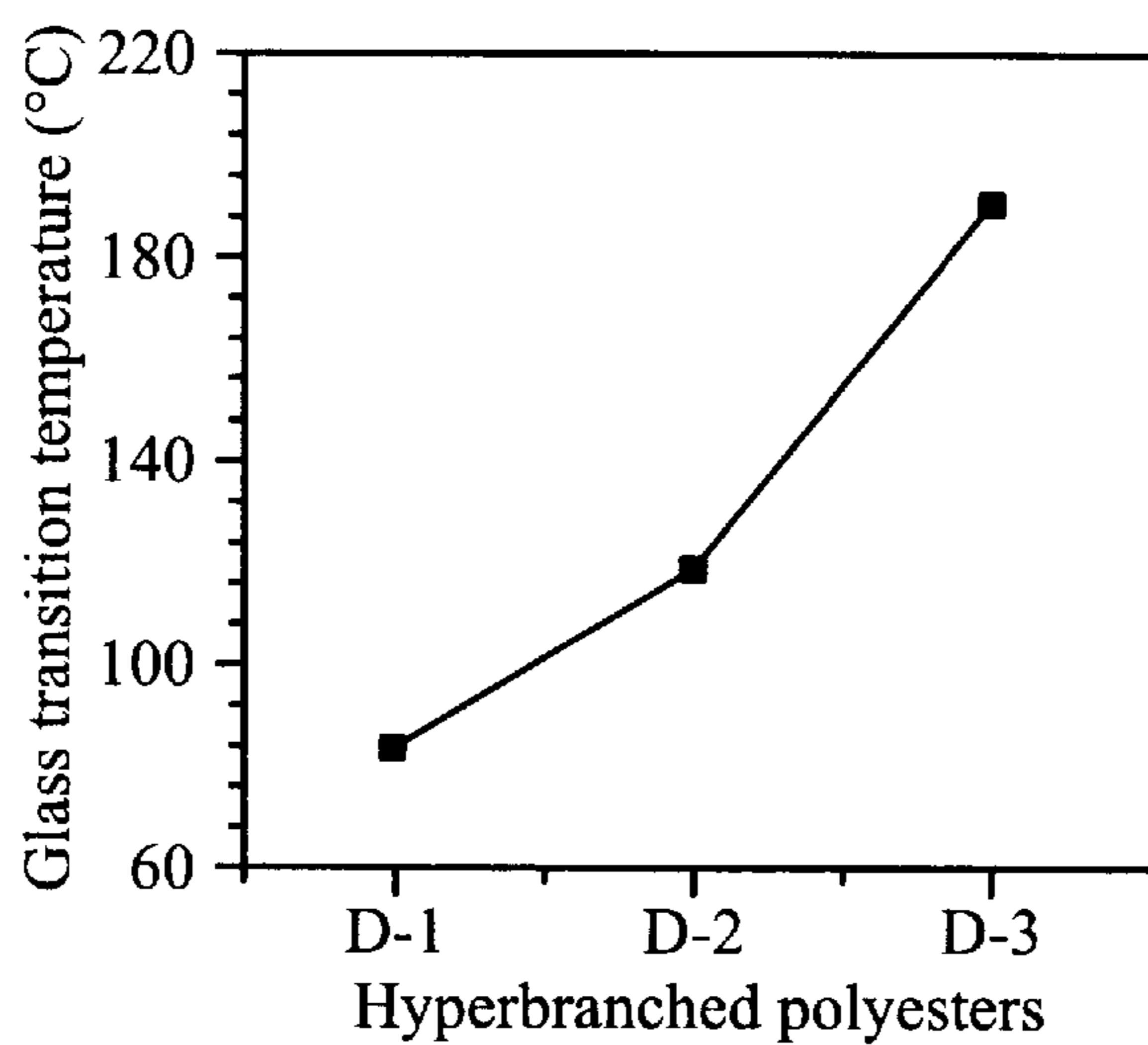
Glass transition temperatures of the cured hyperbranched polyesters.
