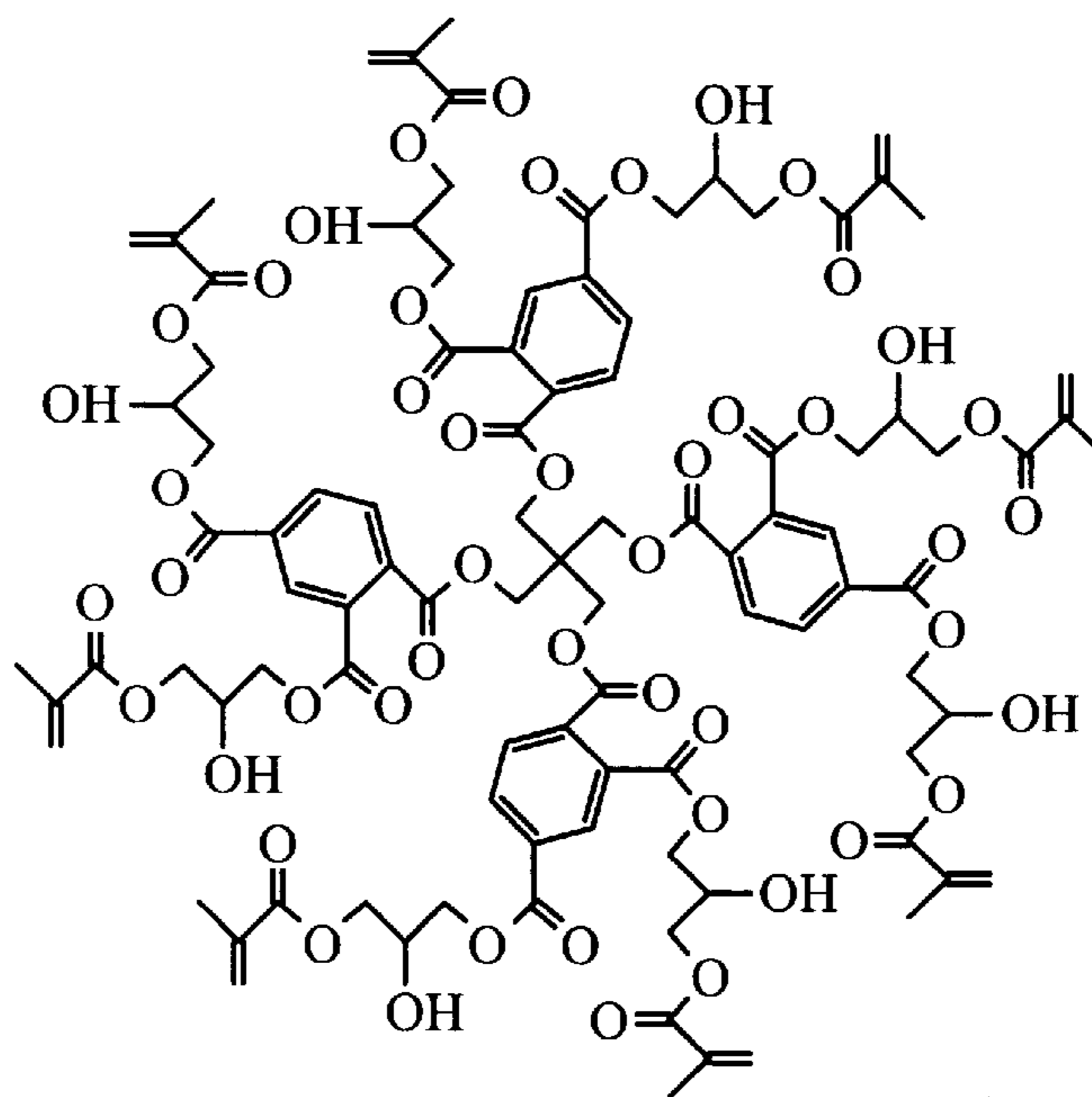
Idealized formula of the hyperbranched methacrylated polyester with 8 double bonds.
