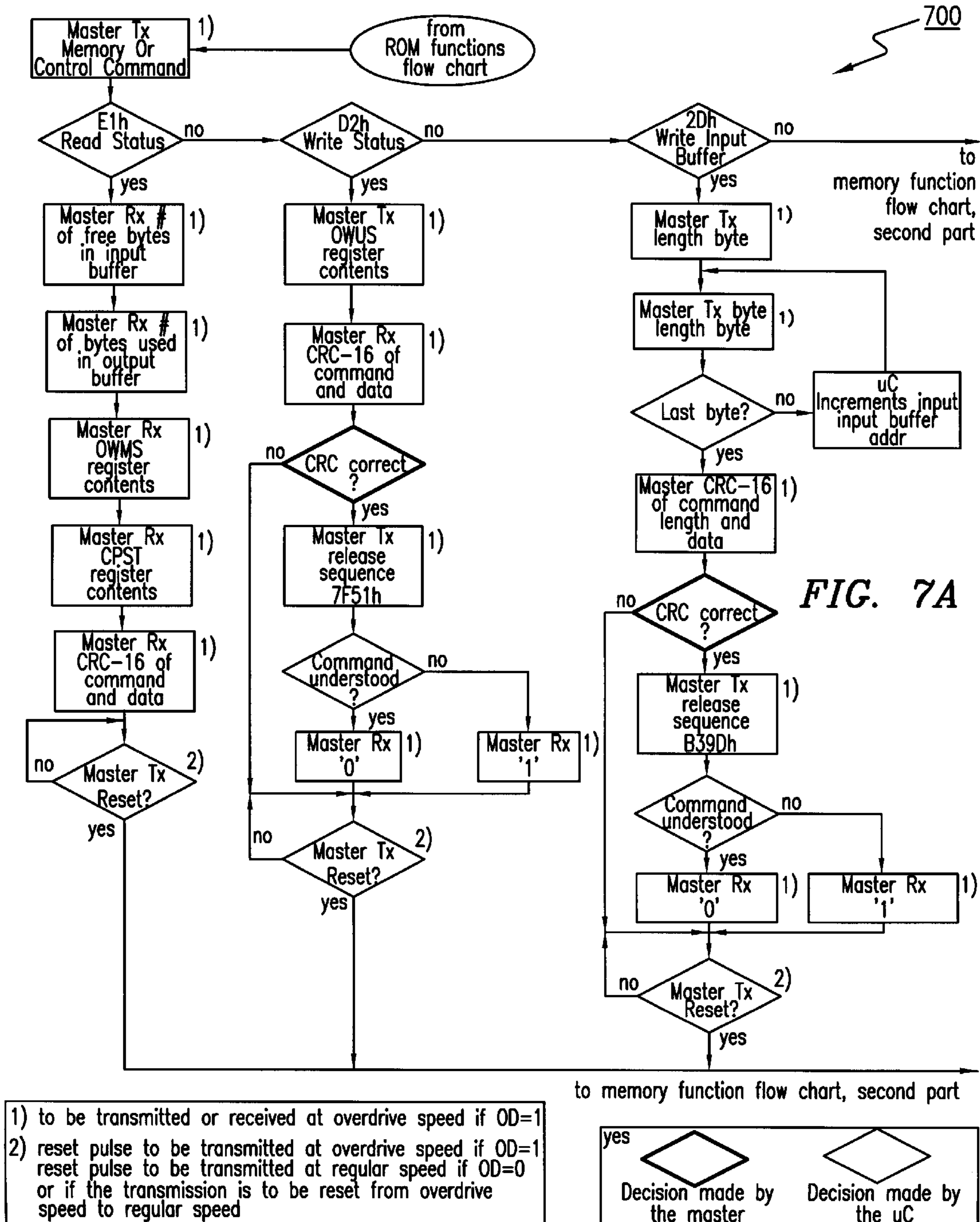
Slave One Wire Memory Function Flow Chart
