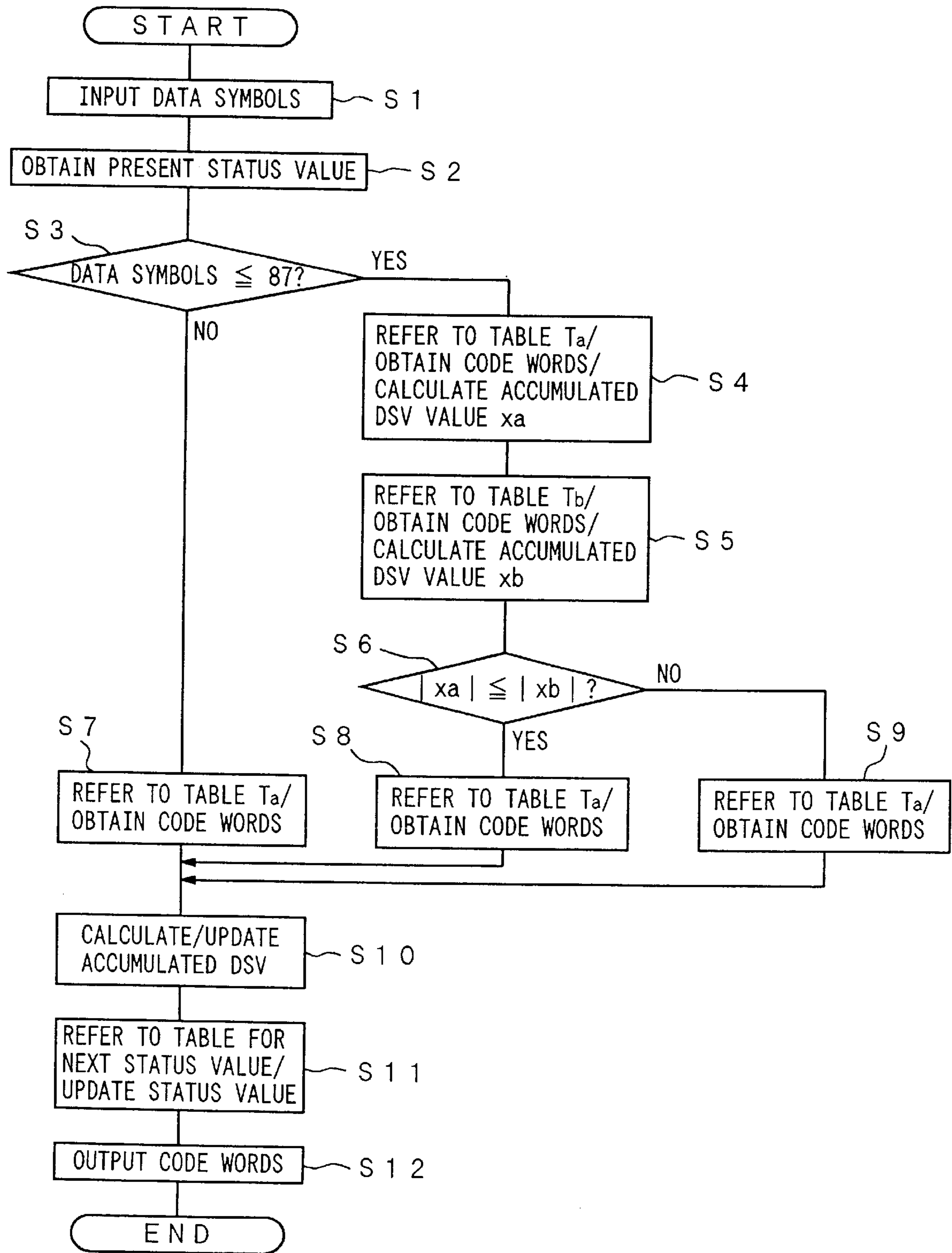
FLOWCHART SHOWING AN EXAMPLE OF ALGORITHM OF MODULATION
