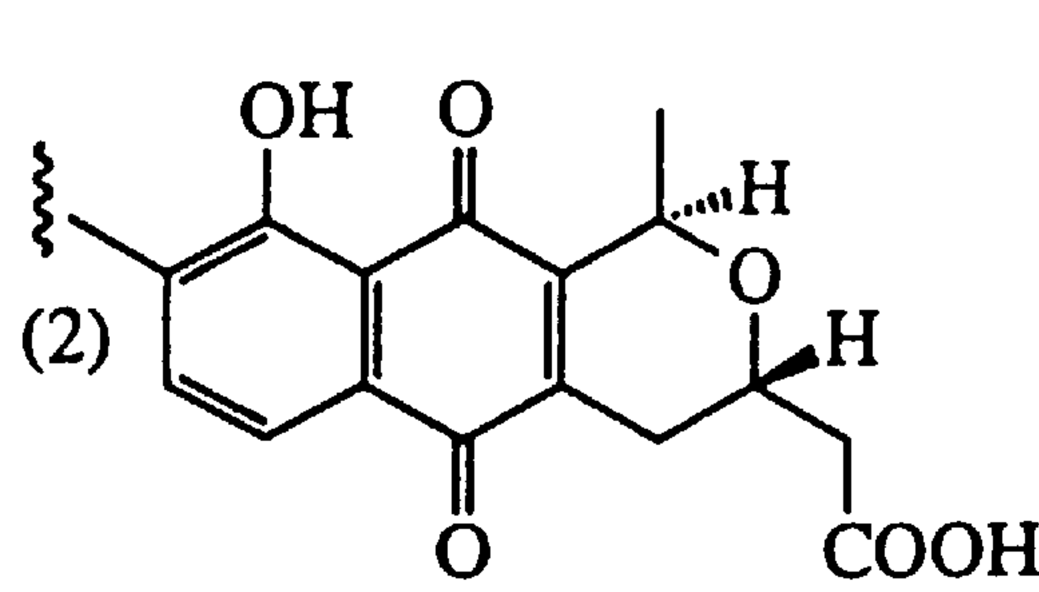
ACTINORHODIN (3)
