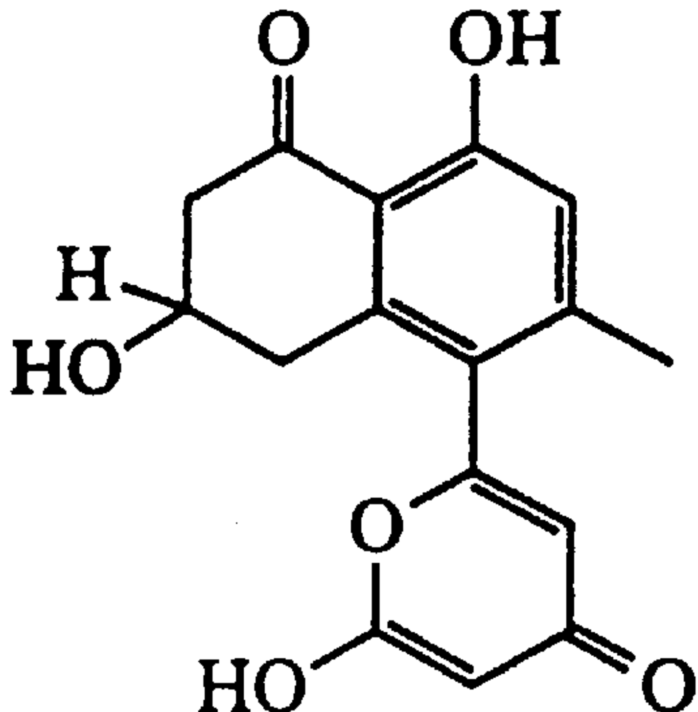
MUTACTIN (6)
