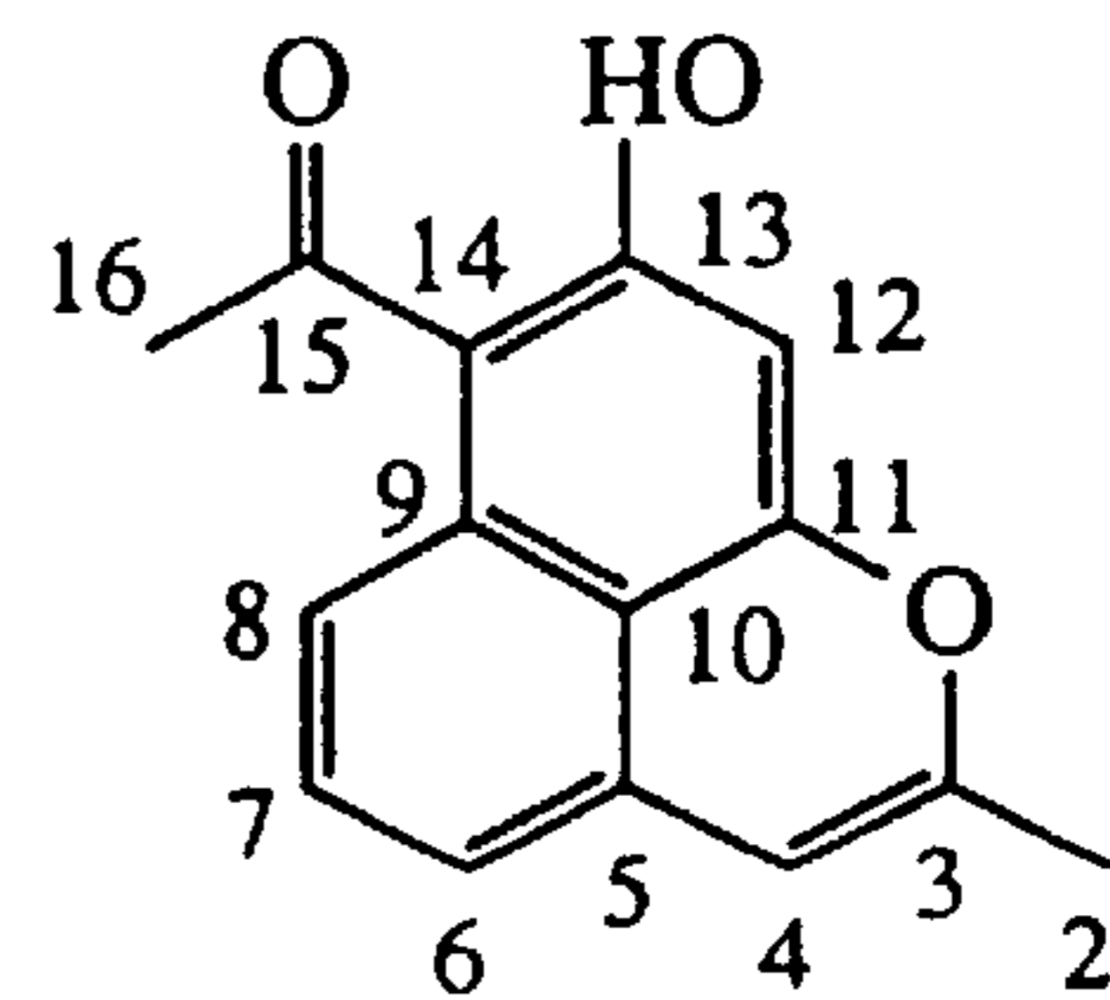
RM 18b (11)
