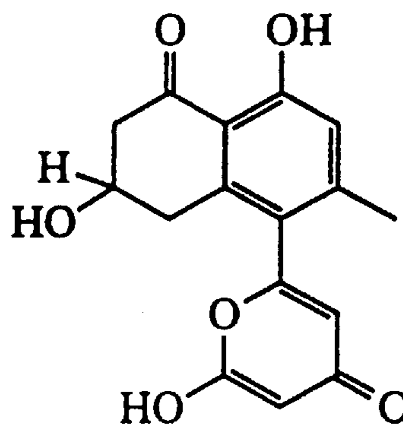
MUTACTIN (6)
