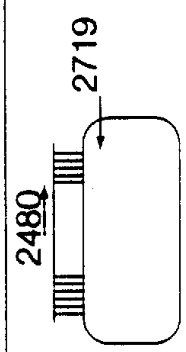
Homologous recombination colony PCR:
