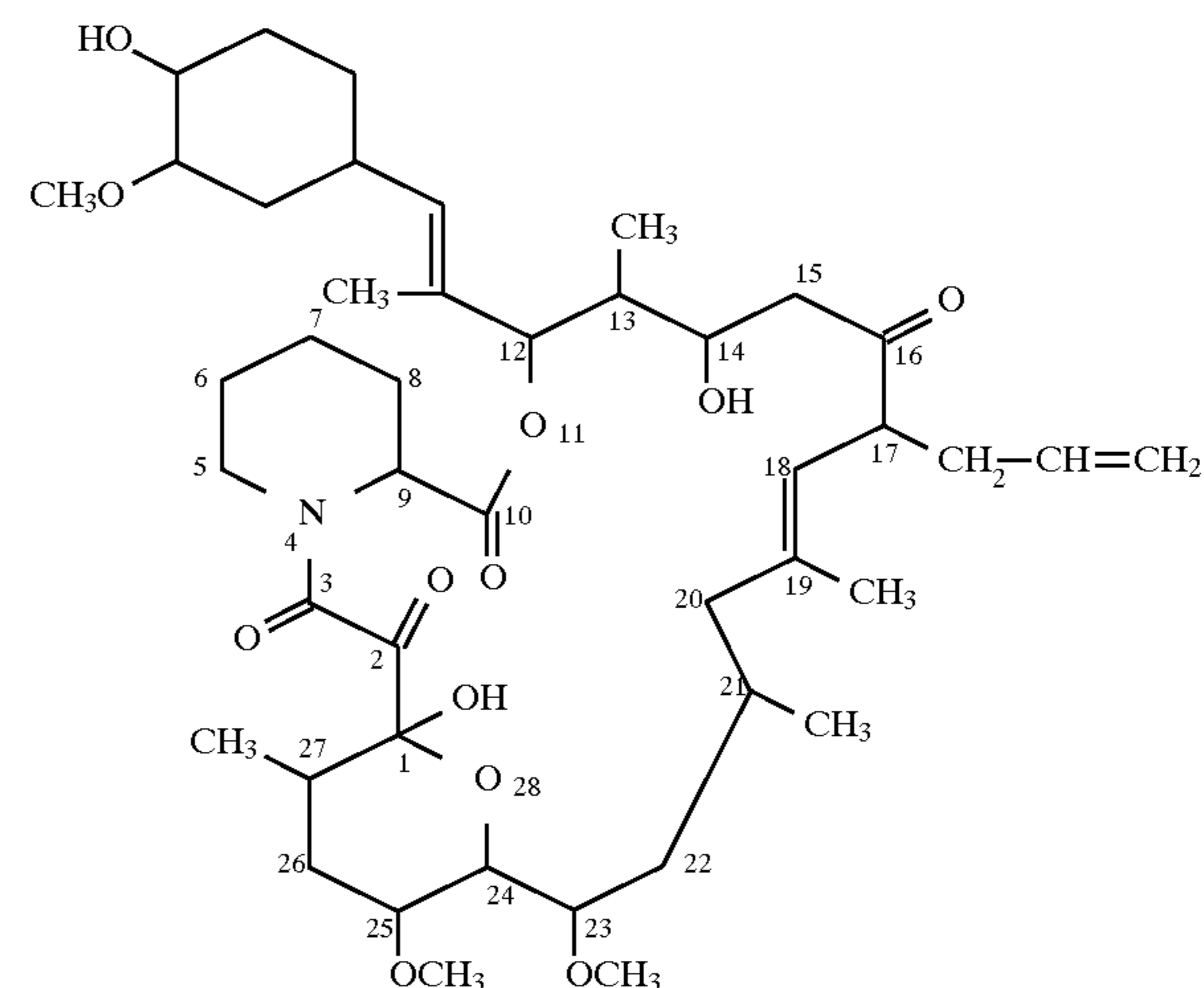
17-Allyl-1,14-dihydroxy-12-[2-(4-hydroxy-3-methoxycyclohexyl)-1-methylvinyl]-23,25-dimethoxy-13,19,21,27-tetramethyl-11,28-dioxo-4-azatricyclo[22.3.1.0 4,9 ]octacos-18-ene-2,3,10,16-tetraone
