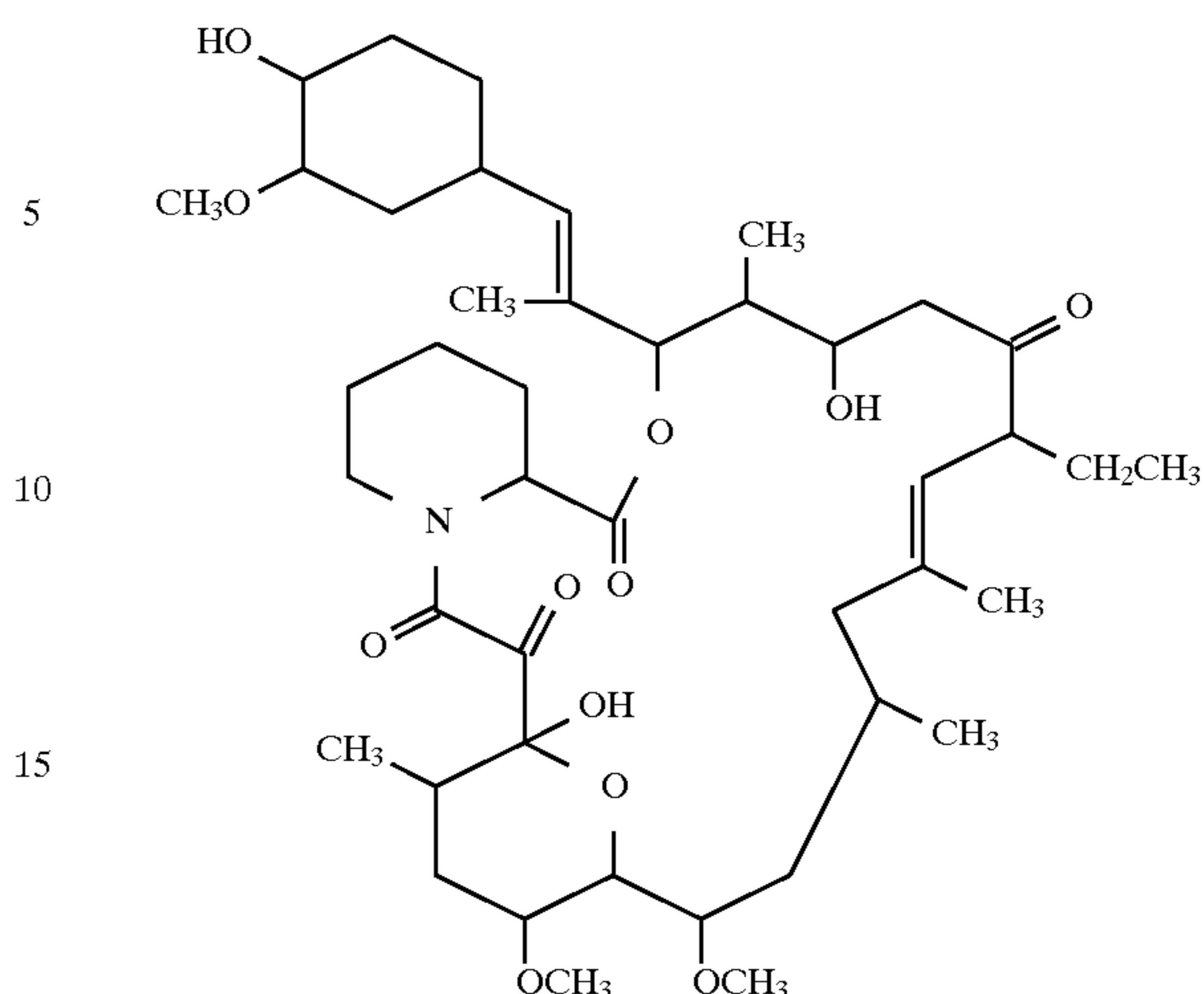
17-Ethyl-1,14-dihydroxy-12-[2-(4-hydroxy-3-methoxycyclohexyl)-1-methylvinyl]-23,25-dimethoxy-13,19,21,27-tetramethyl-11,28-dioxo-4-azatricyclo-[22.3.1.0 4,9 ]octacos-18-ene-2,3,10,16-tetraone
