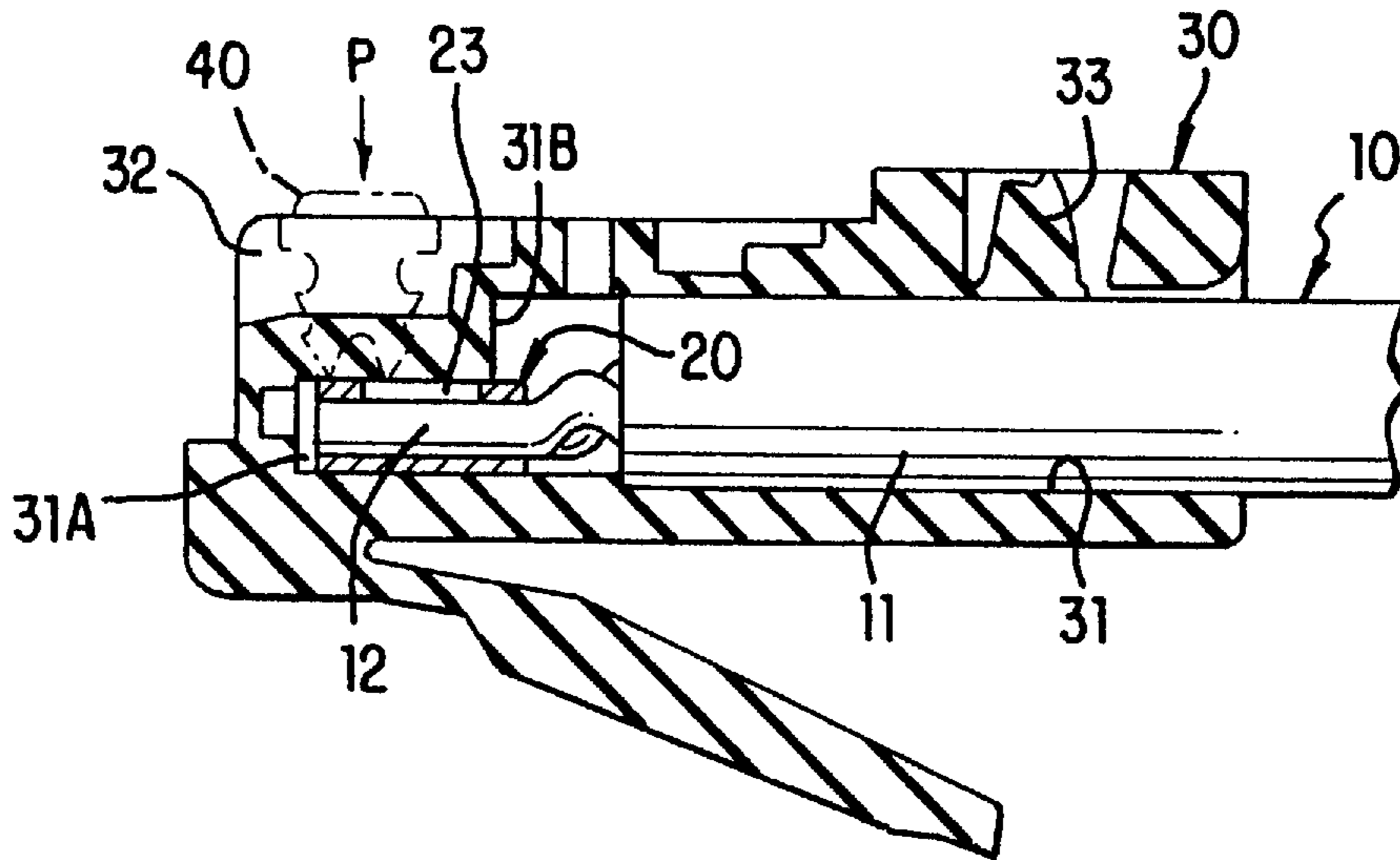
FIG. 8 PRIOR ART
