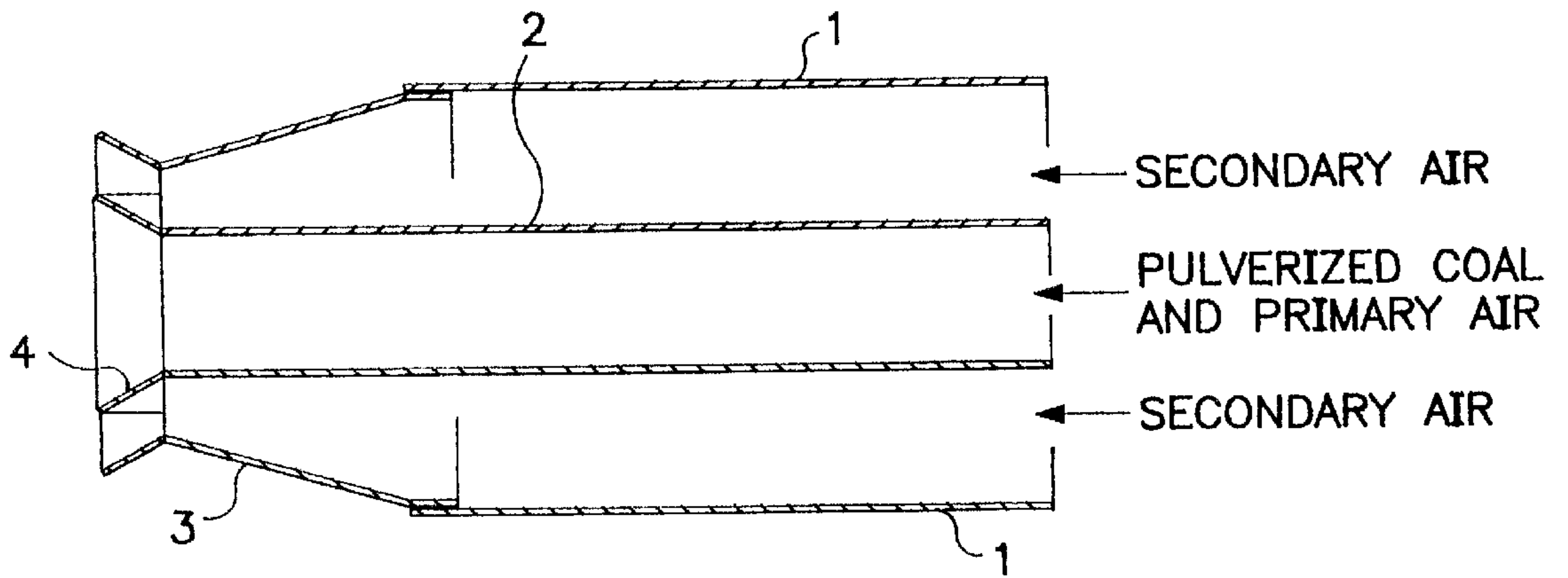
FIG. 28 PRIOR ART
