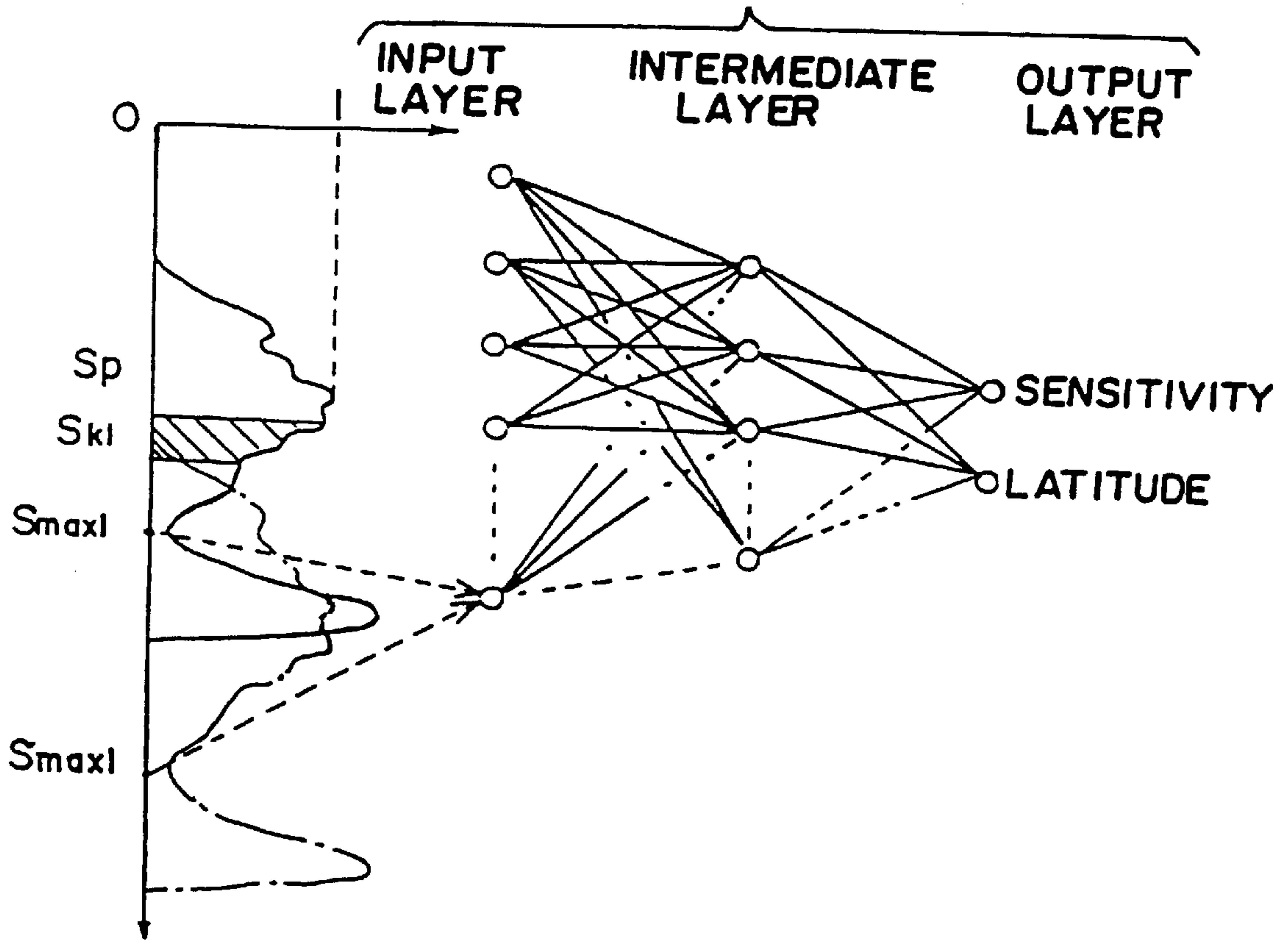
NEURAL NETWORK
