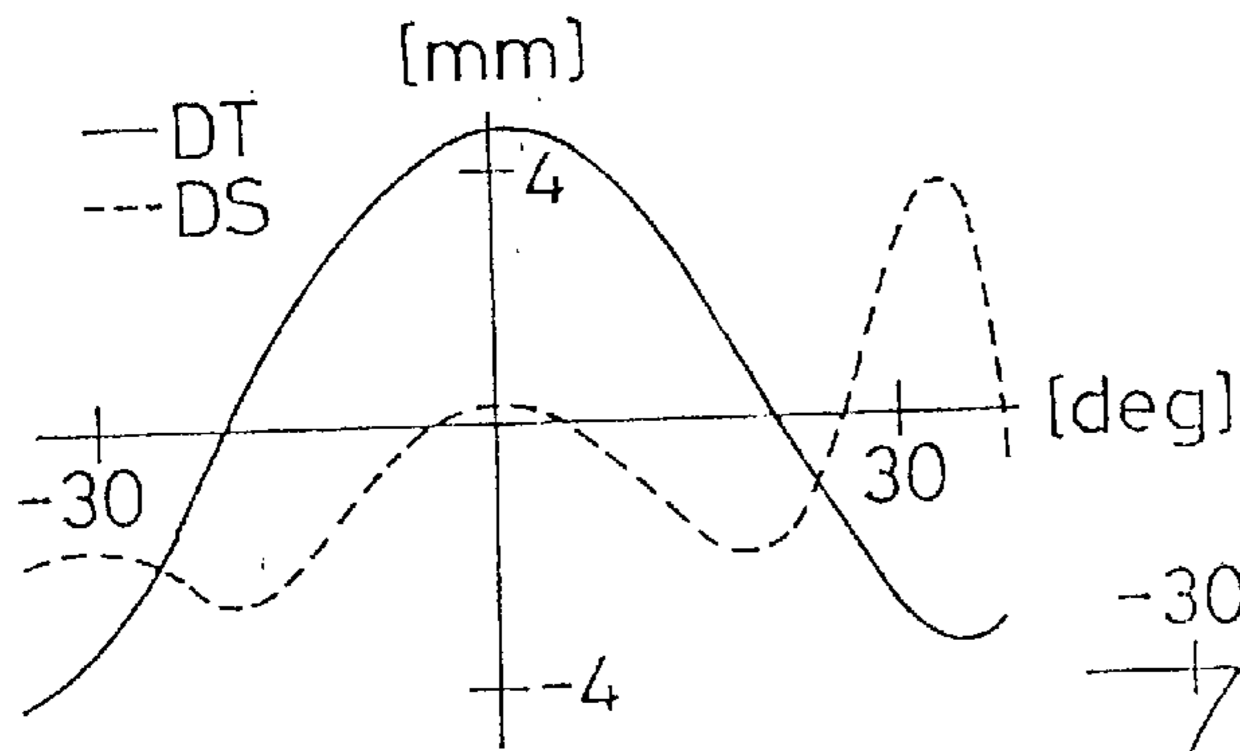
FIELD CURVATURE
