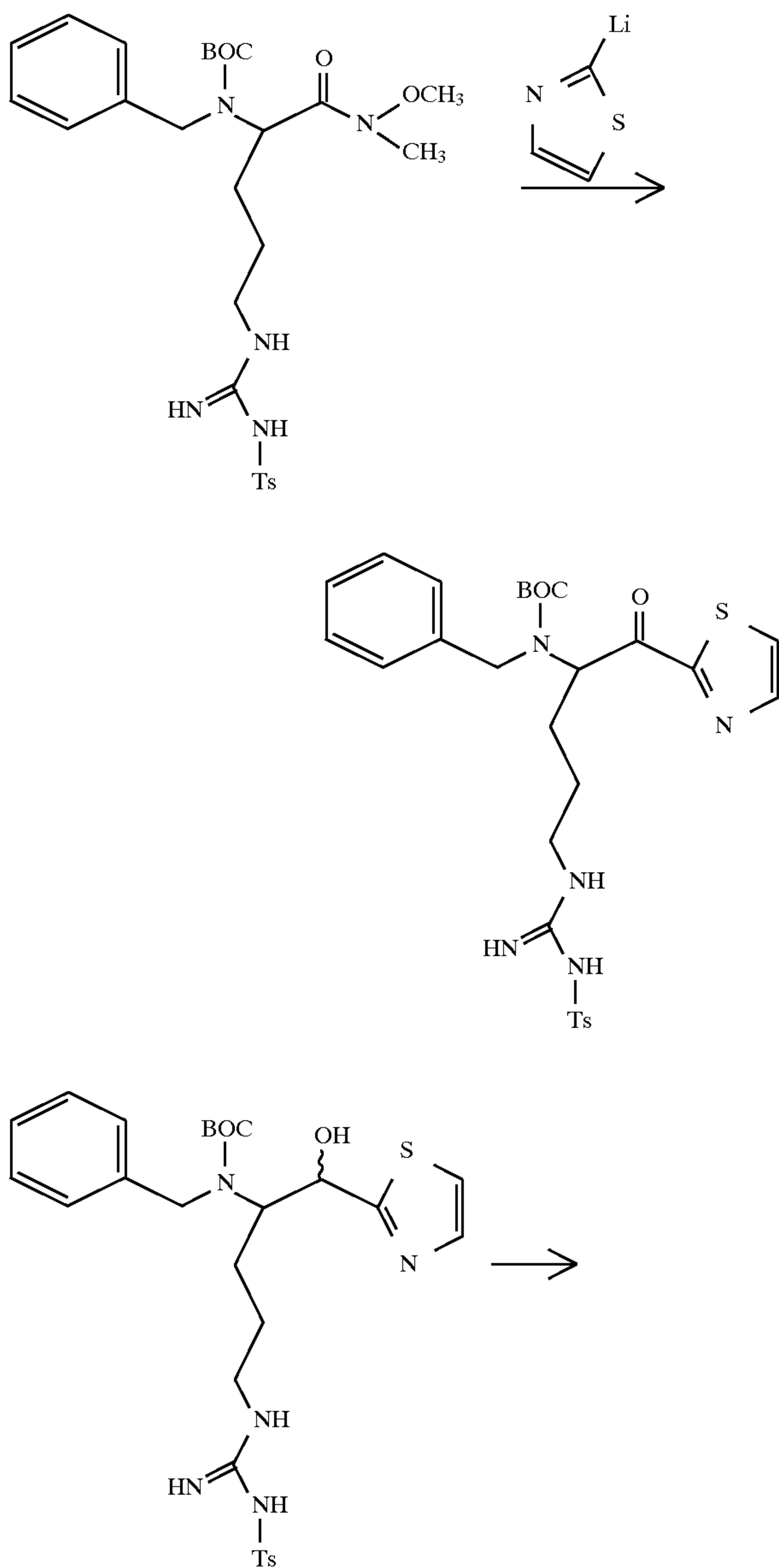
SCHEME IIA
