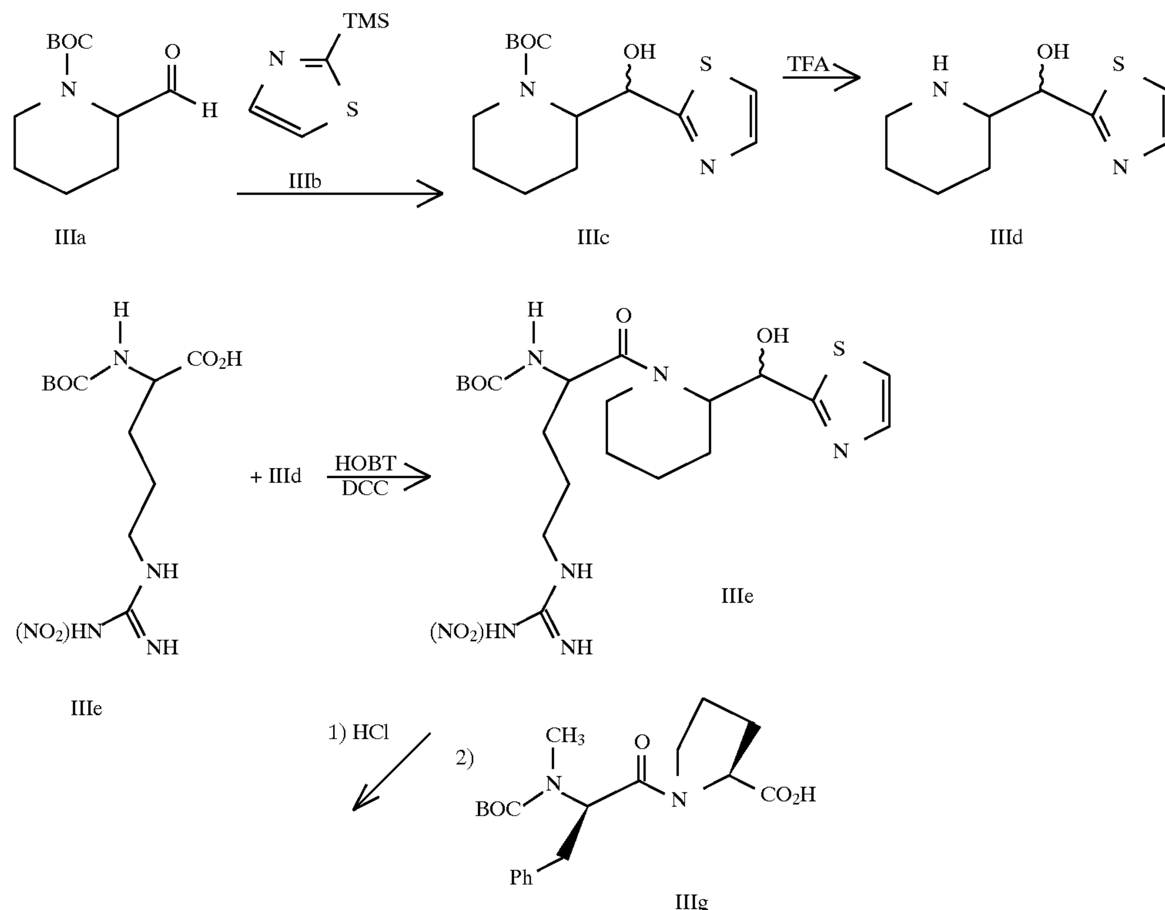
SCHEME III
