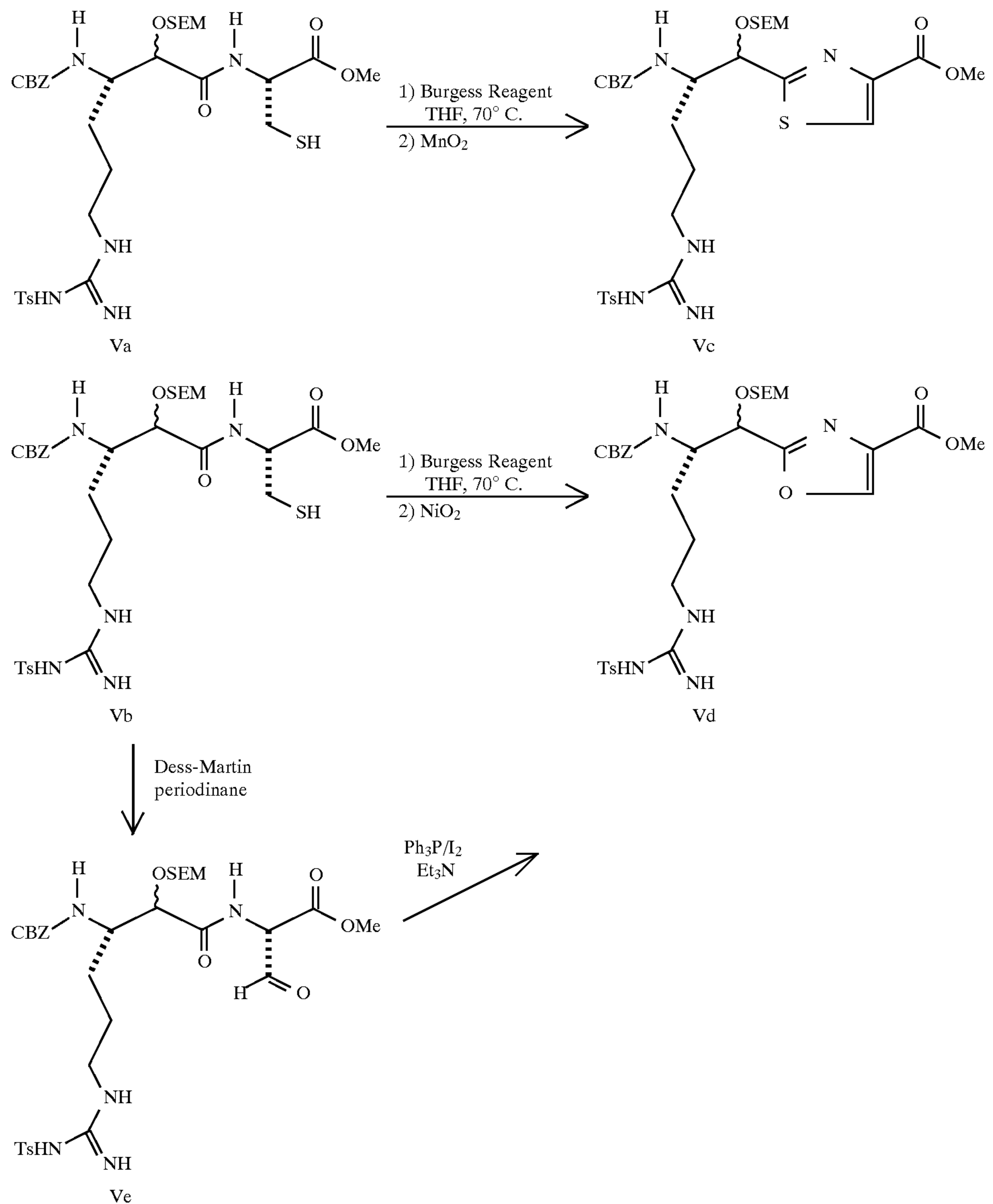
SCHEME V
