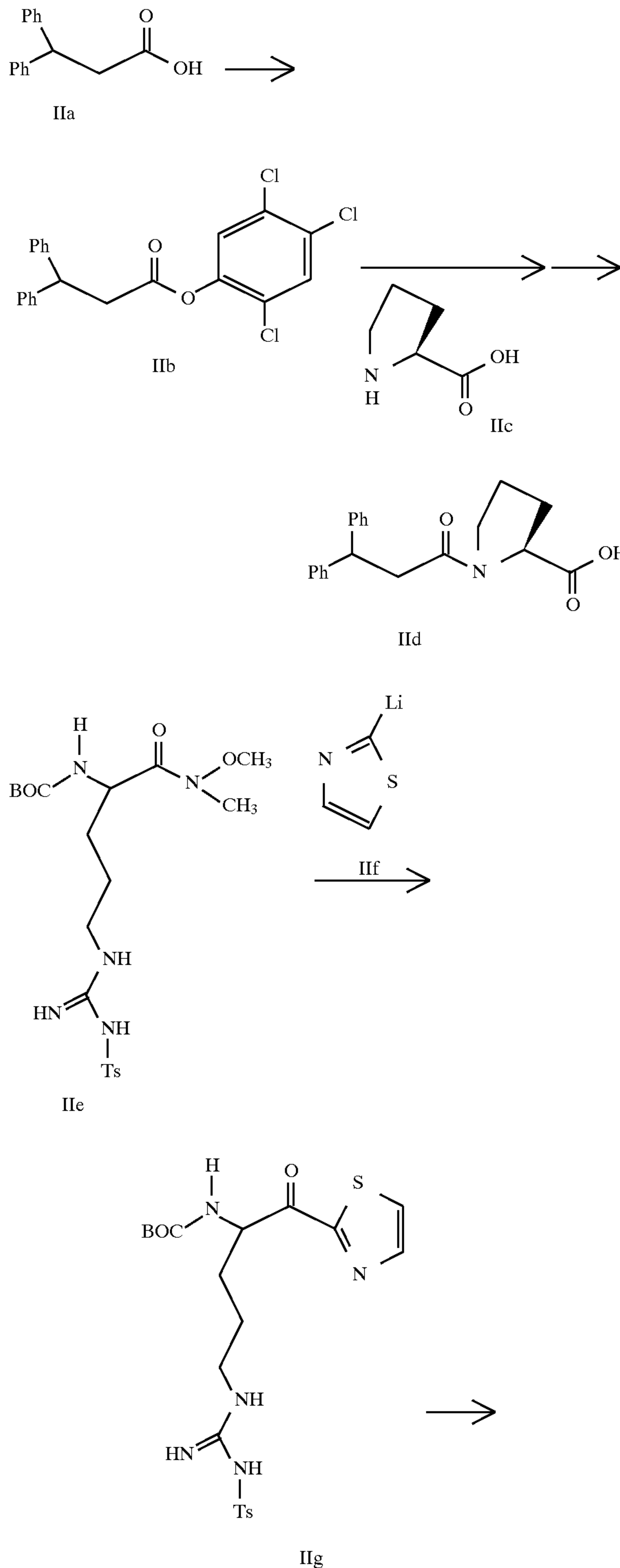
SCHEME II
