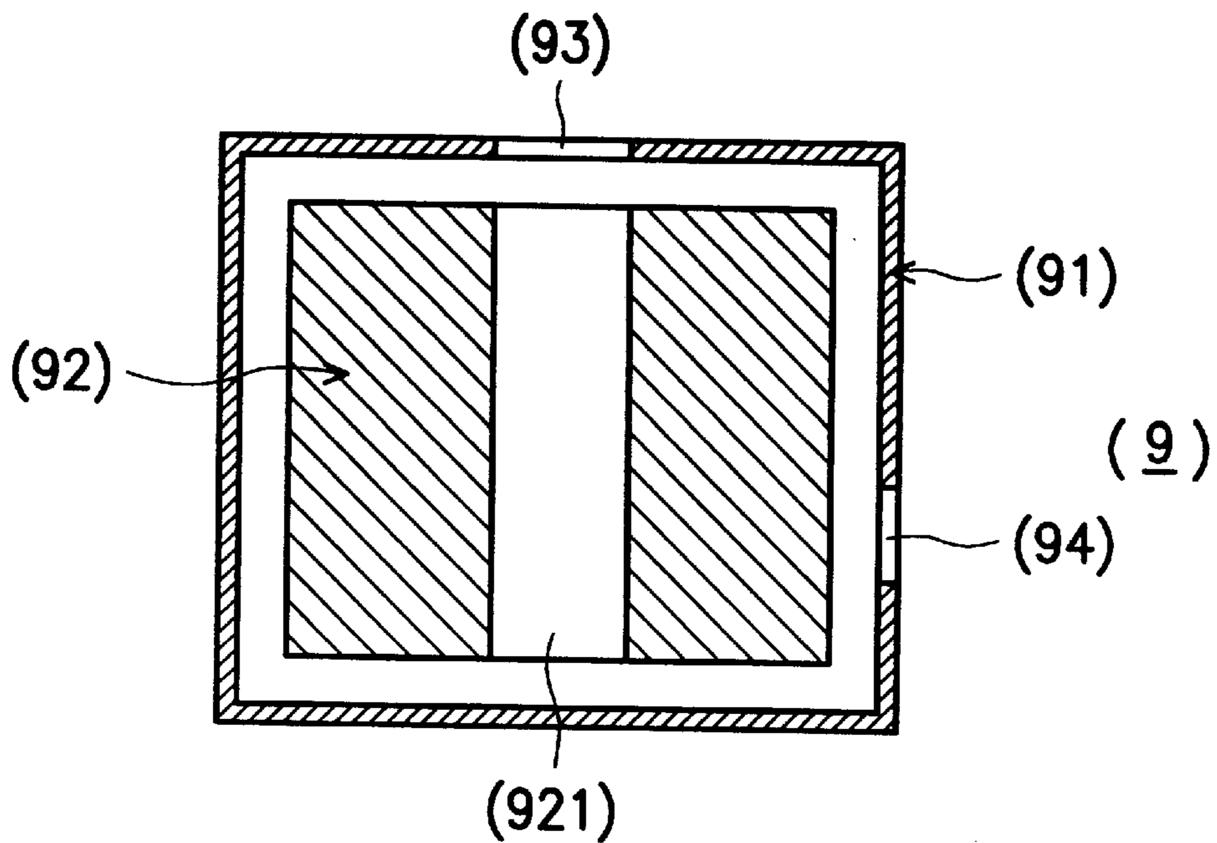
FIG. 10 (PRIOR ART)
