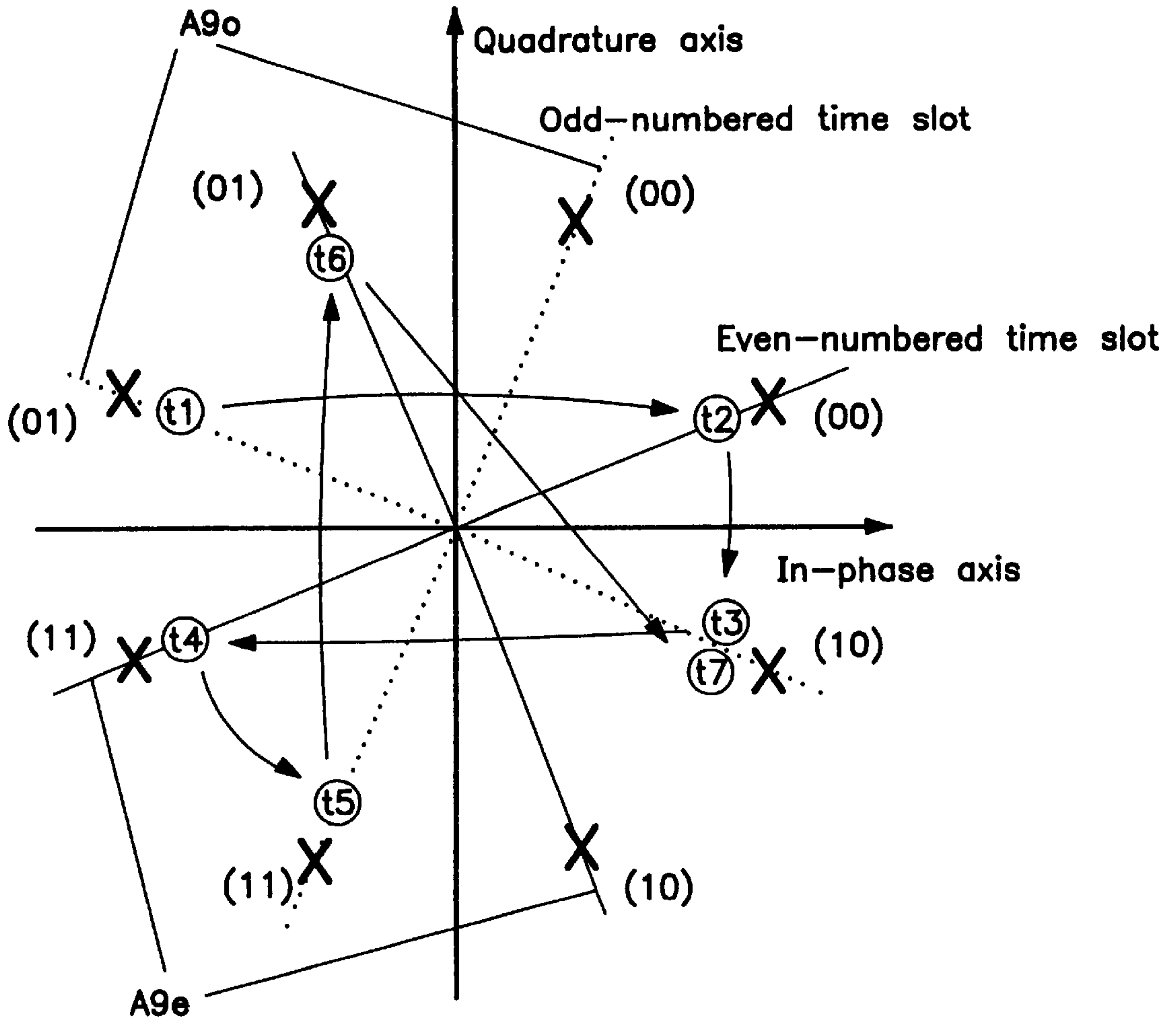
FIG. 10 PRIOR ART
