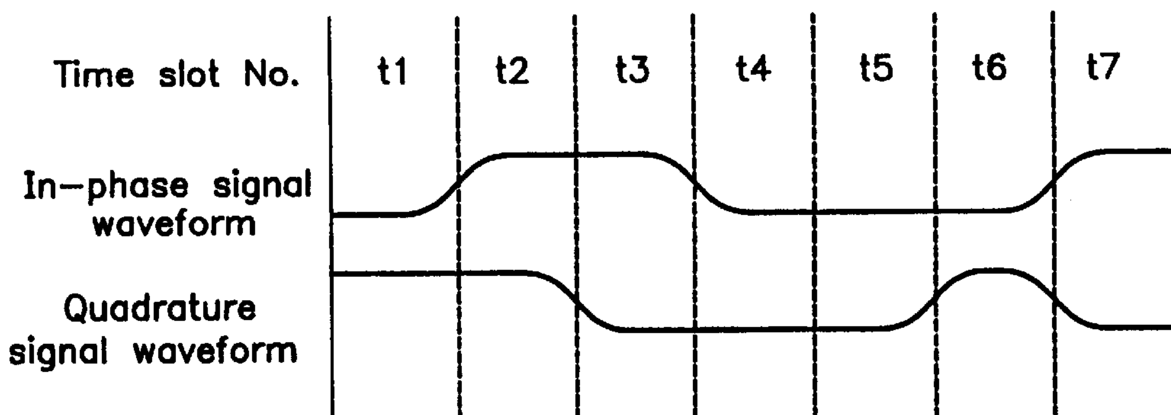
FIG. 5C PRIOR ART
