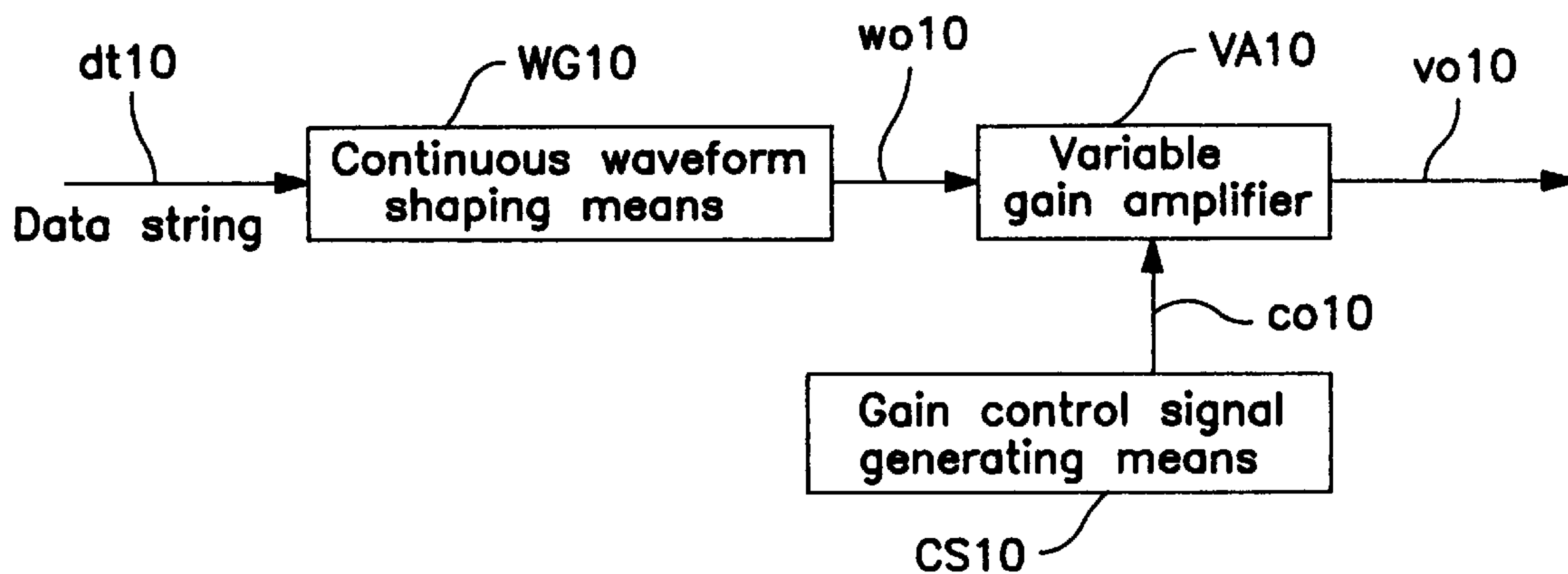
FIG. 11 PRIOR ART
