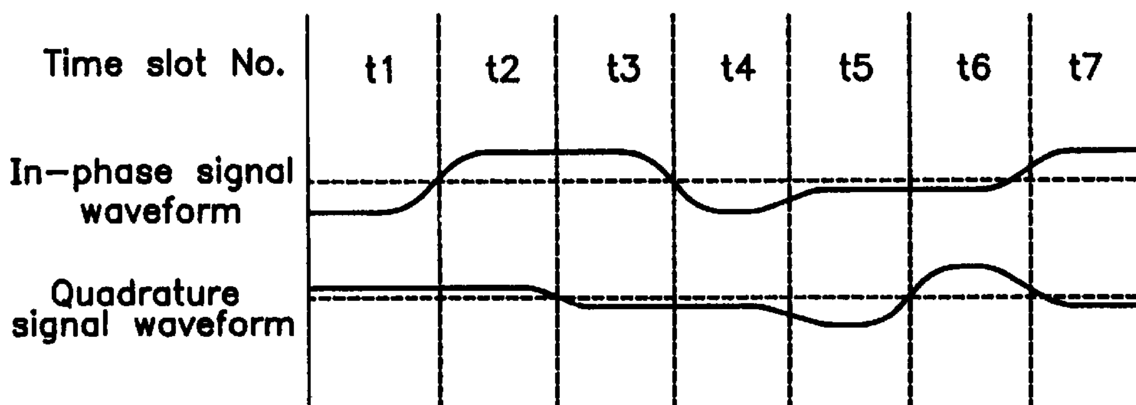
FIG. 9C PRIOR ART
