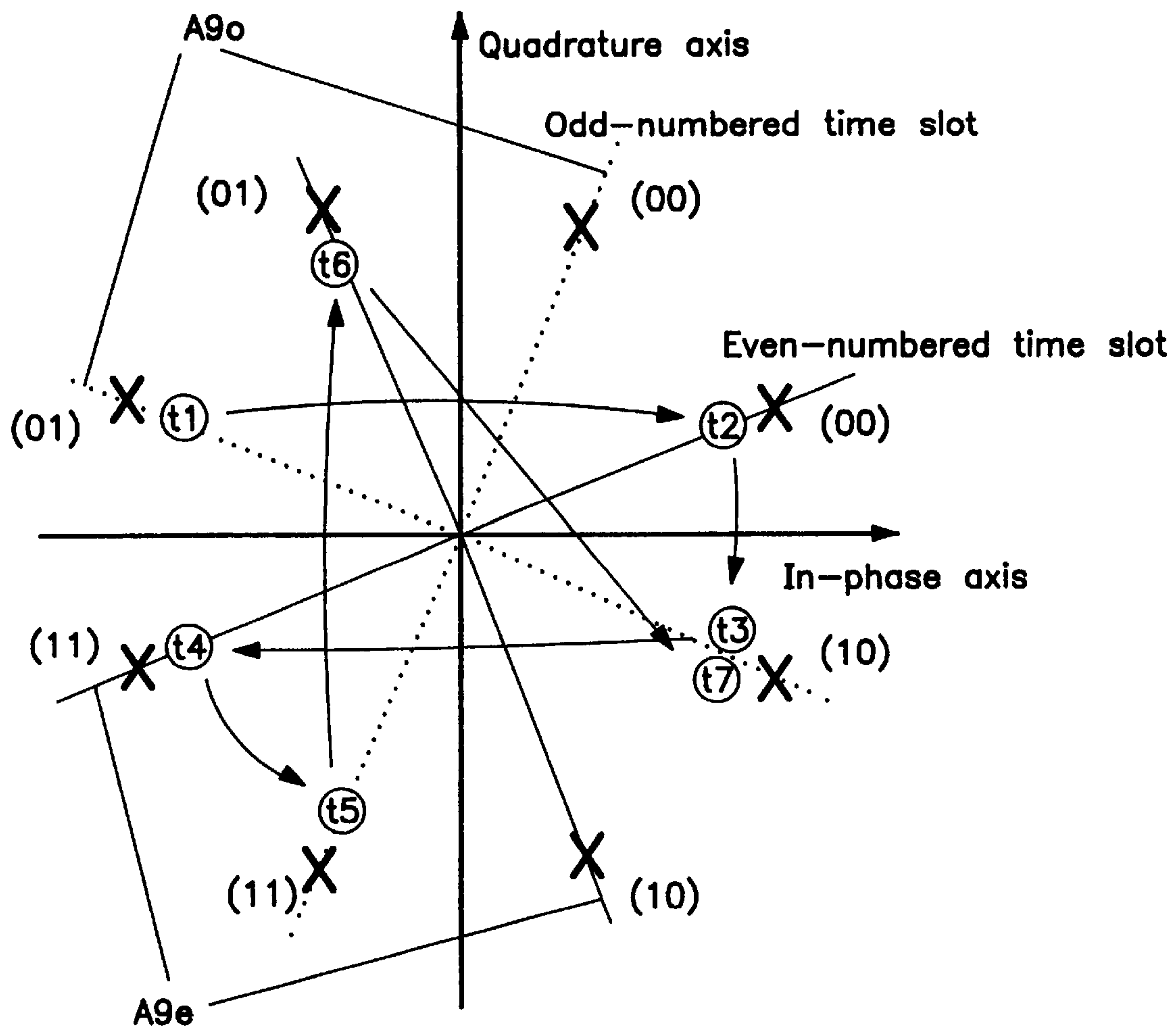
FIG. 10 PRIOR ART
