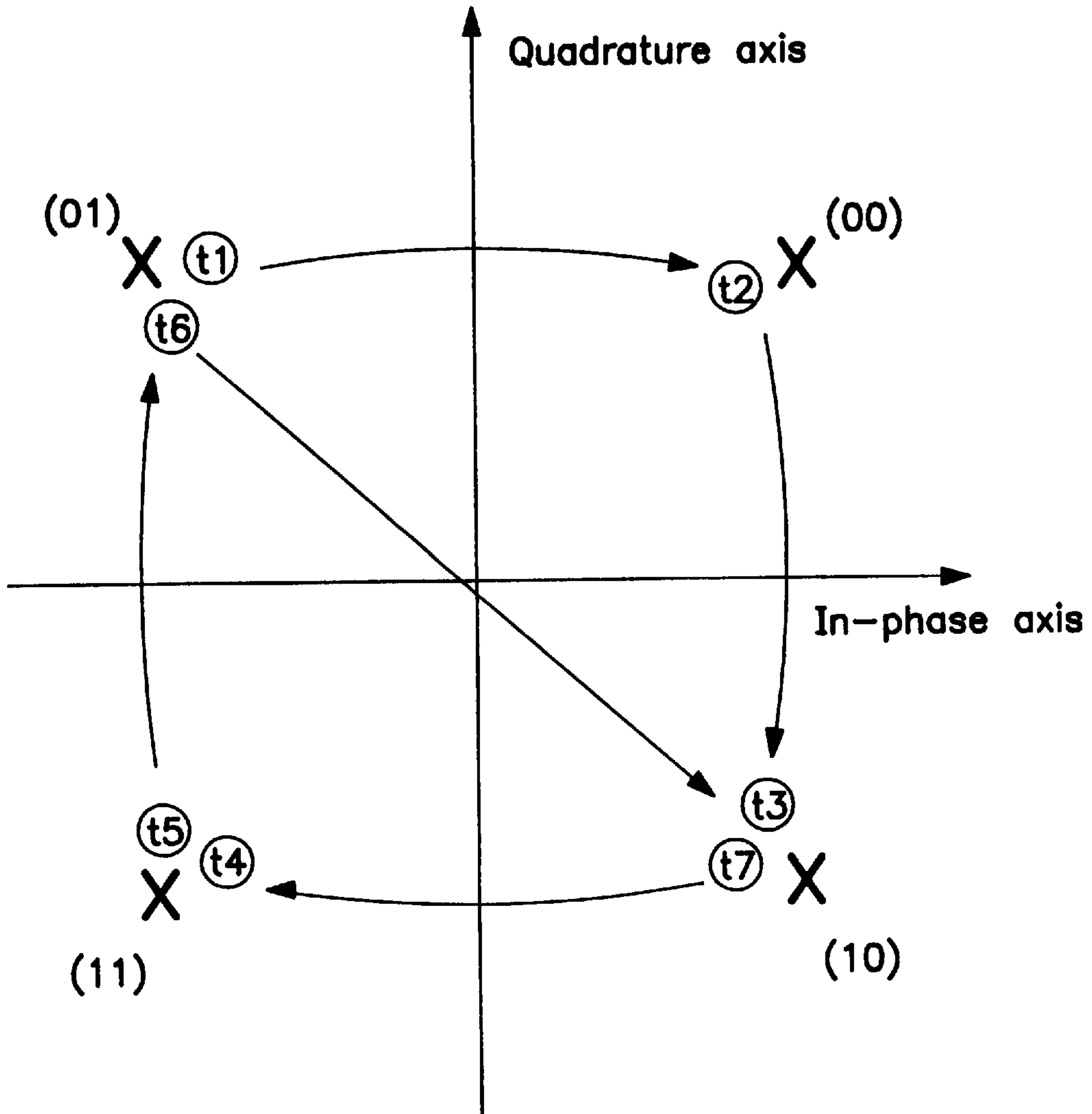
FIG. 6 PRIOR ART
