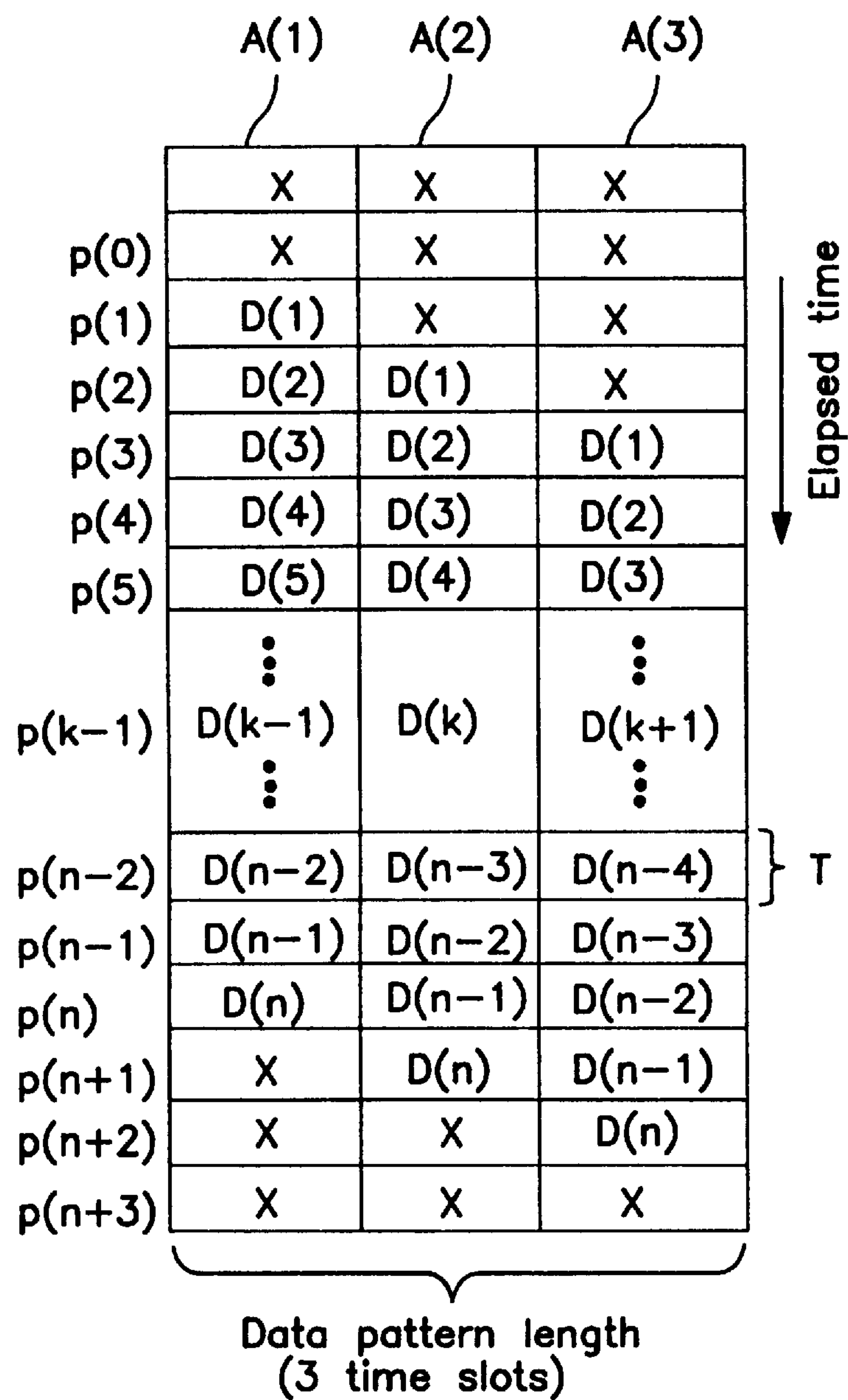
FIG. 3 PRIOR ART
