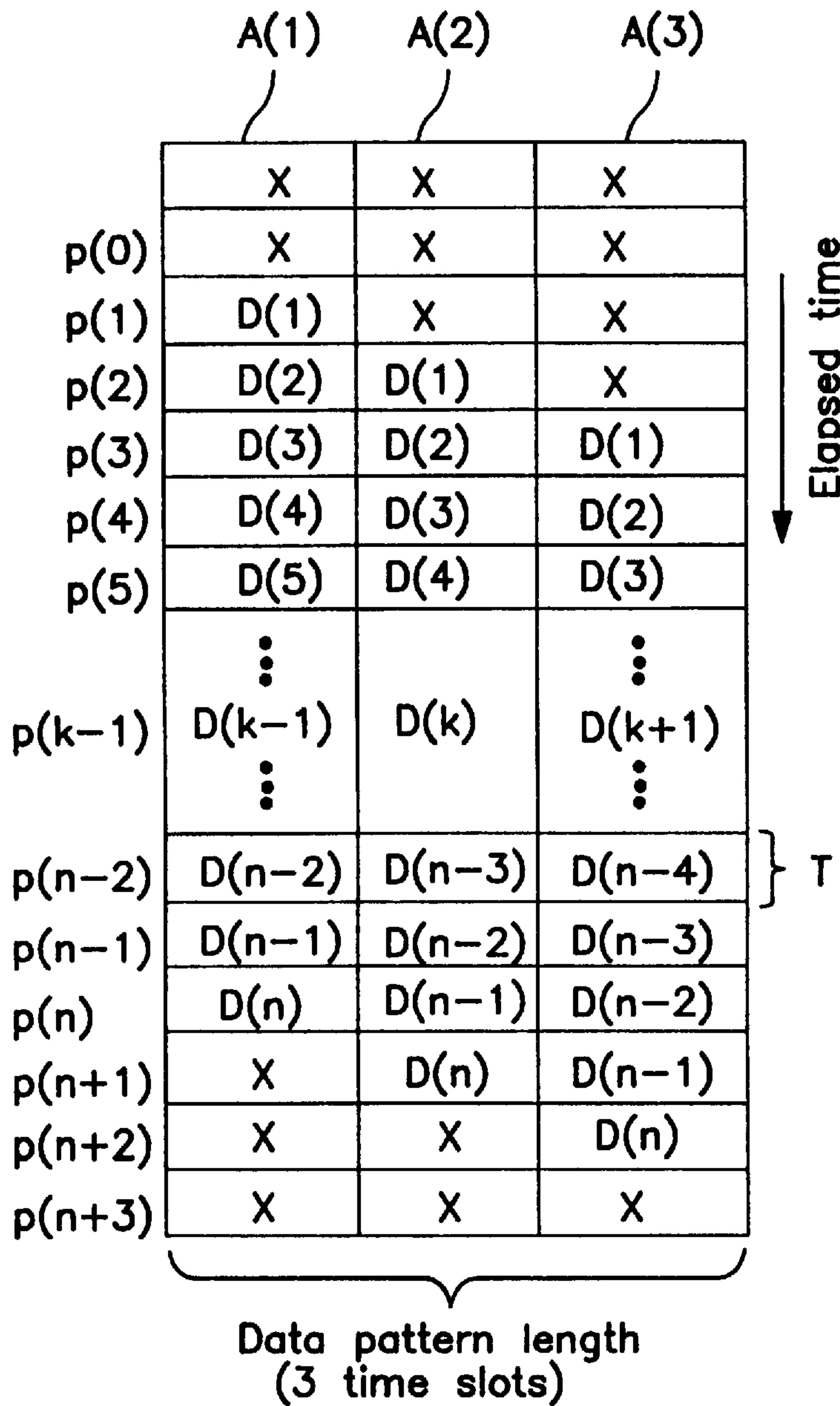
FIG. 3 PRIOR ART
