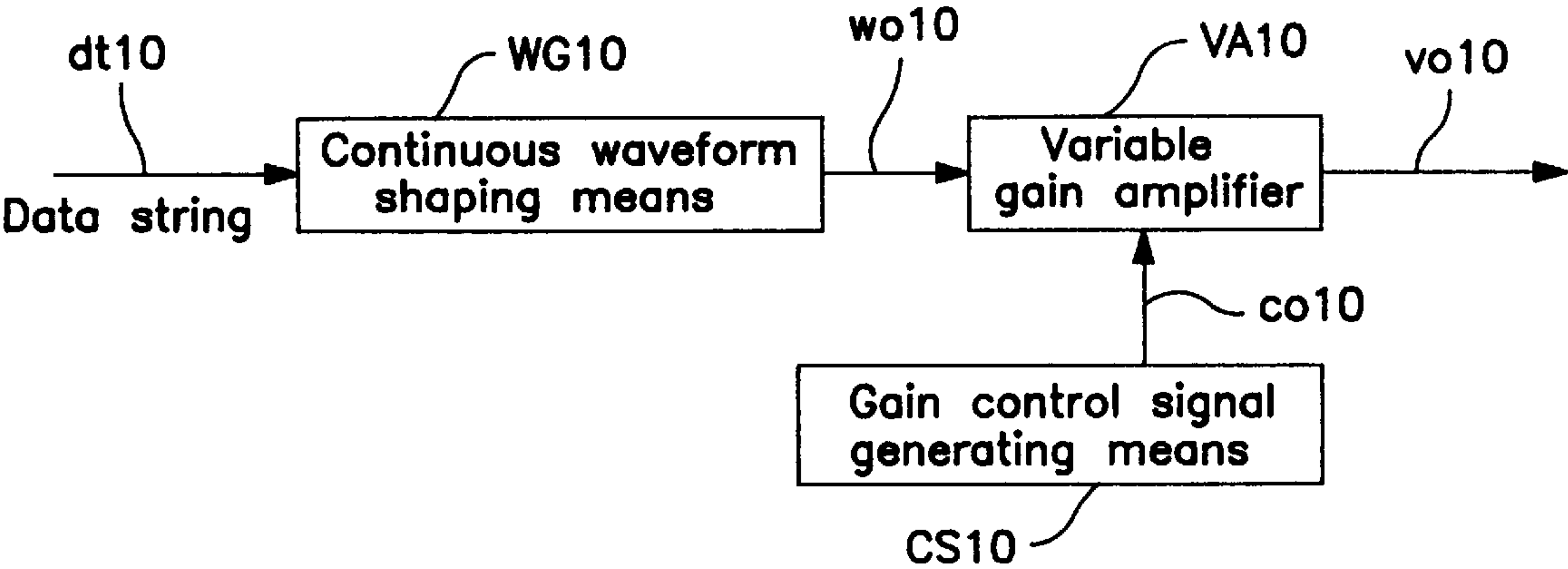
FIG. 11 PRIOR ART
