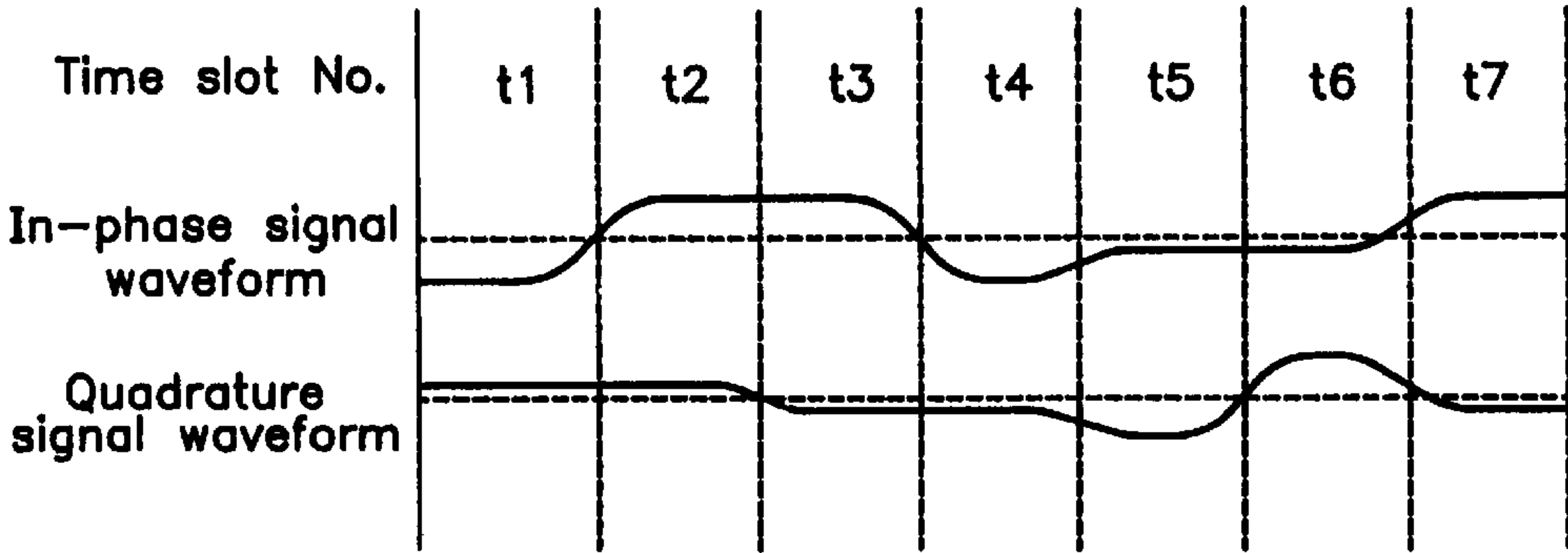
FIG. 9C PRIOR ART
