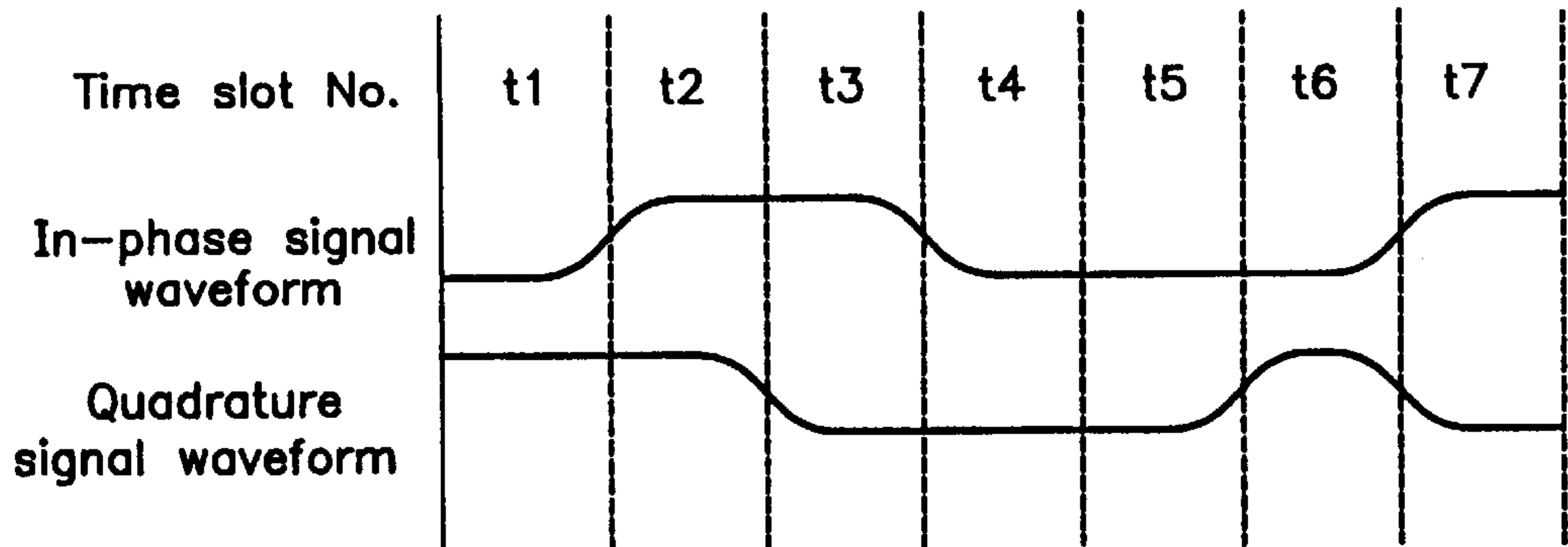
FIG. 5C PRIOR ART
