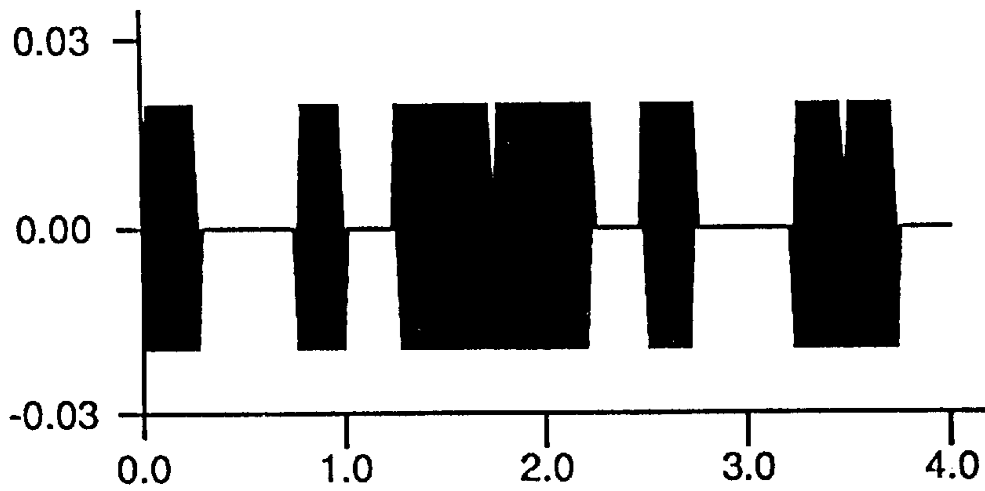
AMPLITUDE ON-OFF PLUS BIPHASE CARRIER MODULATION
