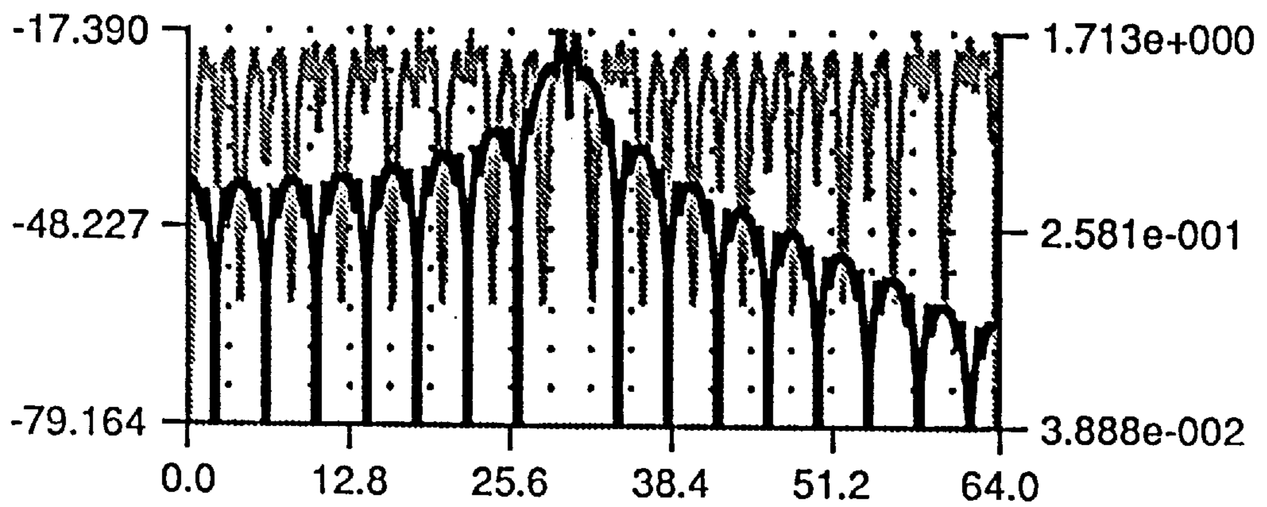
BIPHASE CARRIER MODULATION SPECTRUM
