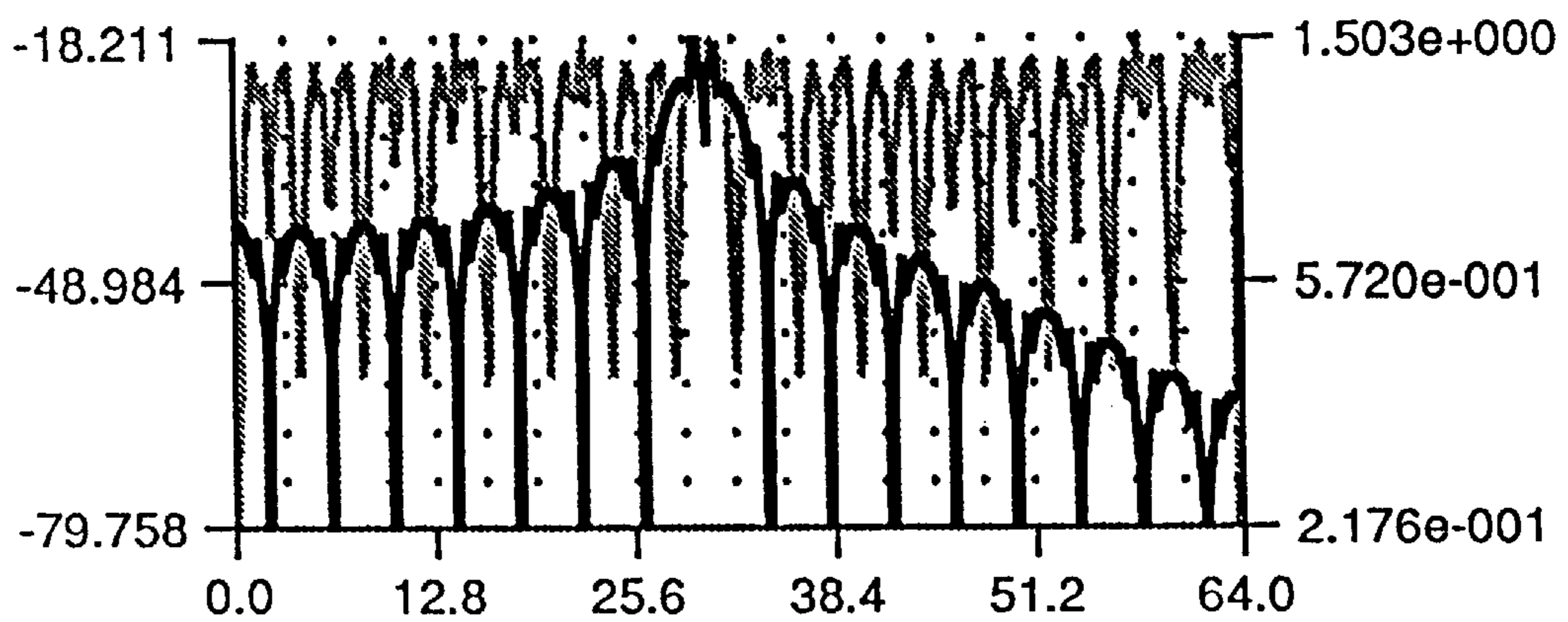
AMPLITUDE ON-OFF PLUS BIPHASE CARRIER MODULATION SPECTRUM
