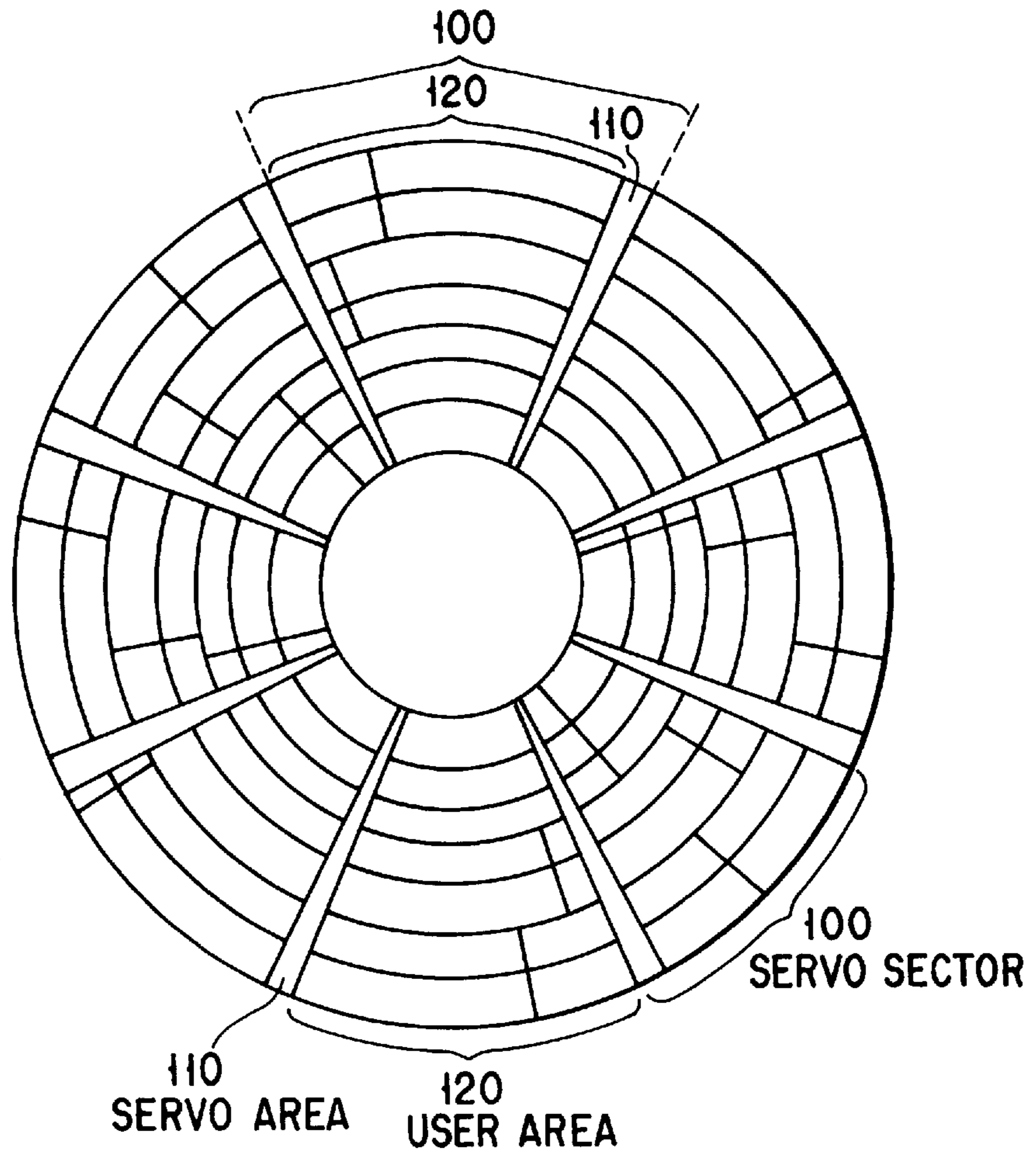
FIG. 1 (PRIOR ART)
