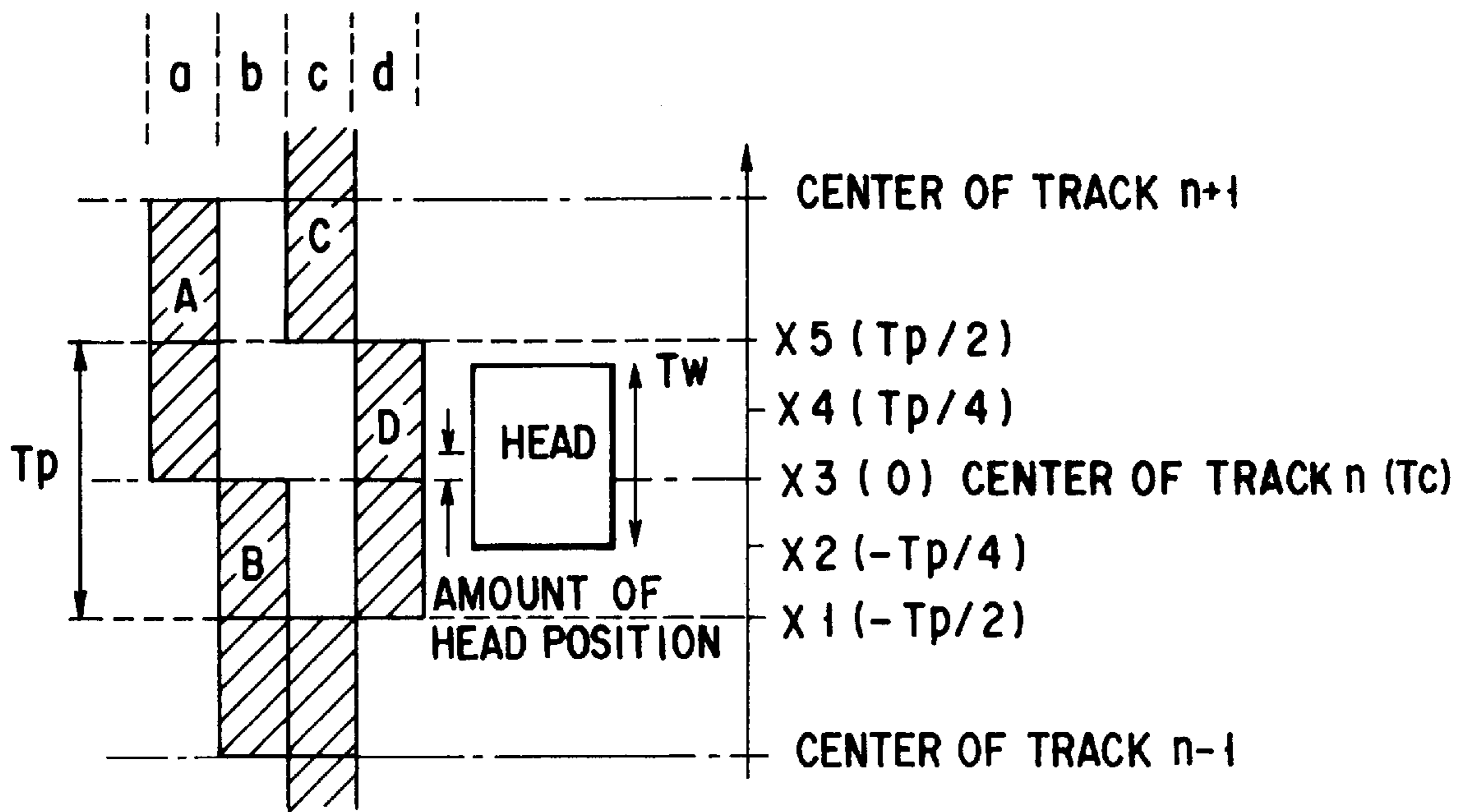
FIG. 3 (PRIOR ART)
