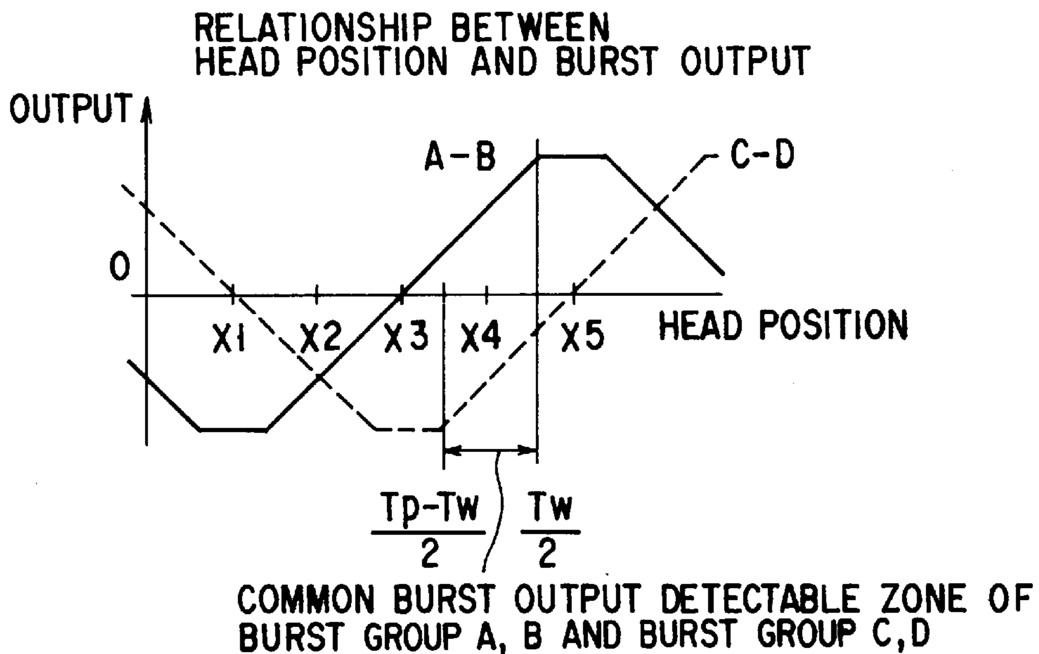
FIG. 4 (PRIOR ART)
