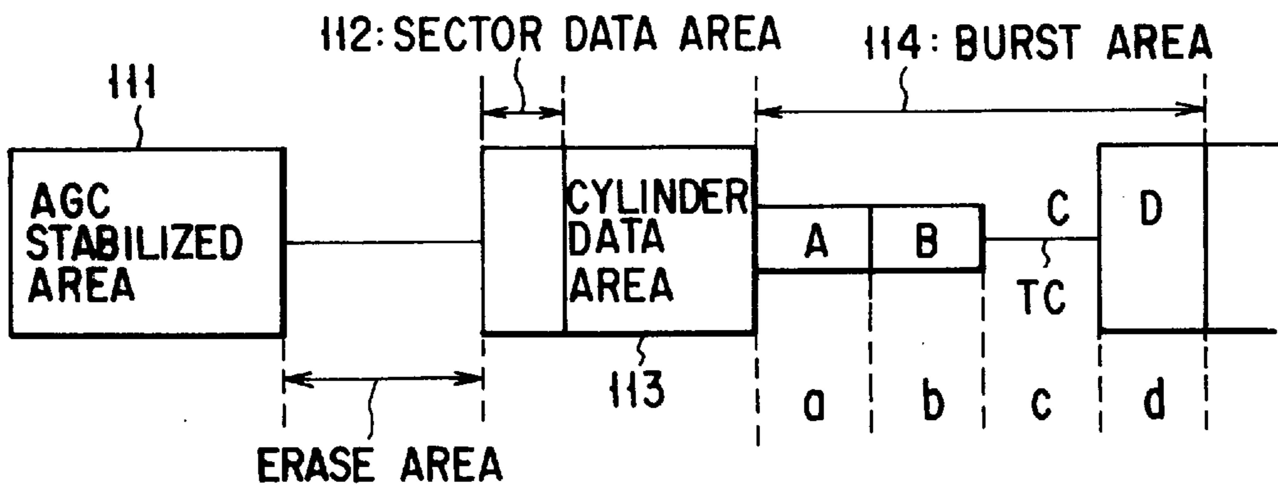
FIG. 2 (PRIOR ART)
