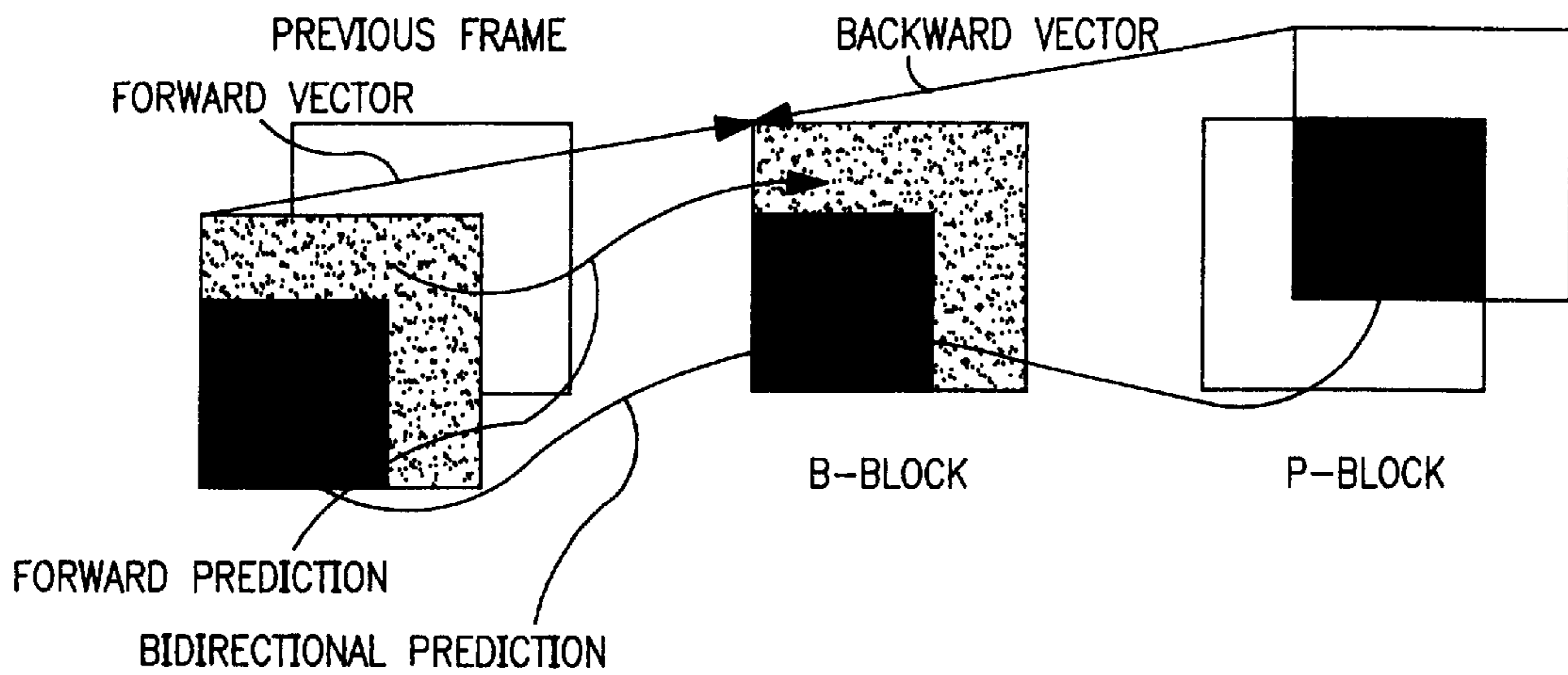
B-BLOCK PREDICTION
