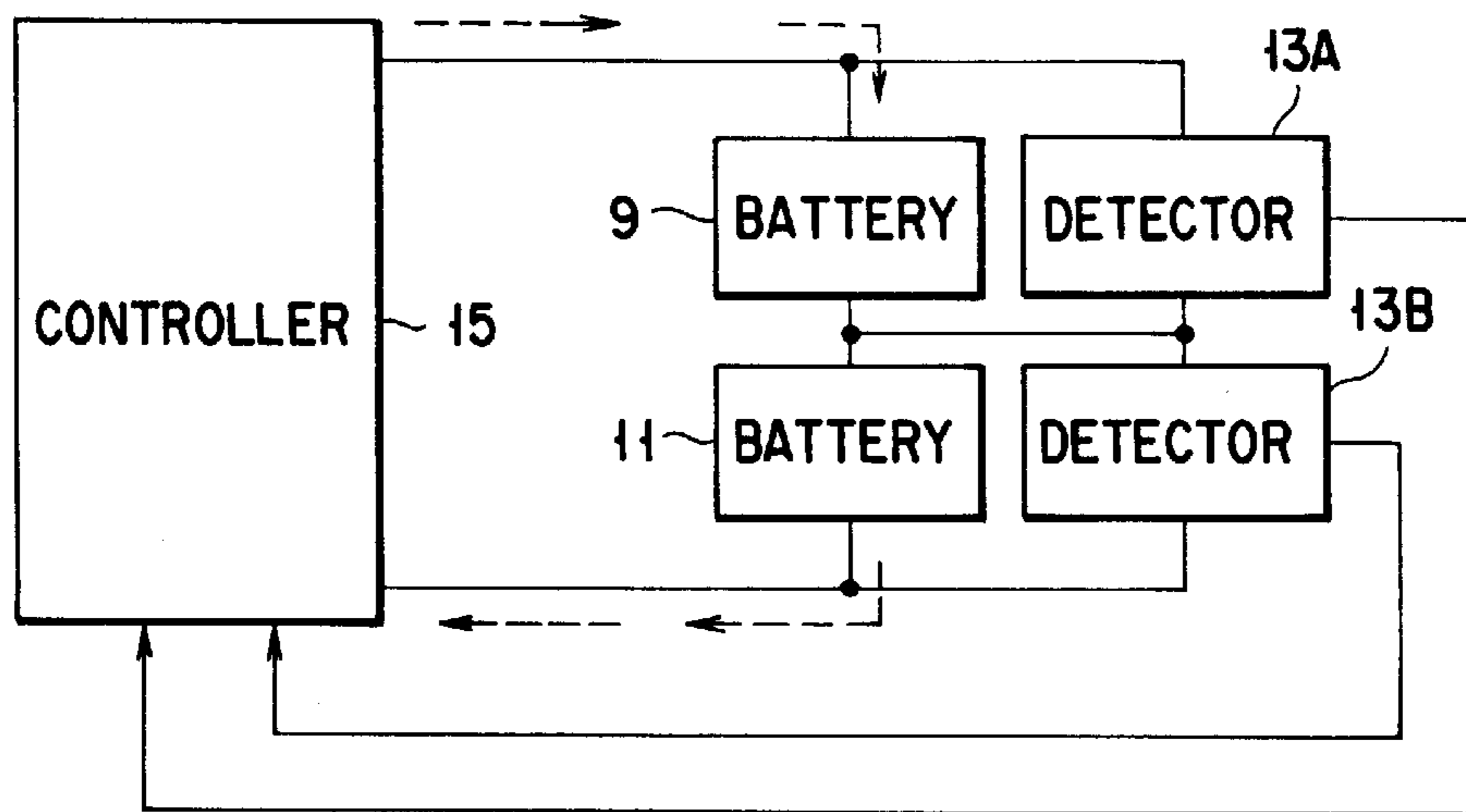
FIG. 84 (PRIOR ART)
