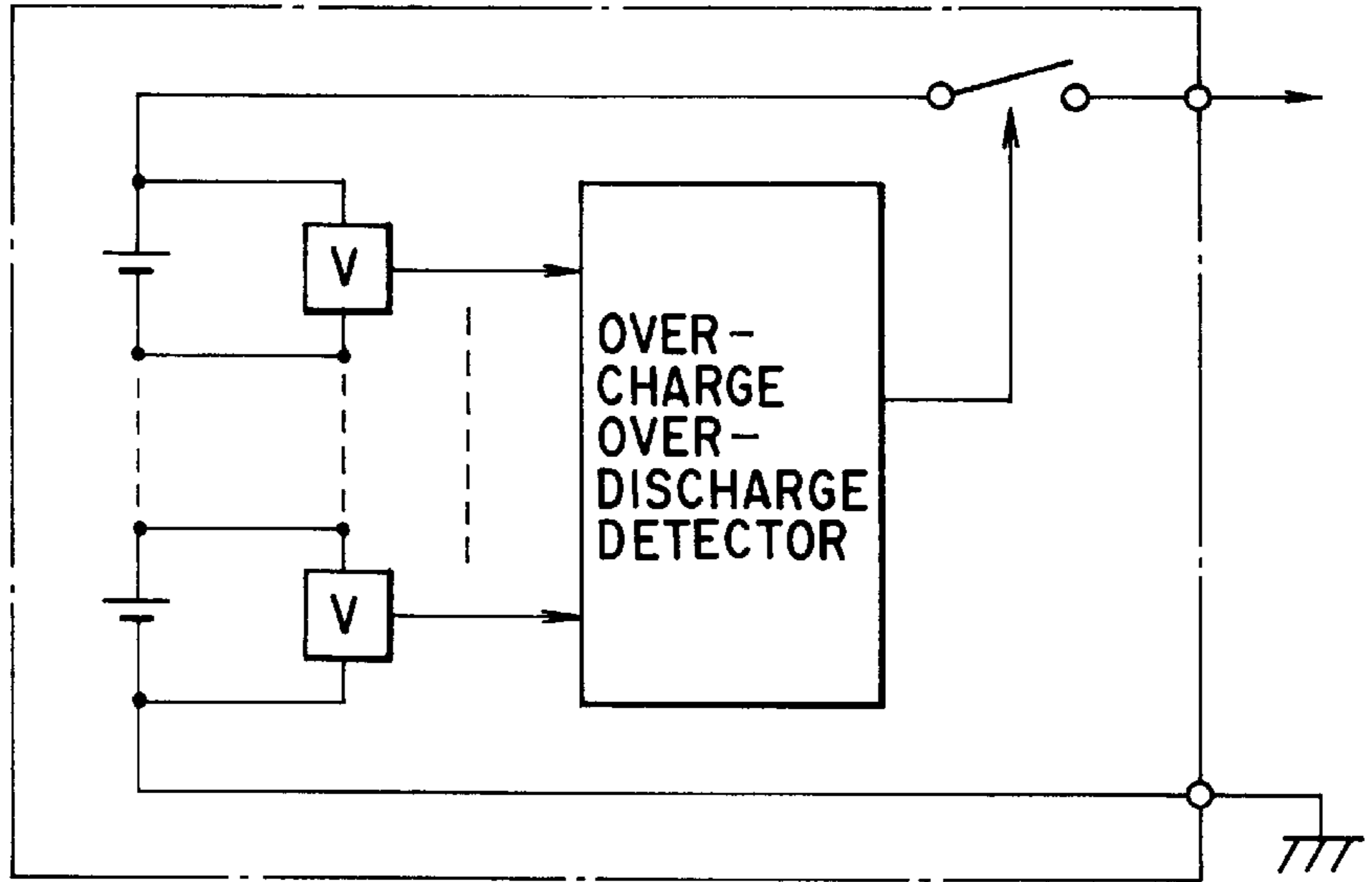
FIG. 30 (PRIOR ART)
