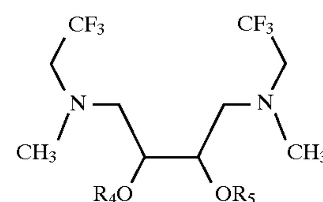
General Precursor for Compound D-1
