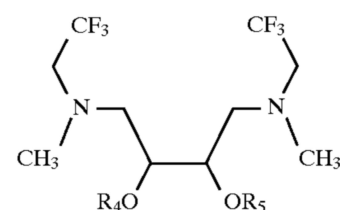
General Precursor for Compound D-1
