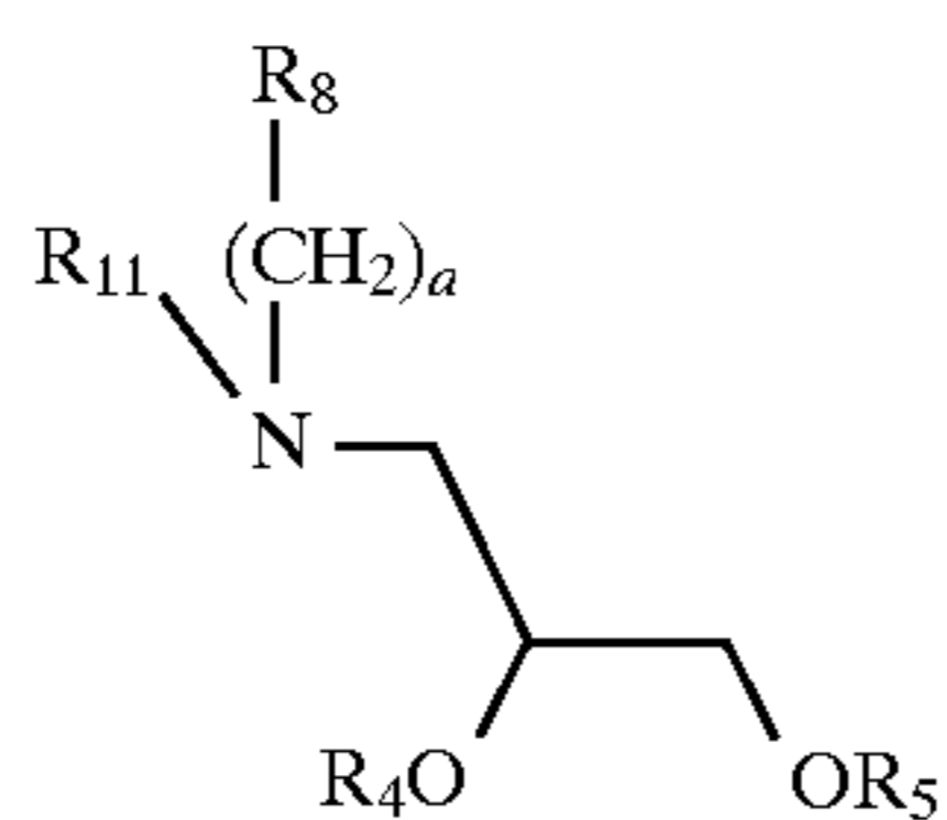
General Precursor for Compound C-1
