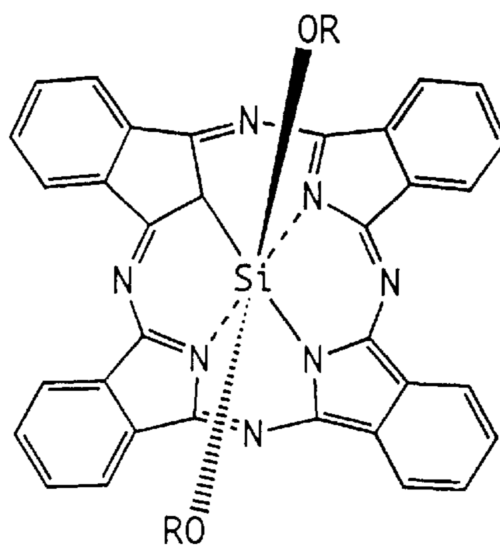
SILICON PHTHALOCYANINE
