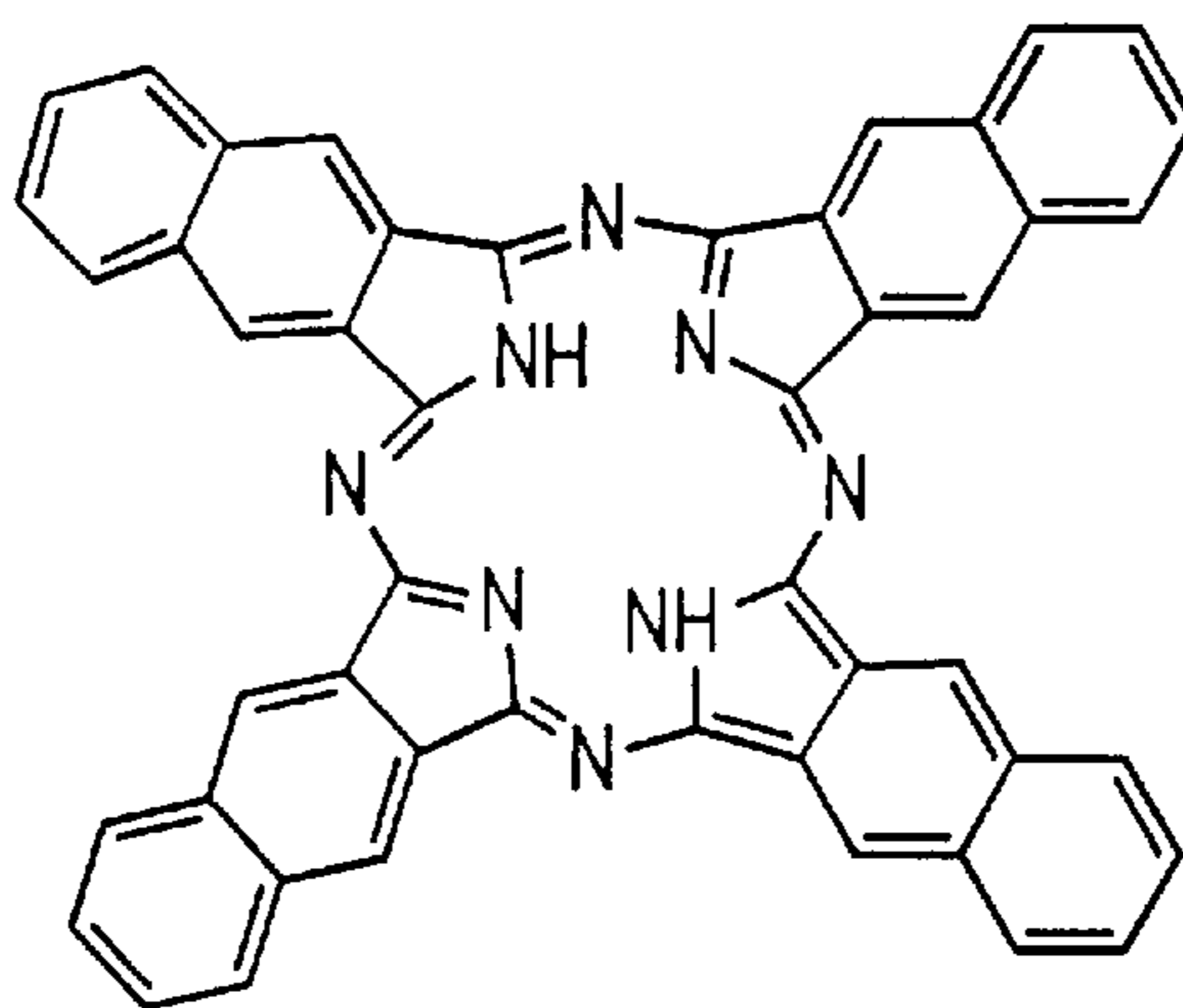
NAPHTHALOCYANINE
