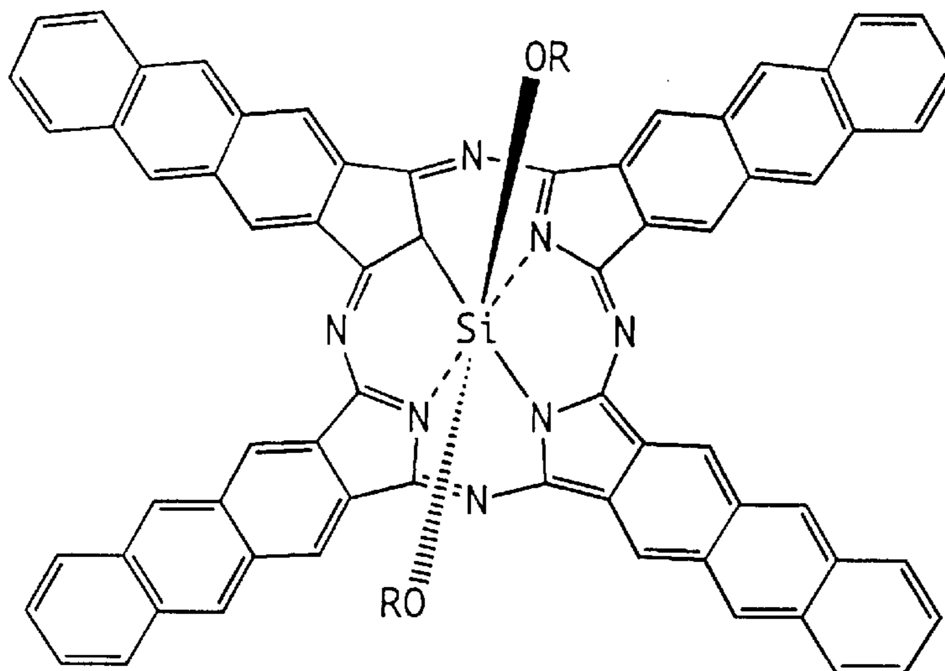
SILICON ANTHRACYANINE
