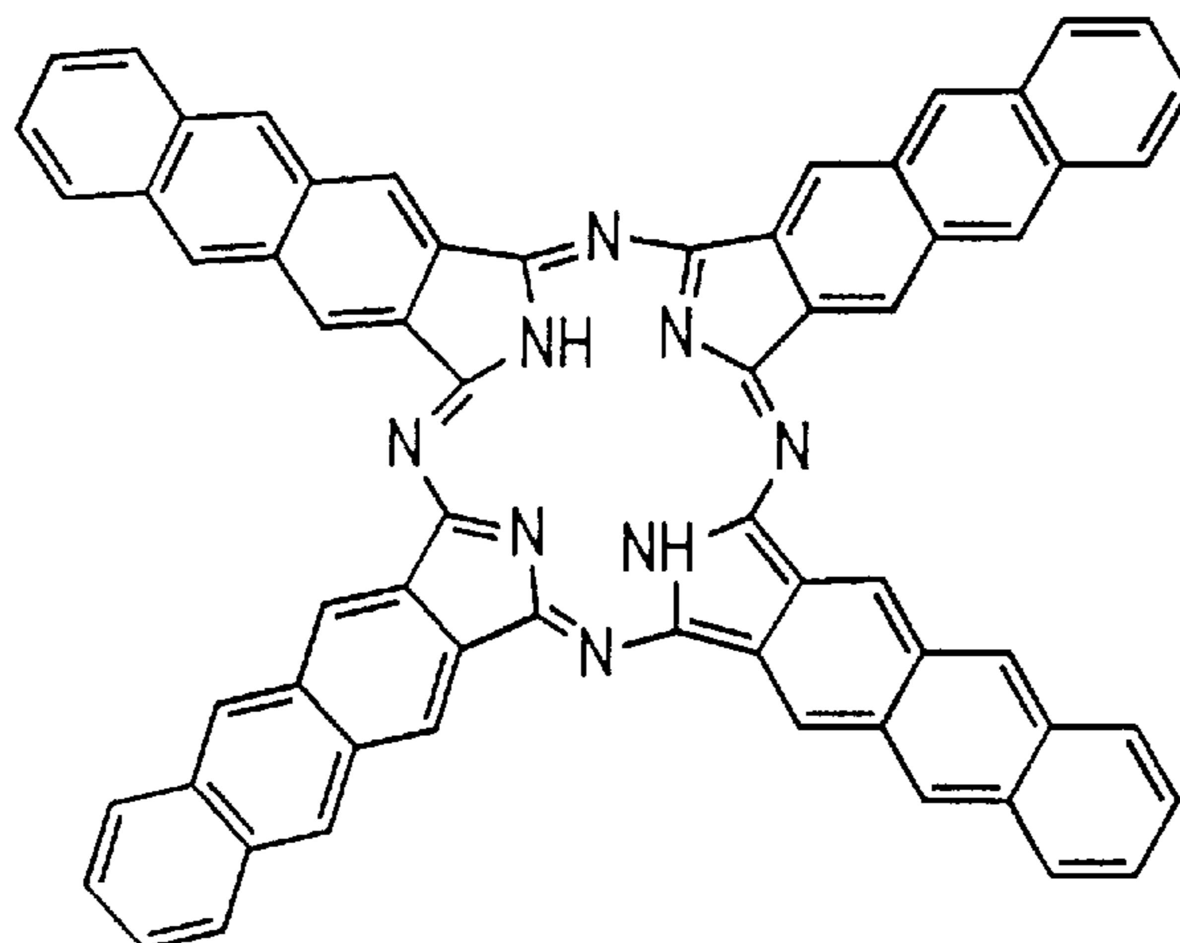
ANTHRANYLOCYANINE
