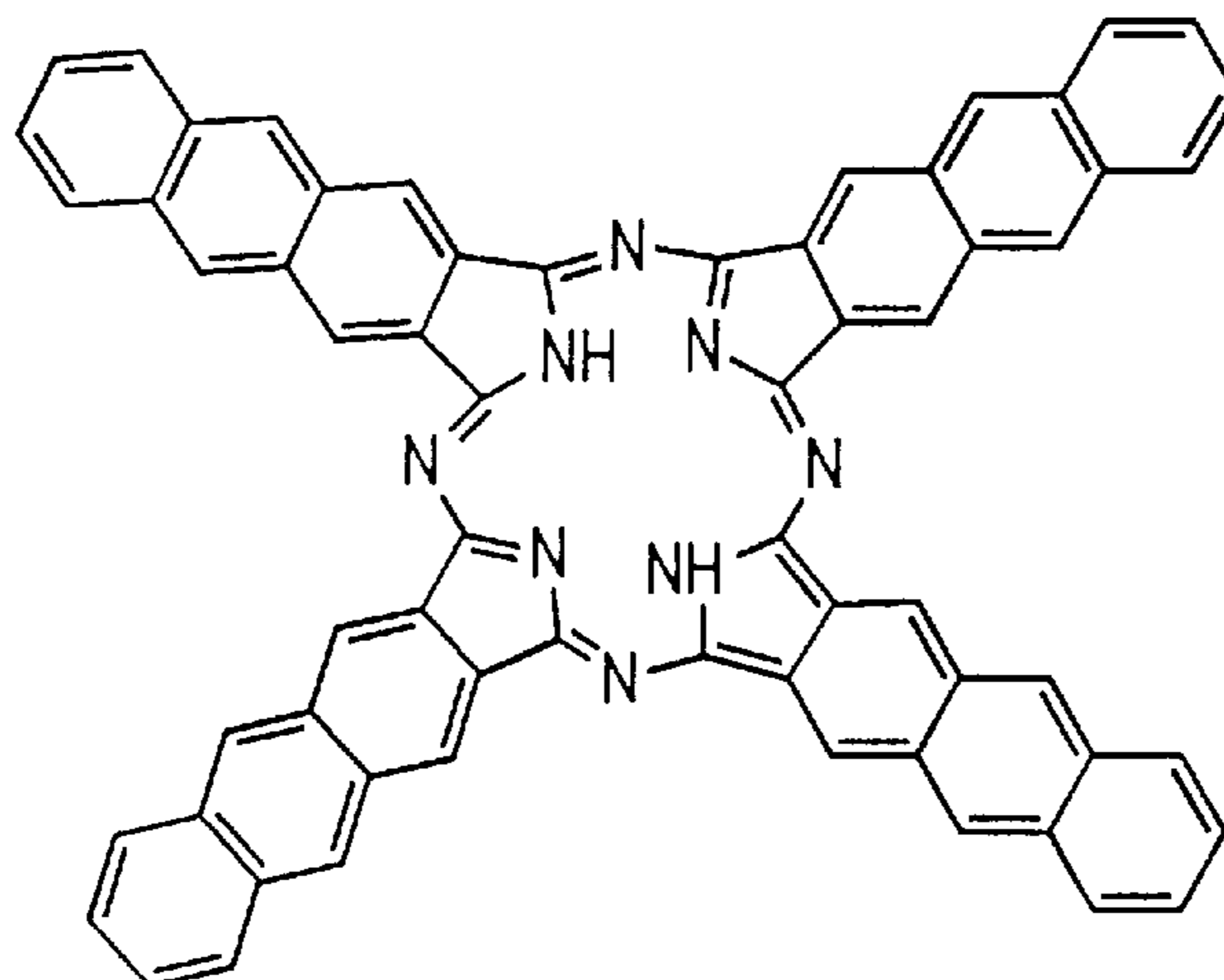
ANTHRANYLOCYANINE
