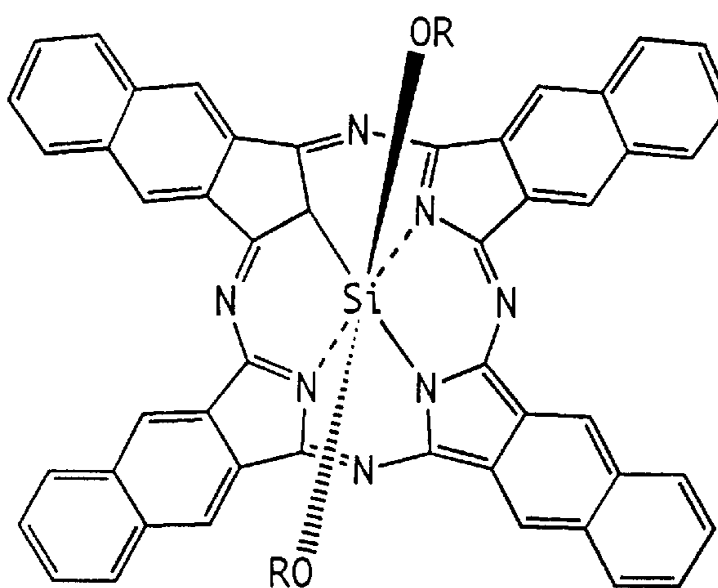
SILICON NAPHTHALOCYANINE
