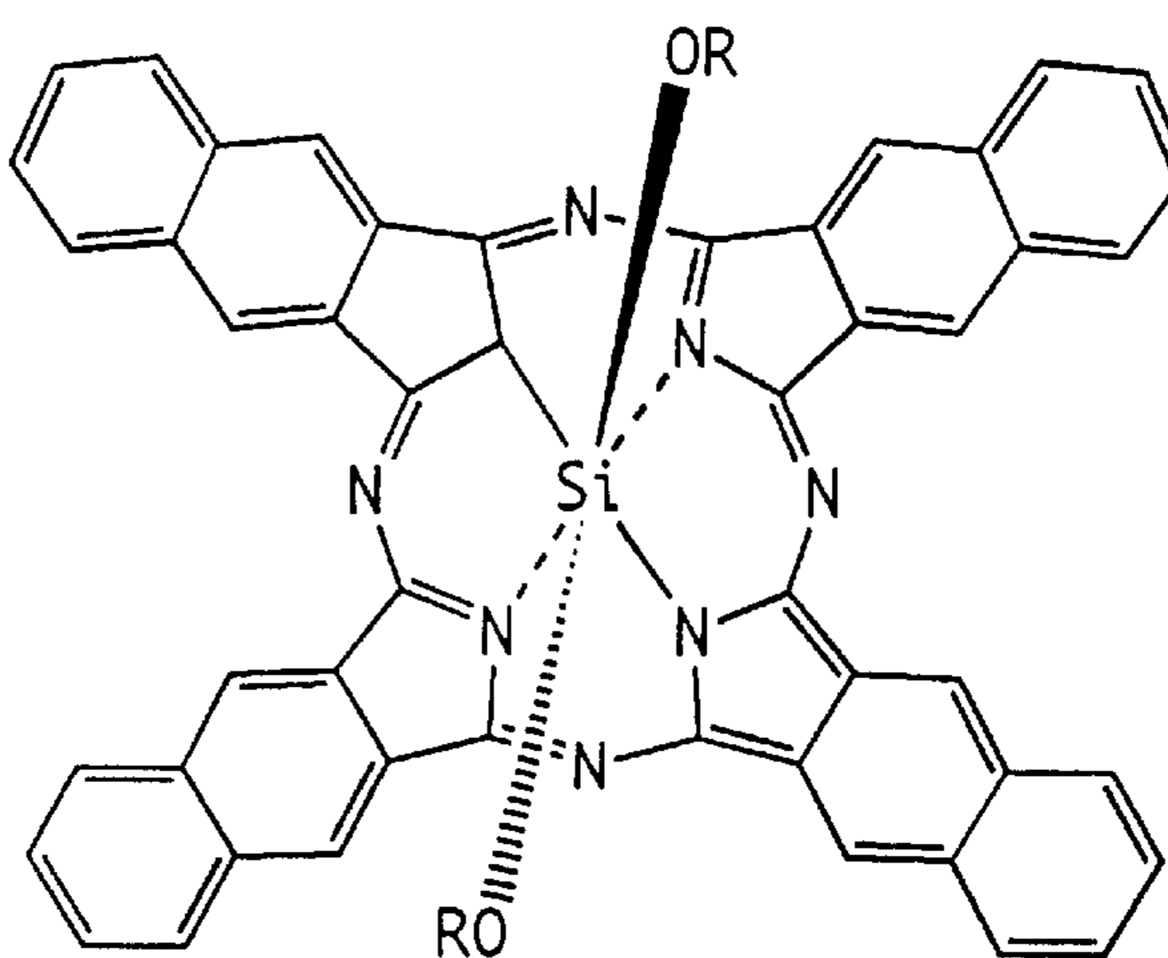
SILICON NAPHTHALOCYANINE
