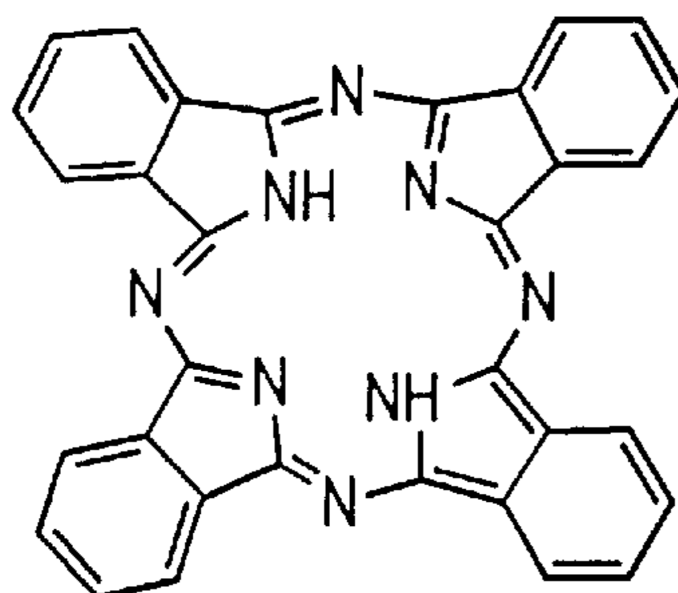
PHTHALOCYANINE
