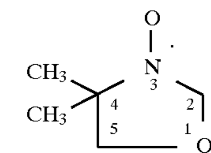
DOXYL (4,4-Dimethyl-3-oxazolinyloxy-) (4,4-Dimethyloxazolidine-N-oxyloxy)
