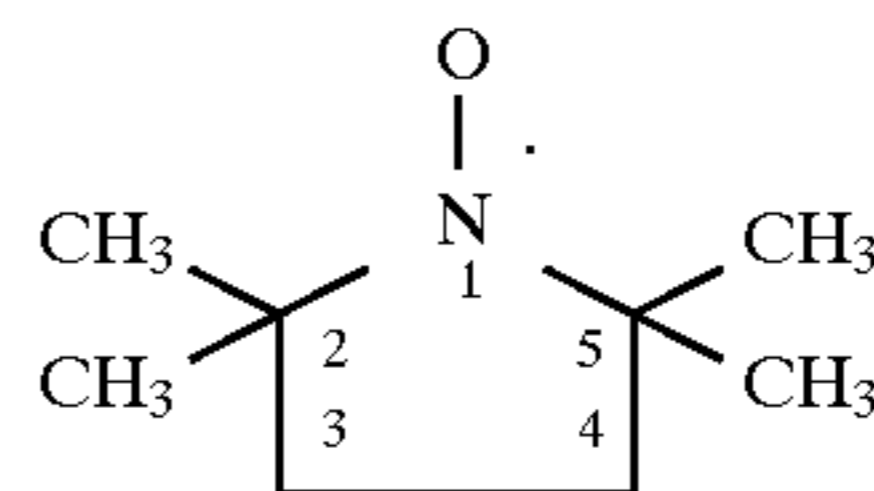
PROXYL (2,2,5,5-Tetramethyl-1-pyrrolidinyl-) (2,2,5,5-Tetramethylpyrrolidine-N-oxyloxy)
