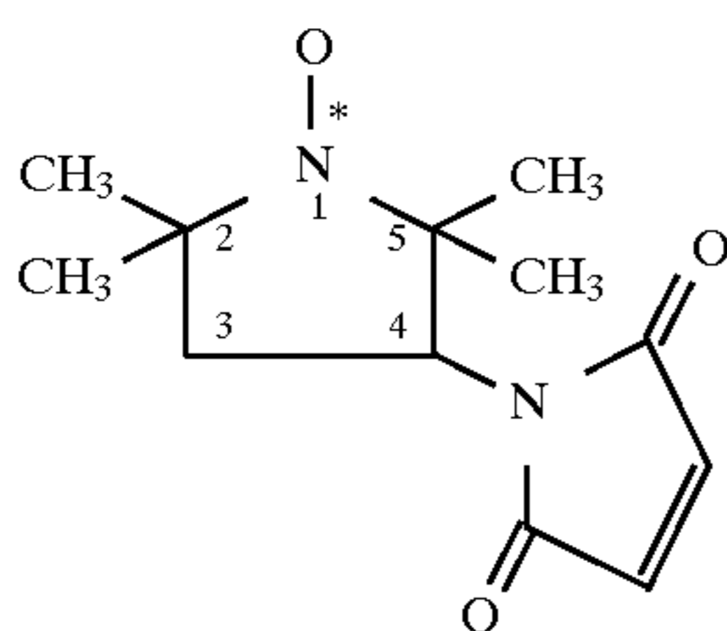
3-Maleimido-PROXYL
