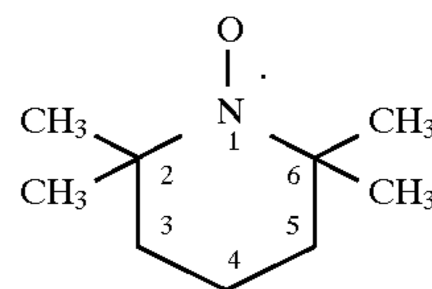
TEMPO (2,2,6,6-Tetramethyl-1-piperidinyl-) (2,2,6,6-Tetramethylpiperidine-N-oxyloxy)
