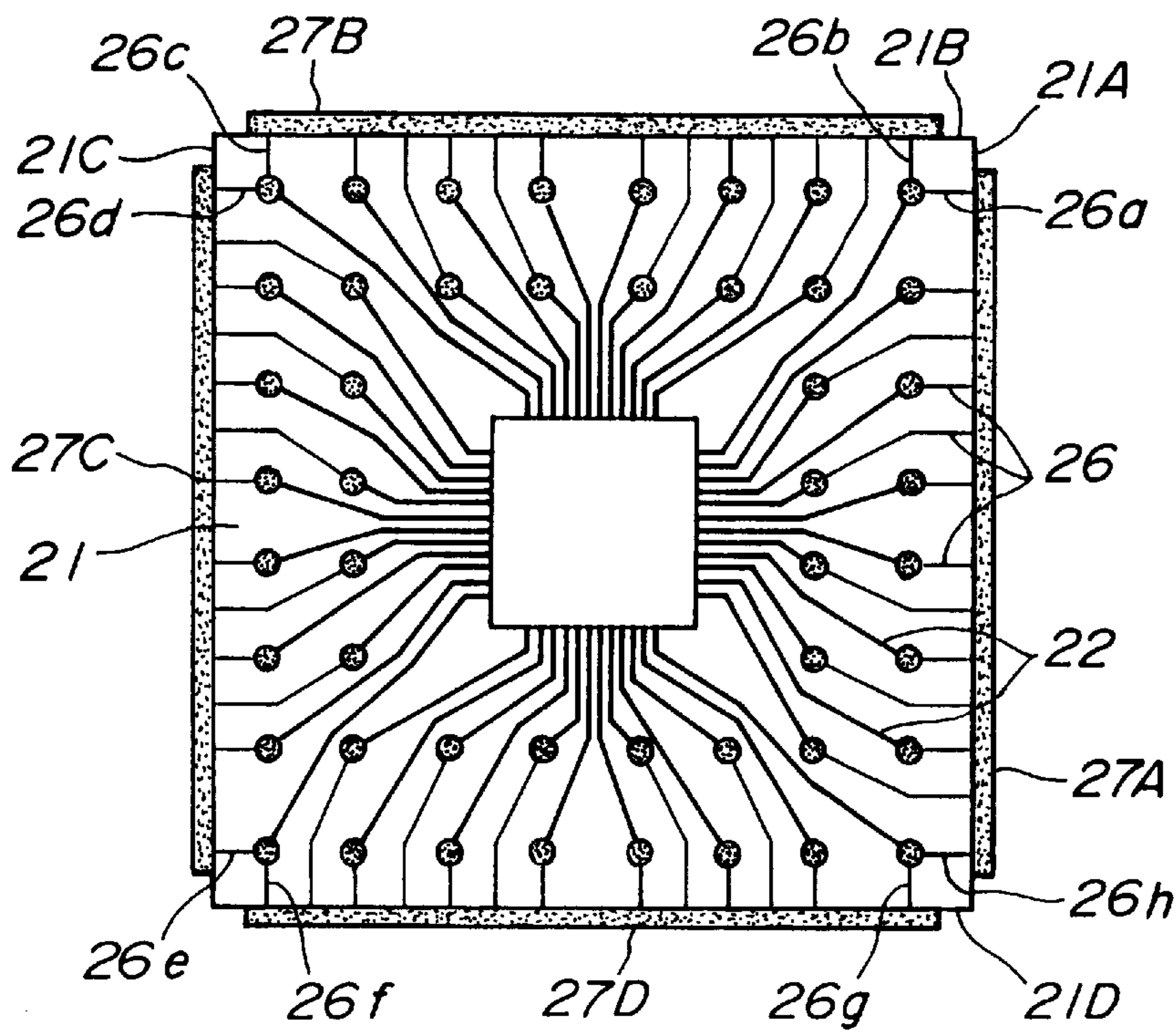
FIG. 8 PRIOR ART
