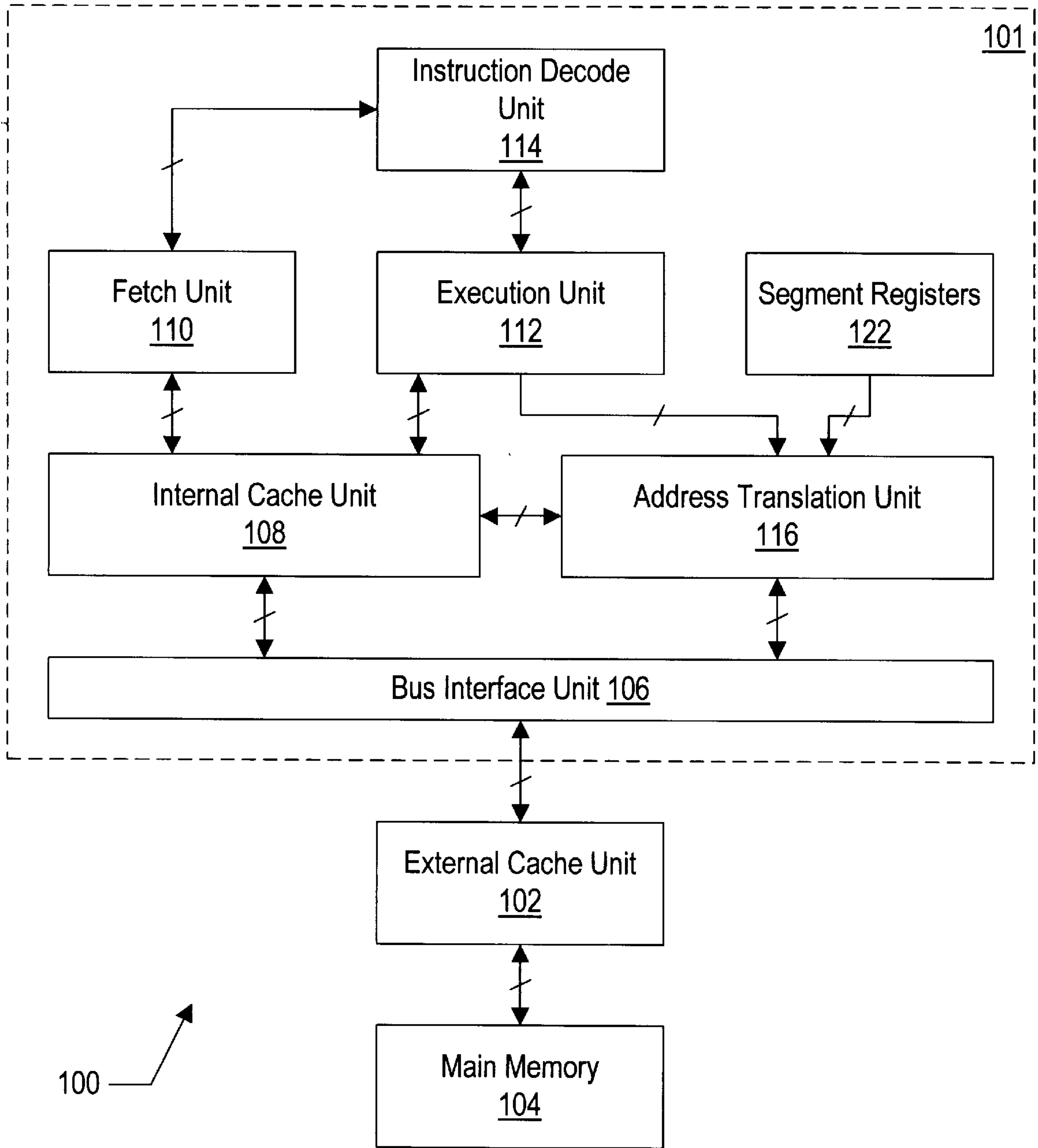
FIG. 1 (PRIOR ART)
