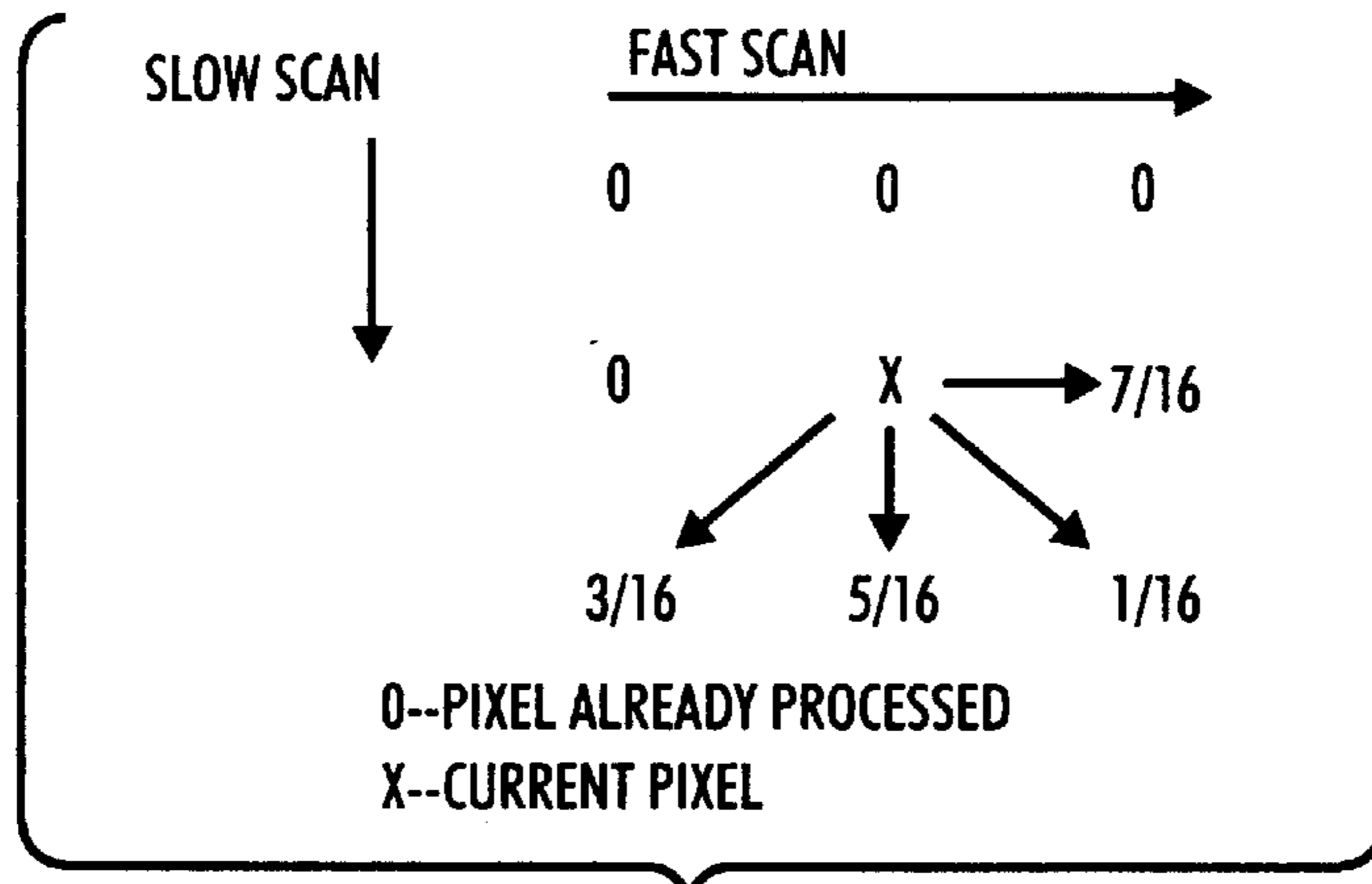
FIG. 23 (PRIOR ART)
