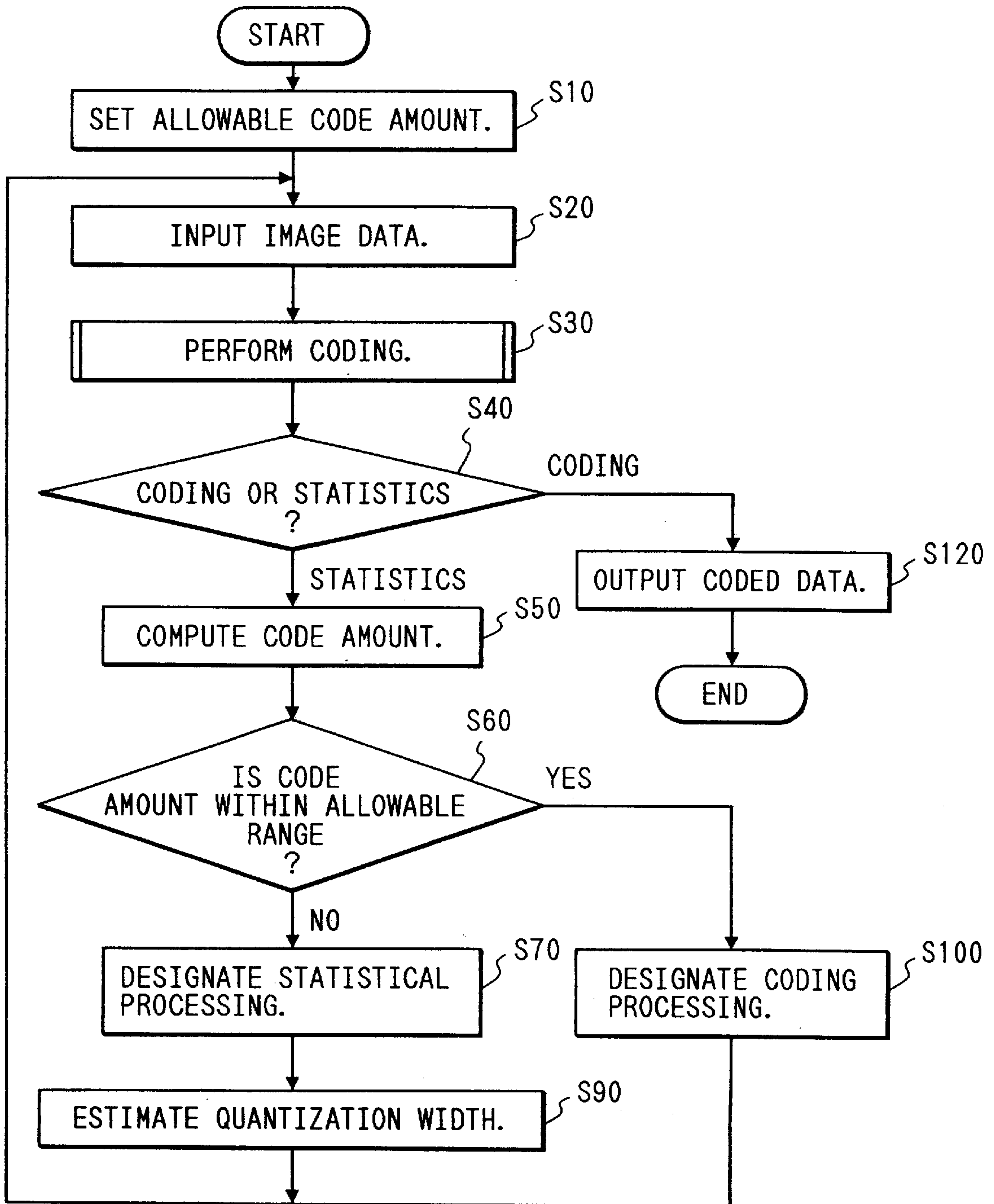
FIG. 13 PRIOR ART
