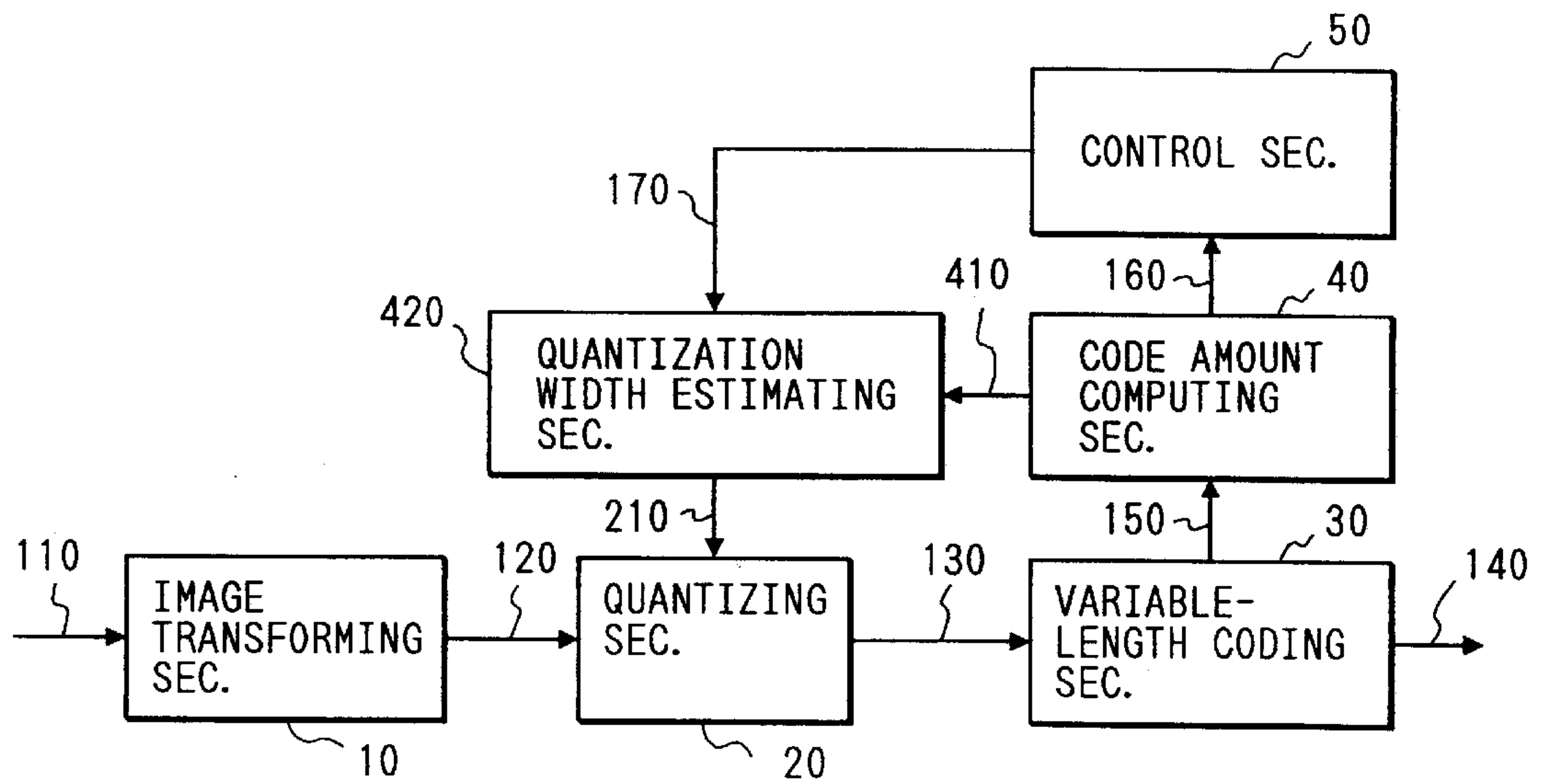
FIG. 12 PRIOR ART
