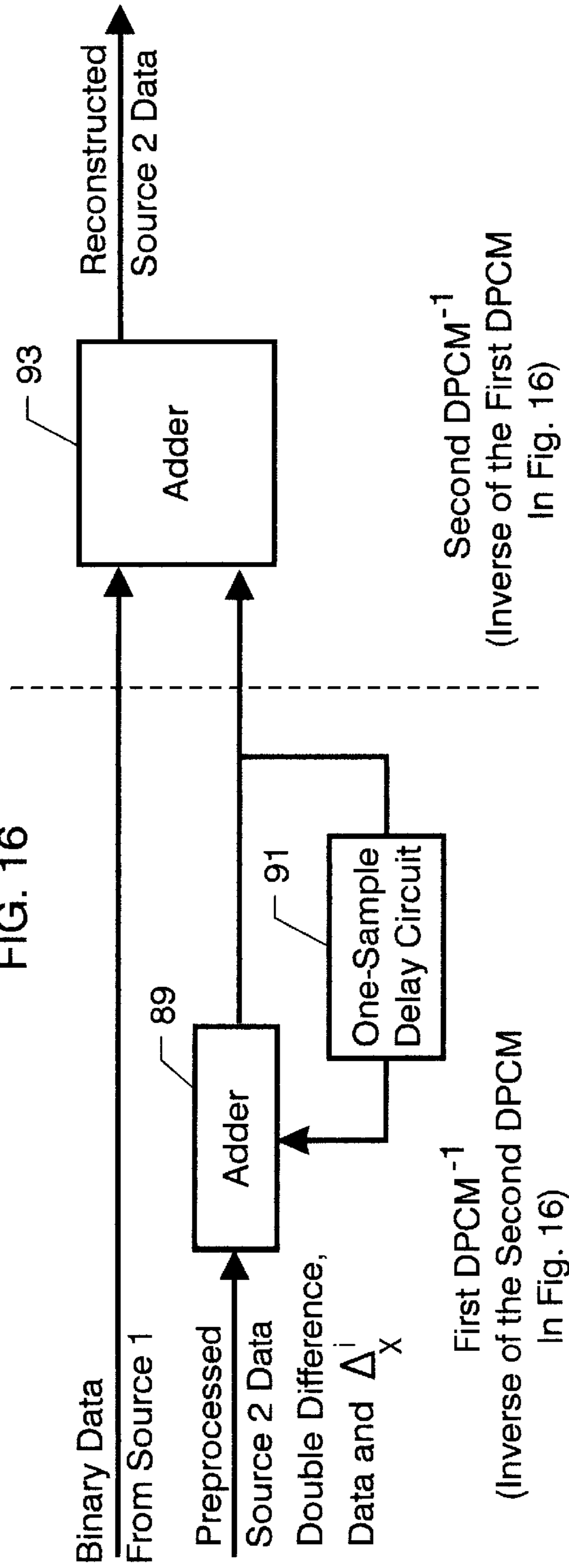
Preferred hardware embodiment for the two inverse DPCM blocks in the data reconstruction operator
