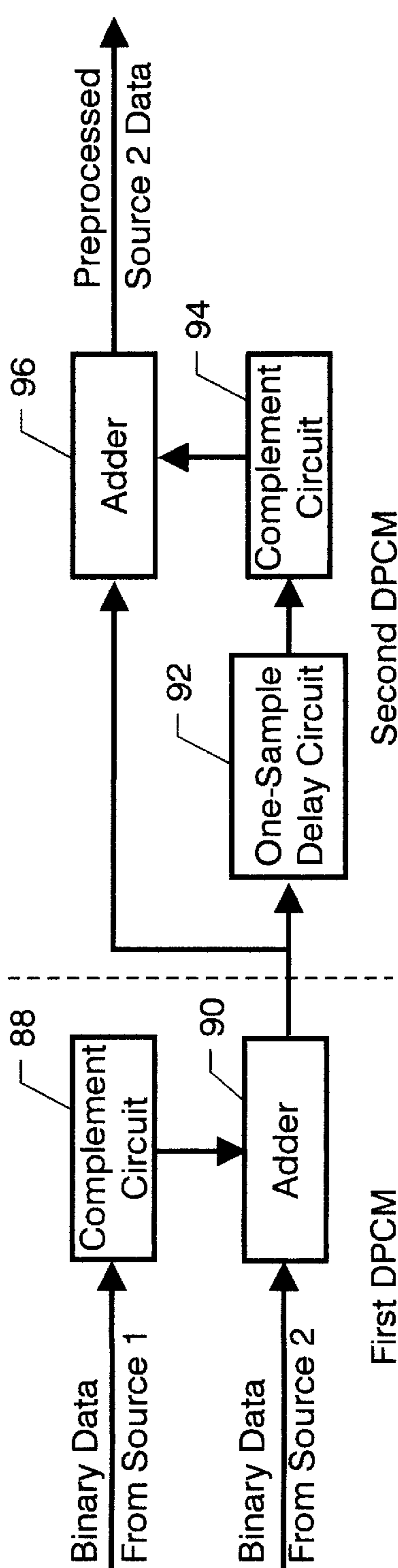
Preferred hardware embodiment for the two DPCM blocks
