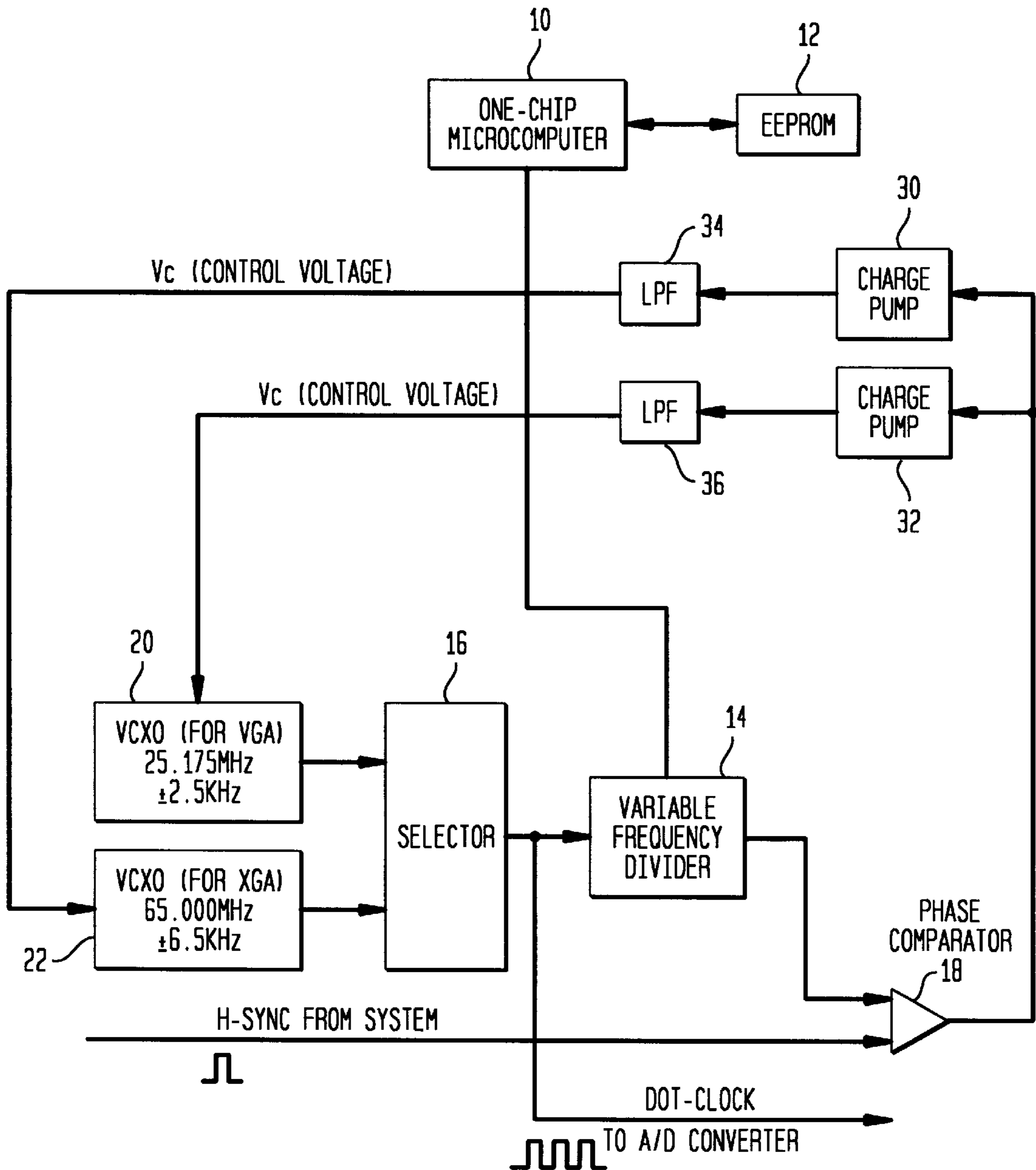
FIG. 6 (PRIOR ART)
