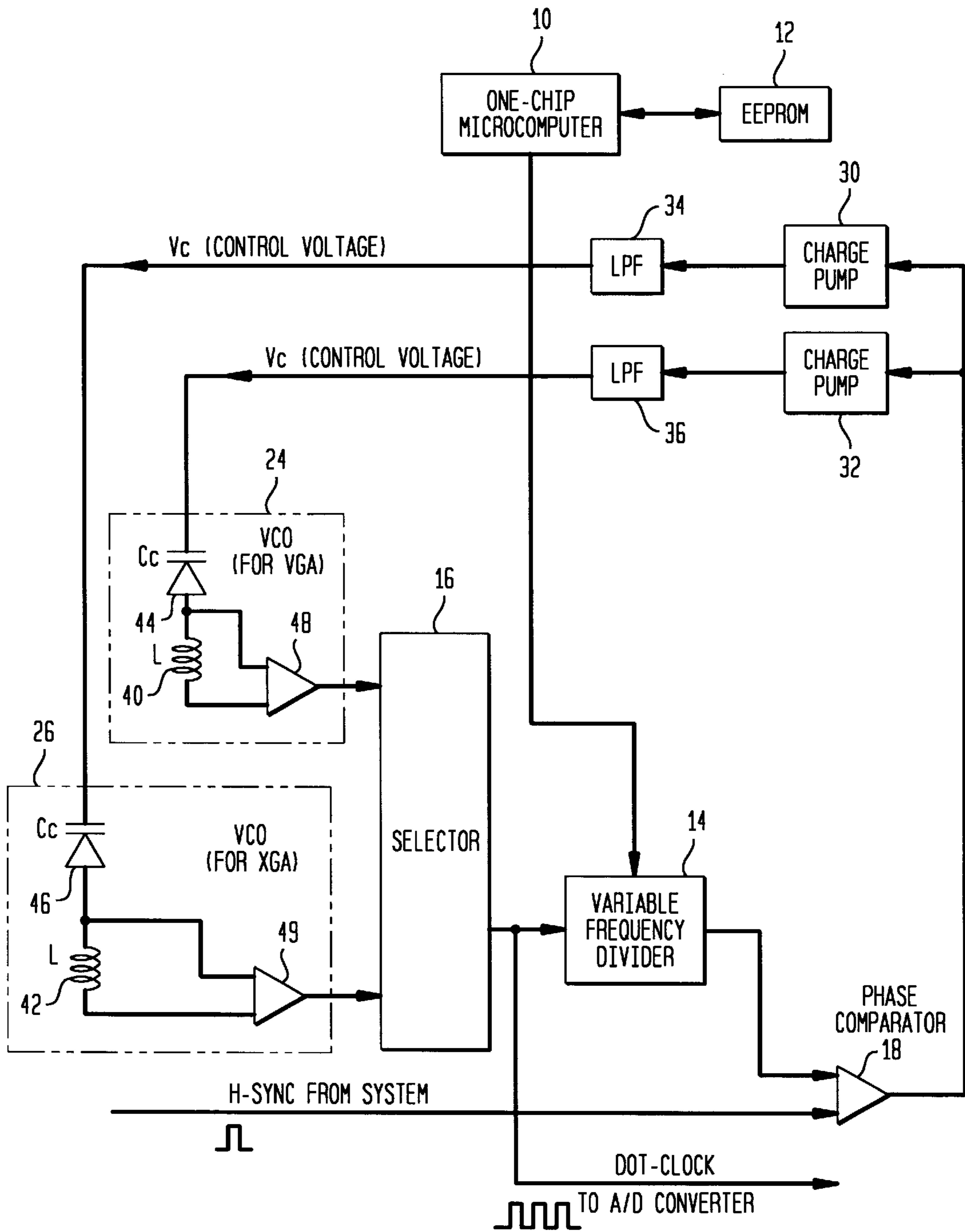
FIG. 7 (PRIOR ART)
