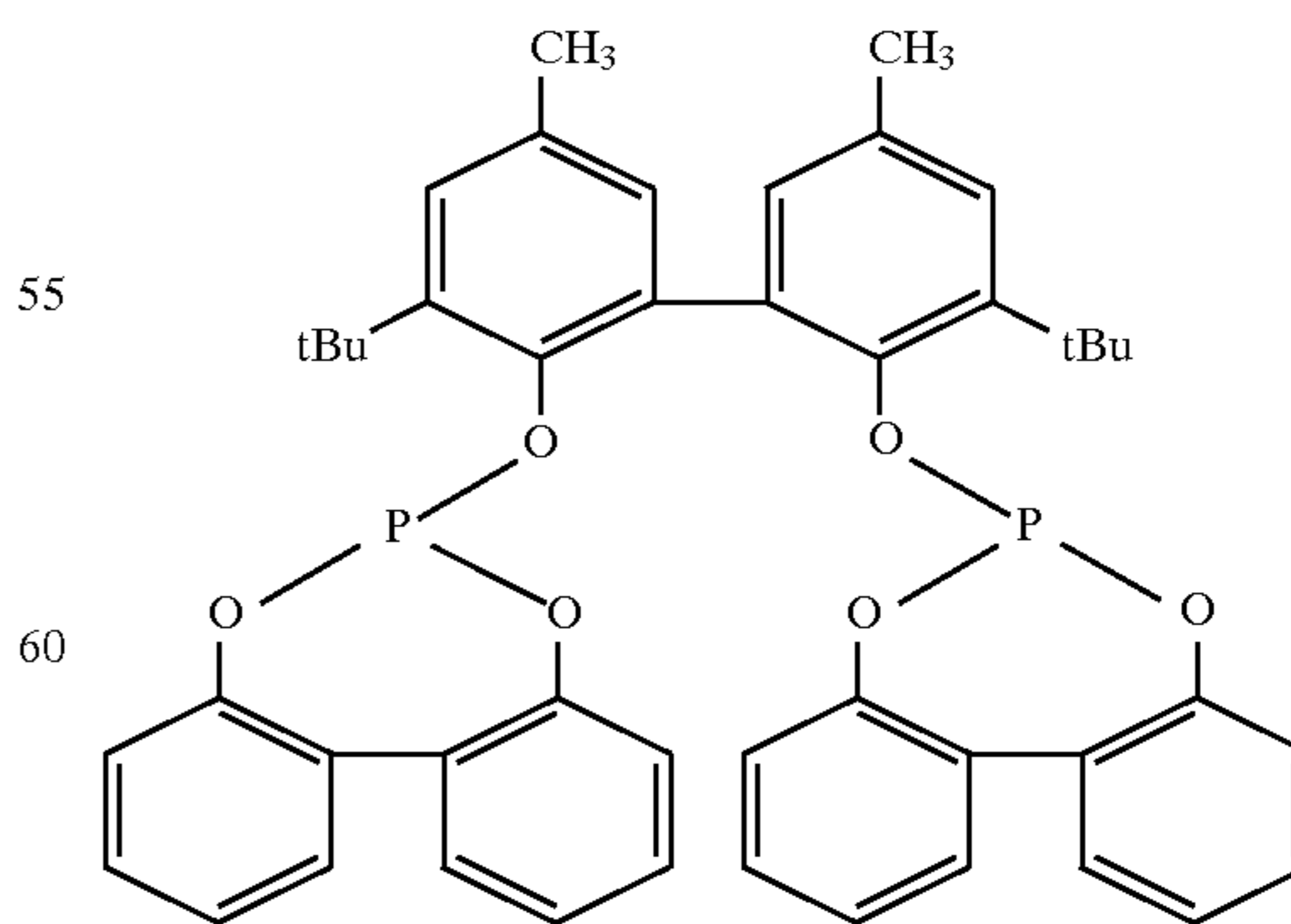
Ligand X
