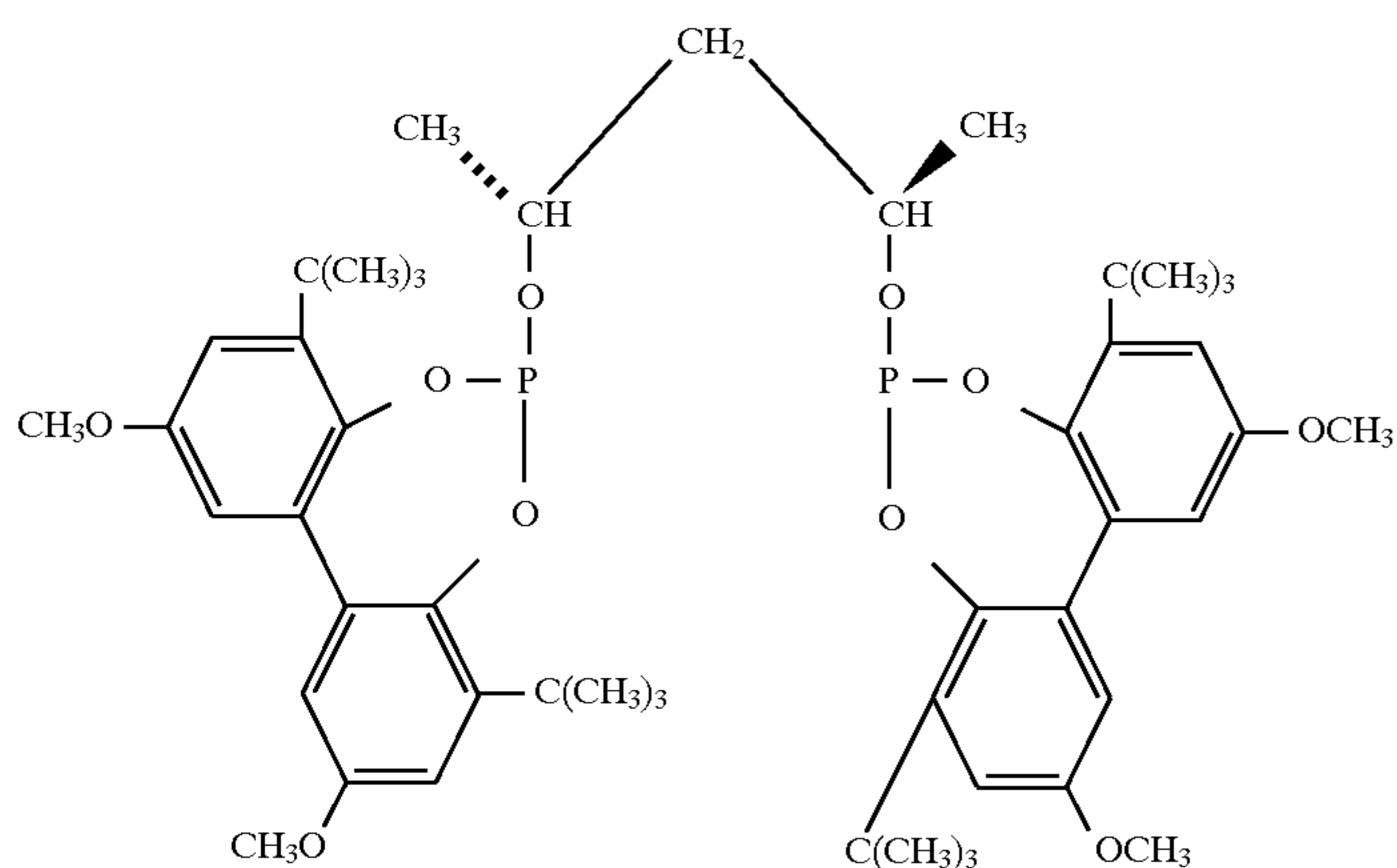
Ligand M
