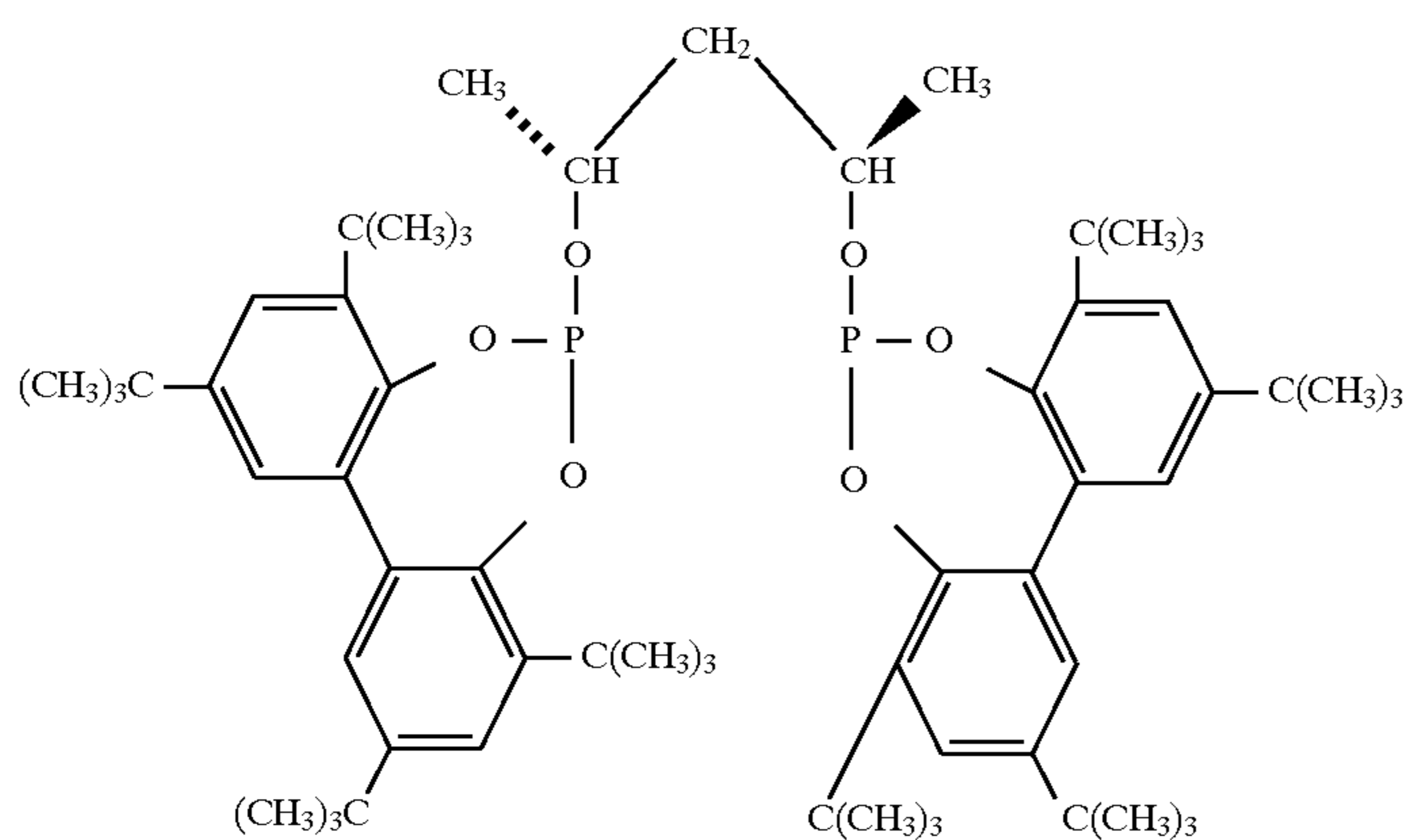
Ligand H
