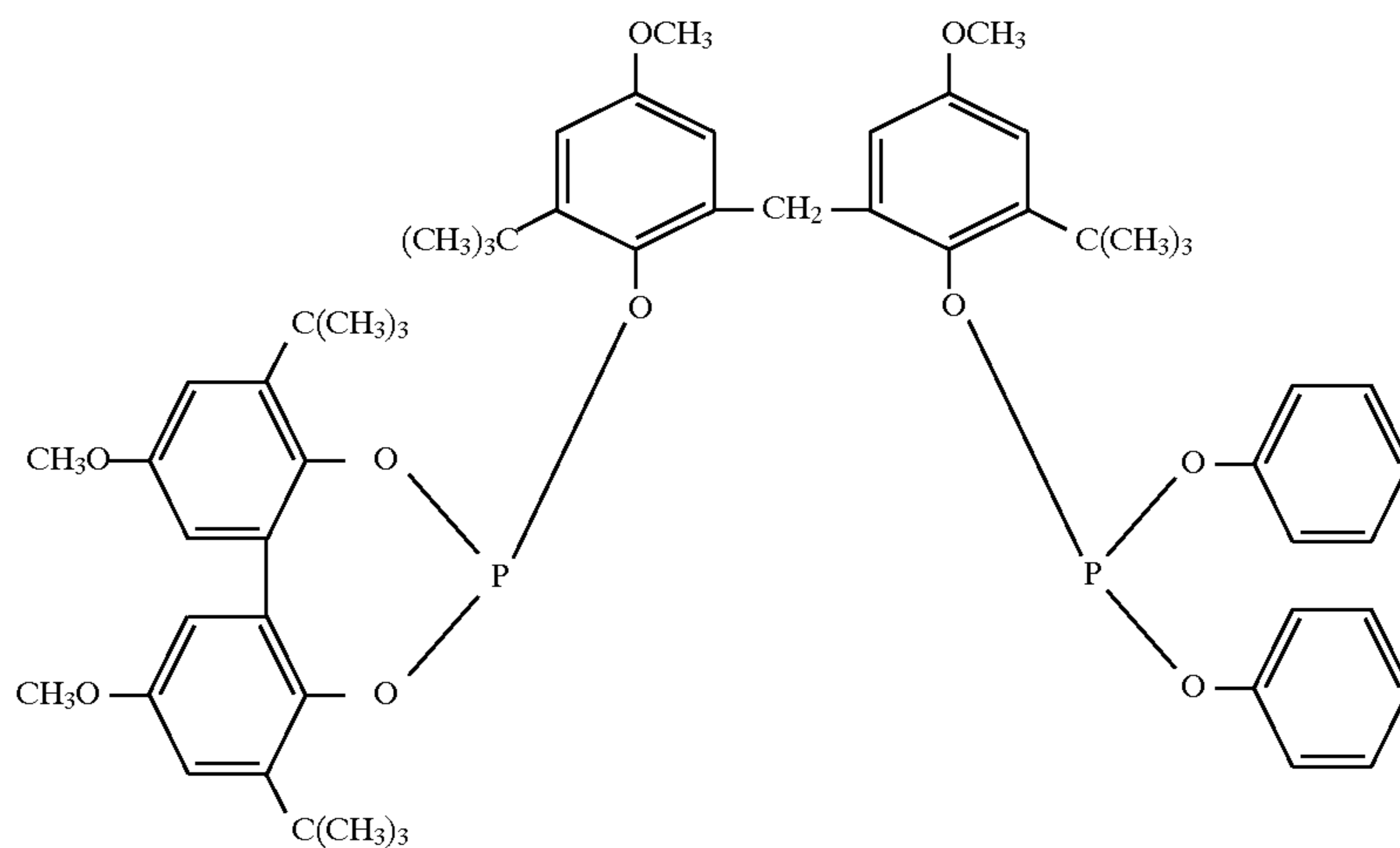
Ligand R
