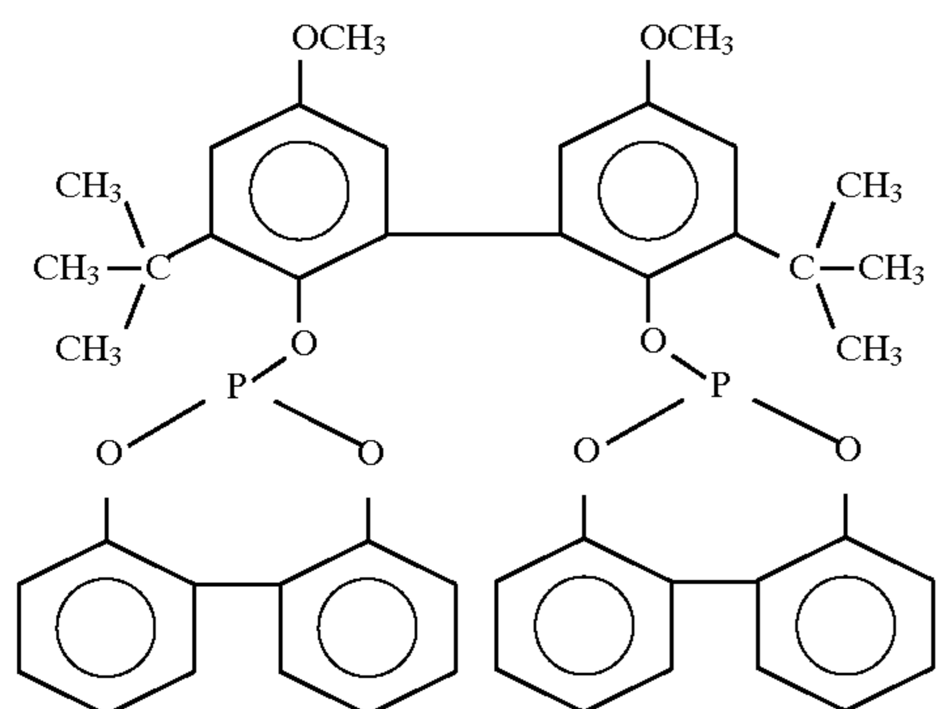
Ligand D 25
