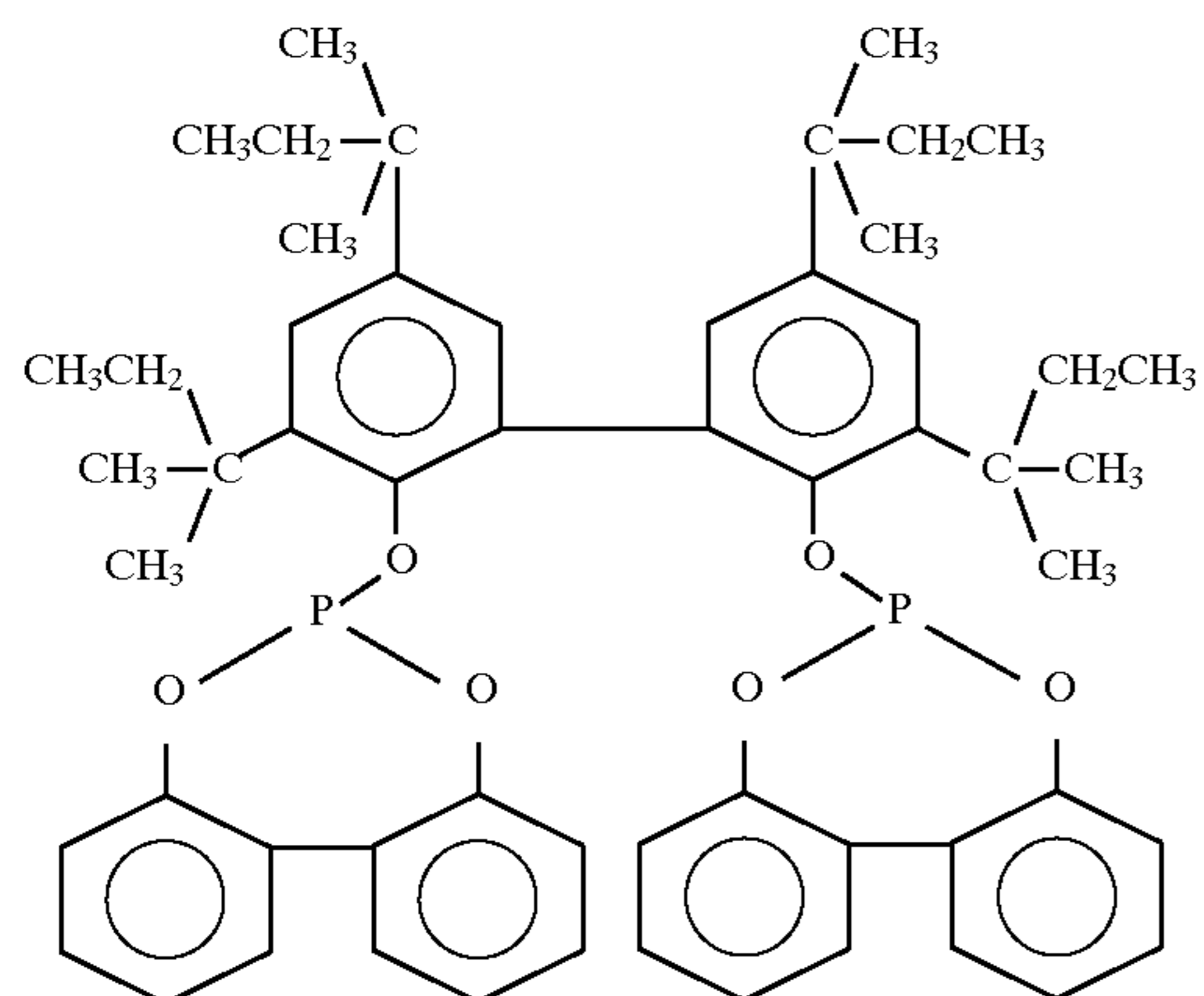
Ligand E 40
