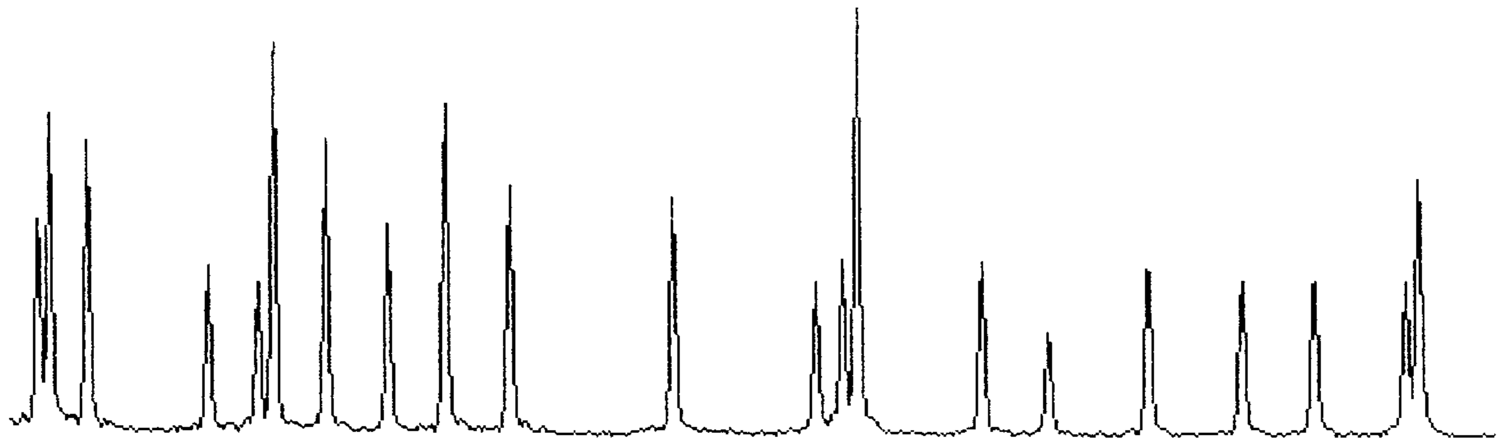
6-FAM-ddCTP 250 pm
