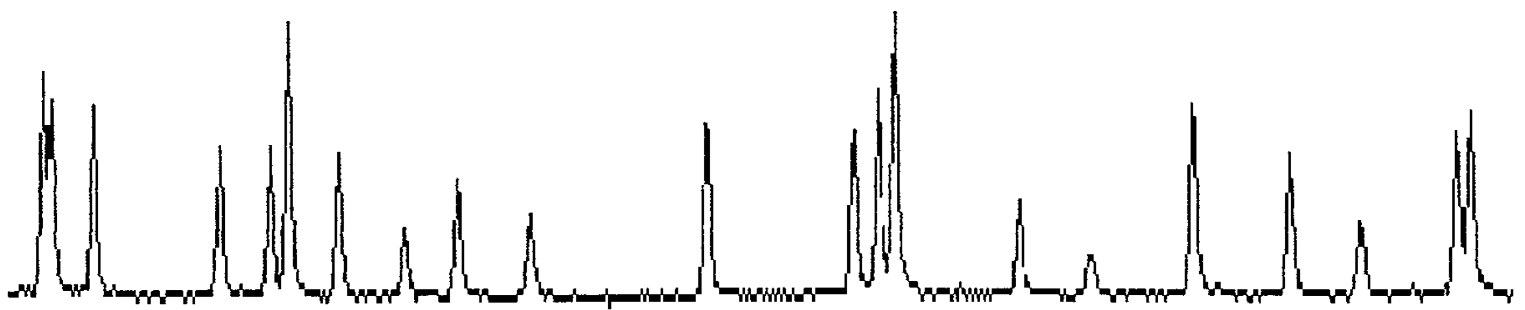
6-FAM-EO-ddCTP 50 pm
