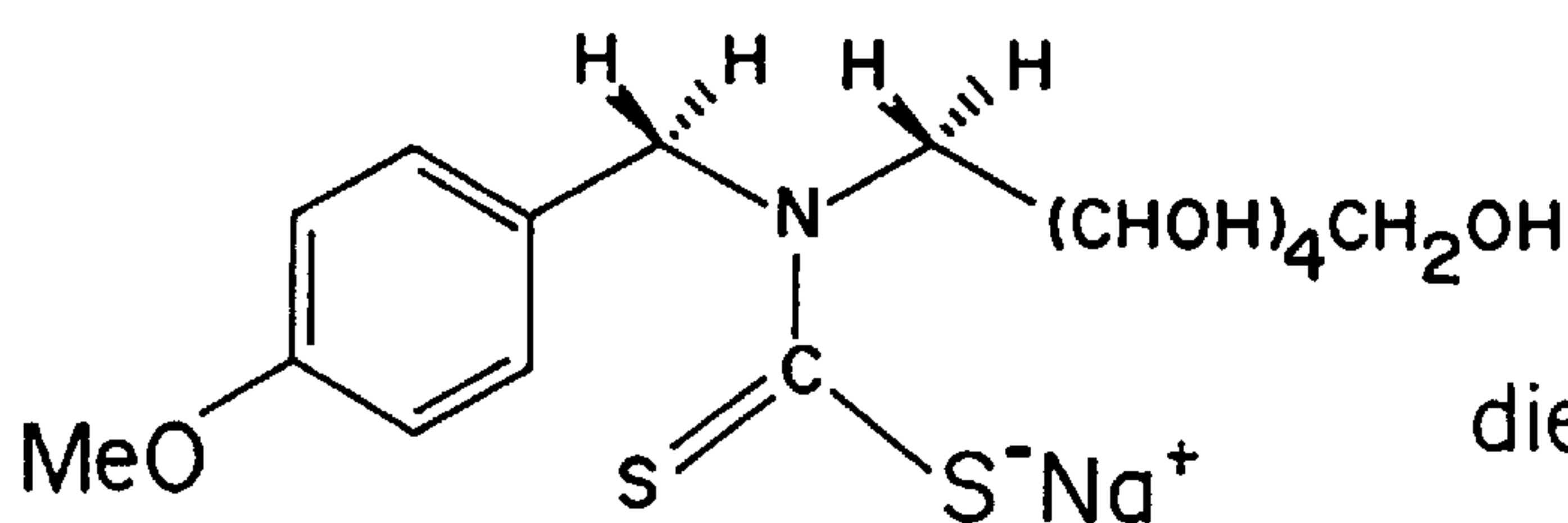
Sodium N -(4-methoxybenzyl)- -D-glucamine- N - carbodithioate
