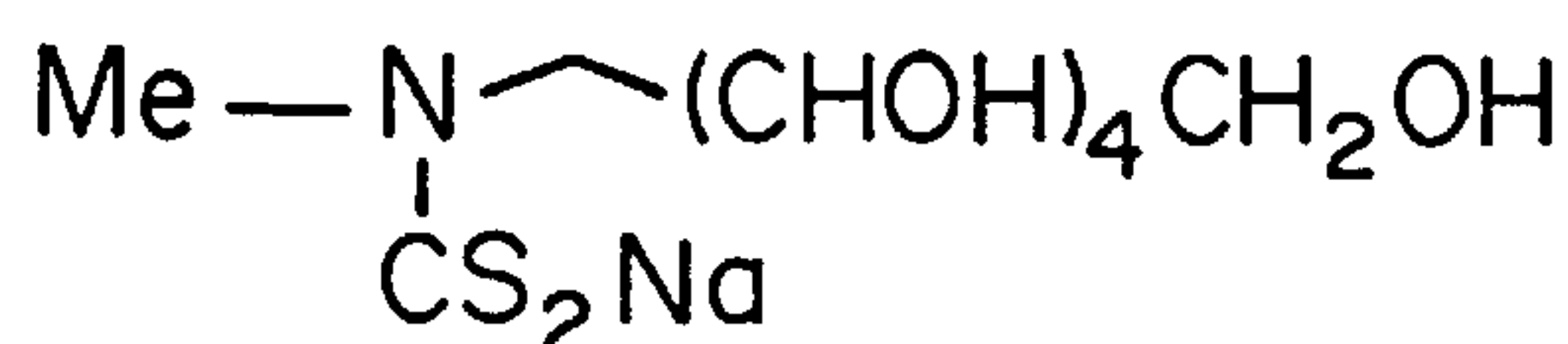
Sodium N -methyl-D- glucamine- N - carbodithioate
