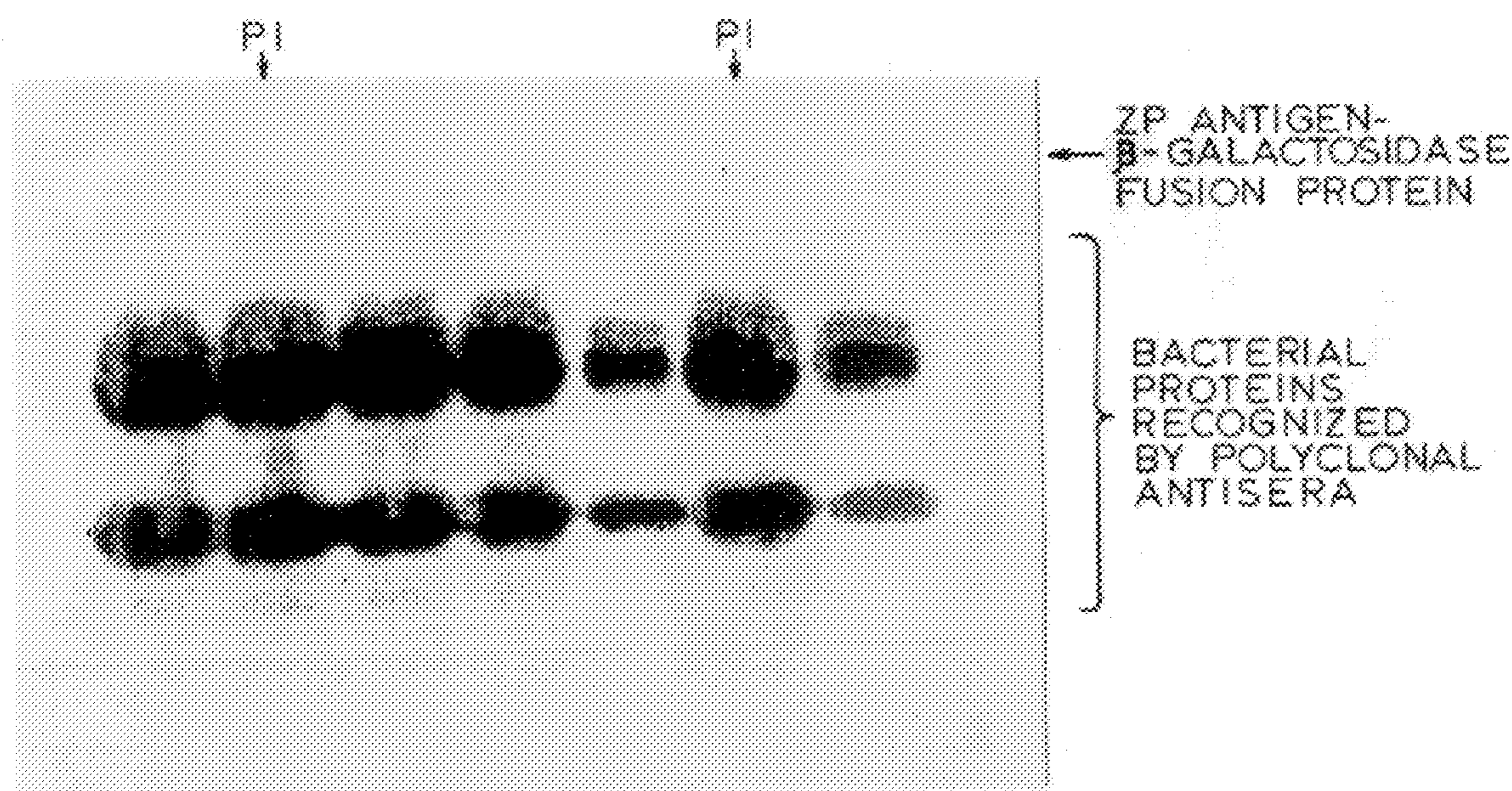
SDS-PAGE IMMUNOBLOT OF PROTEIN EXPRESSED FROM \lambda gt10 DNA FROM CLONE PI PROBED WITH SHEEP ANTISERA TO HEAT SOLUBILIZED ZONA PELLUCIDA
