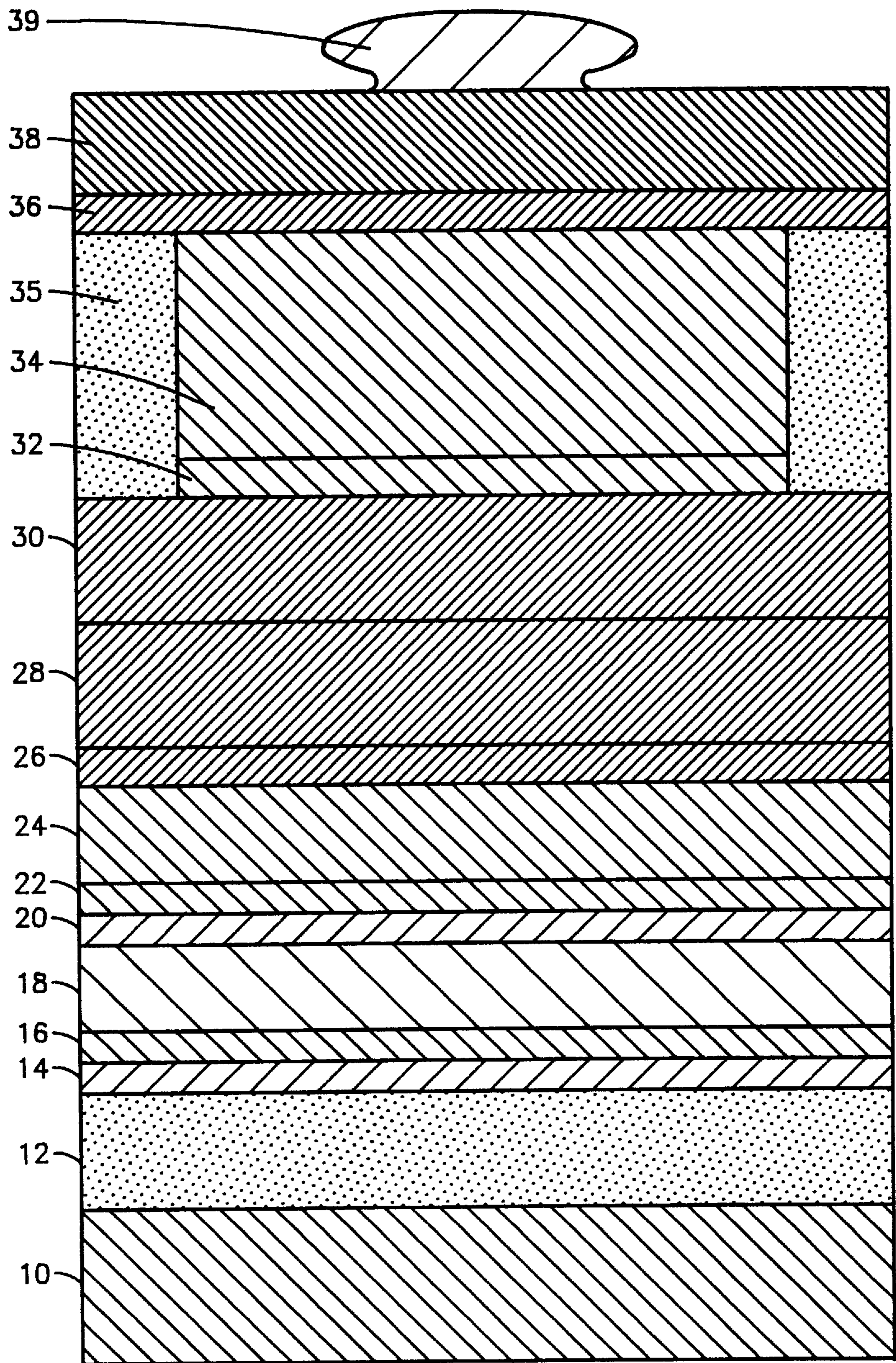
FIG. 1 (PRIOR ART)
