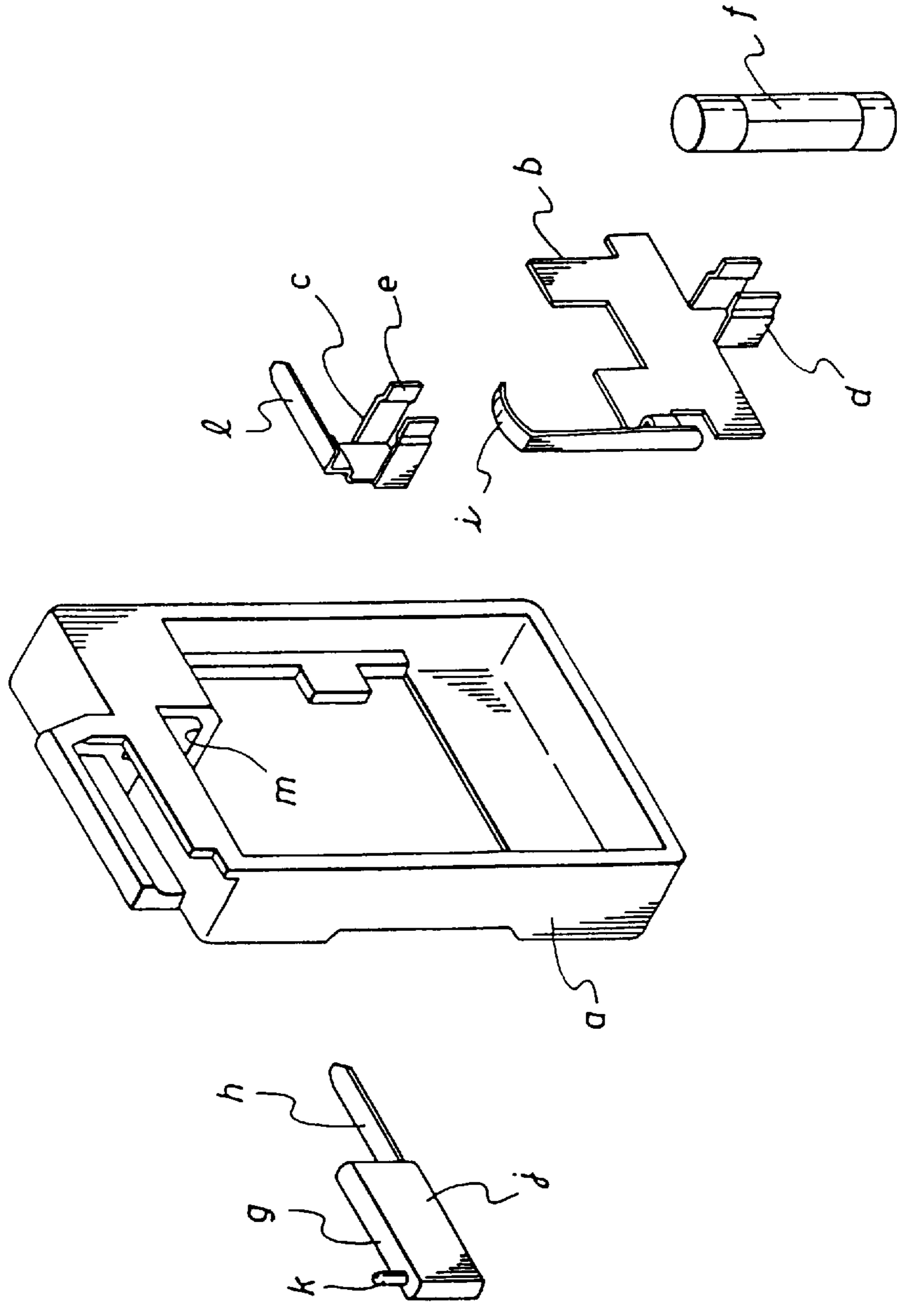
FIG. 63 PRIOR ART
