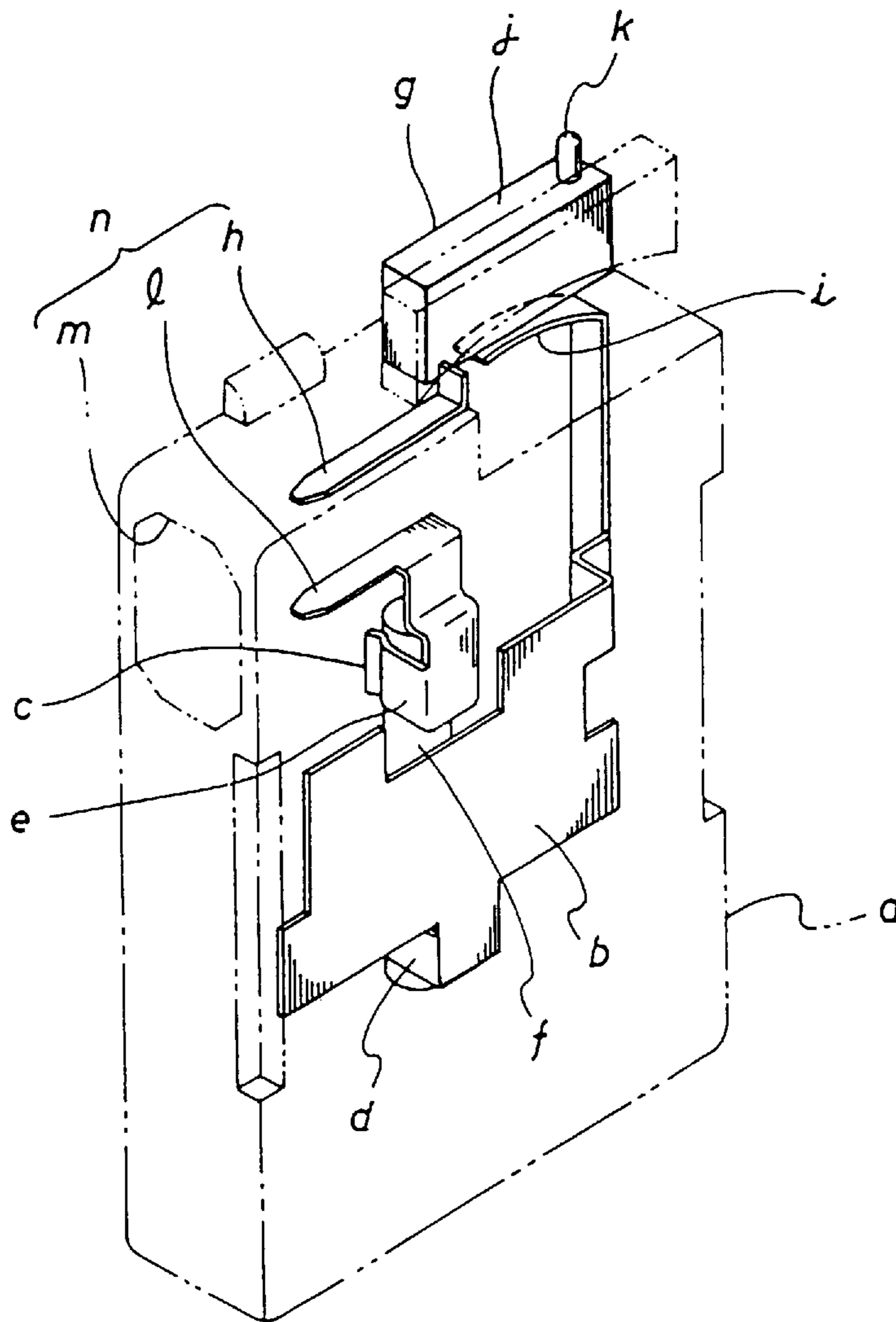
FIG. 62 PRIOR ART
