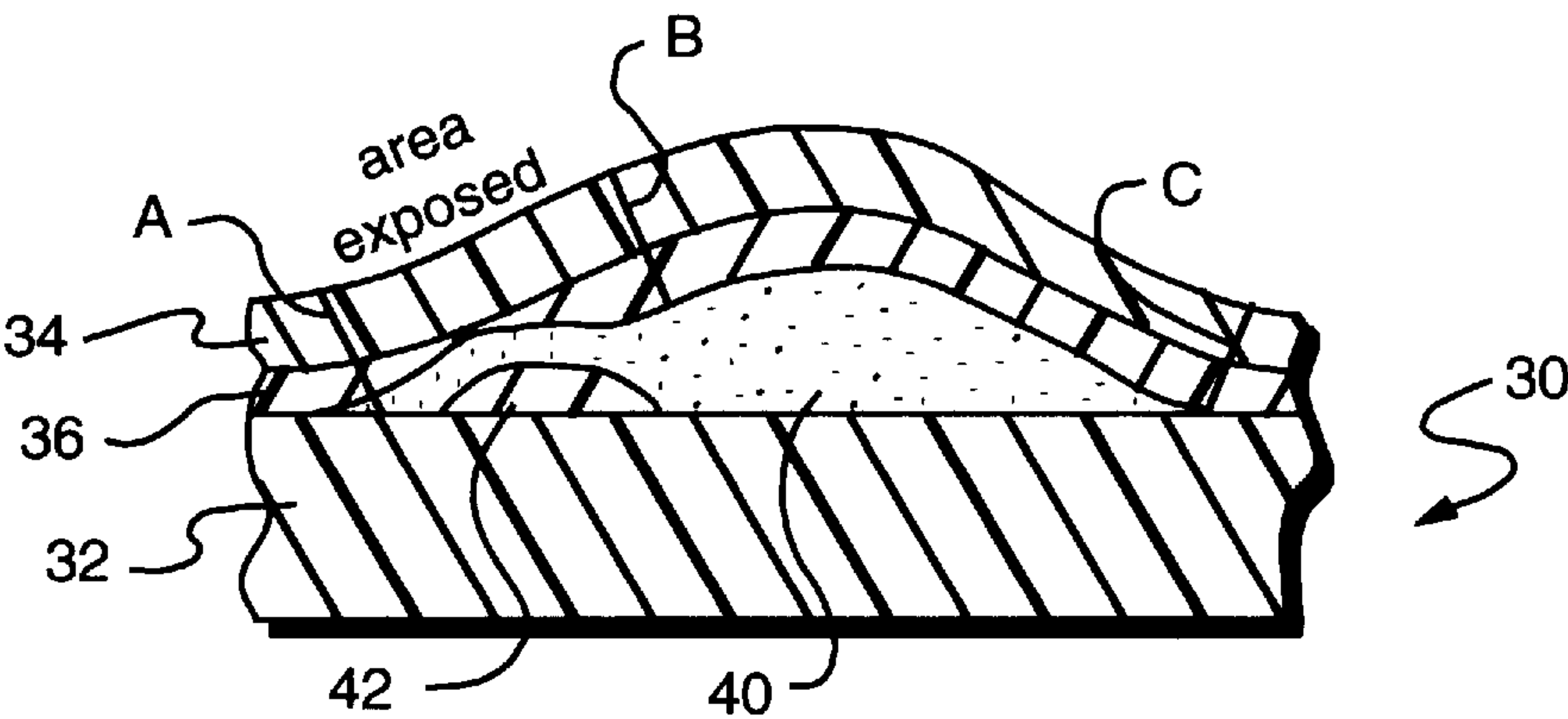
FIG. 1C PRIOR ART
