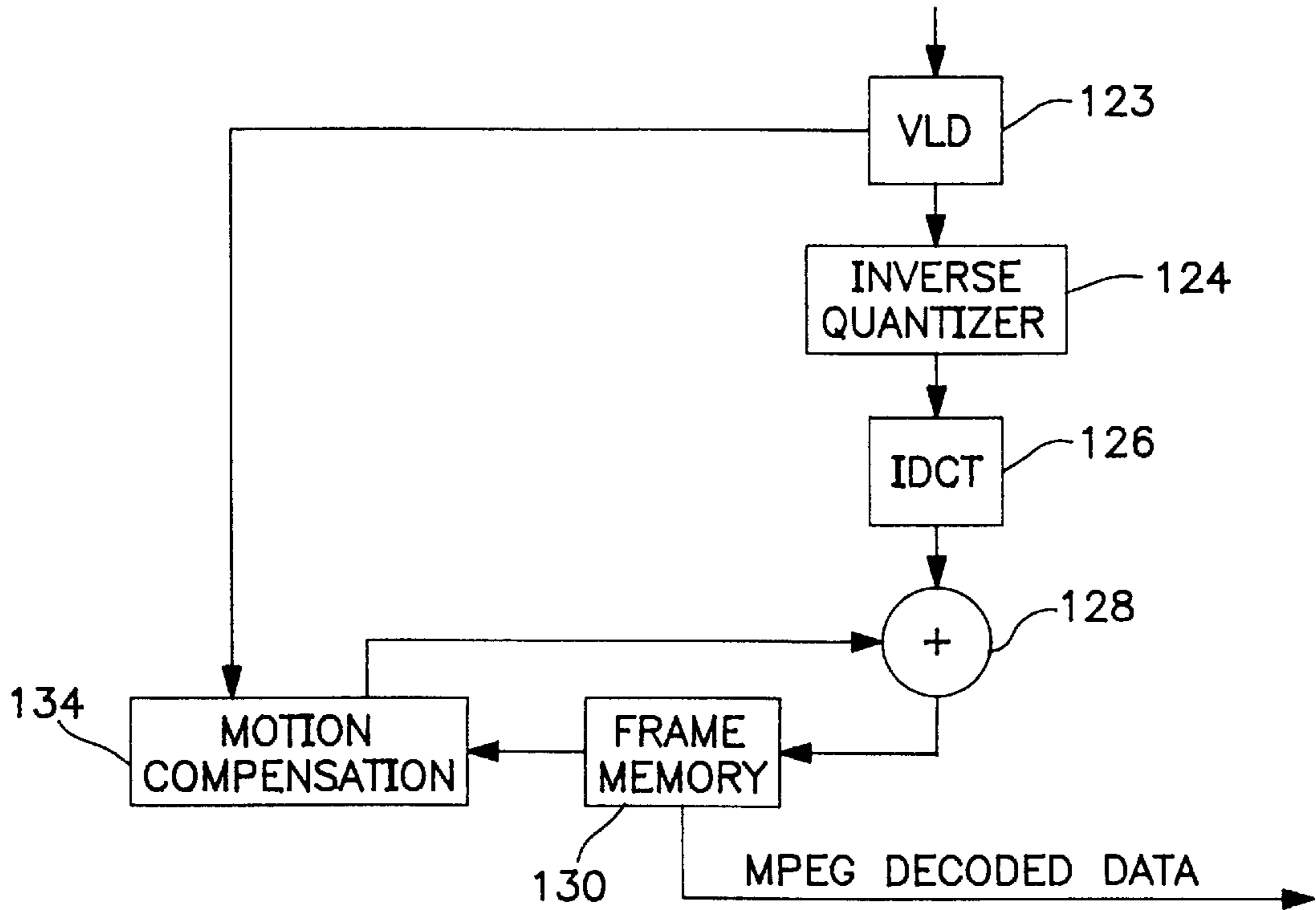
FIG. 3 (PRIOR ART)
