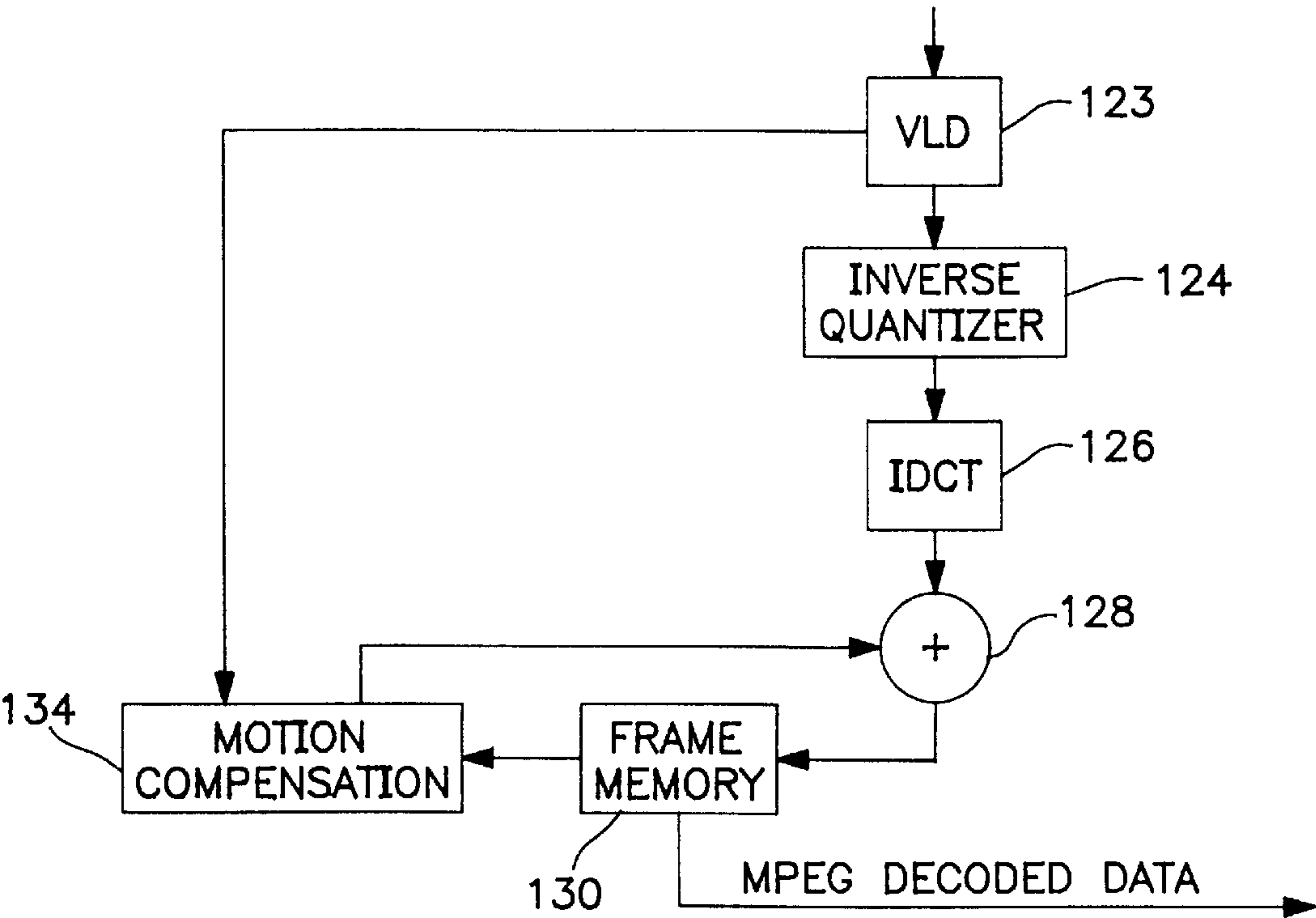
FIG. 3 (PRIOR ART)
