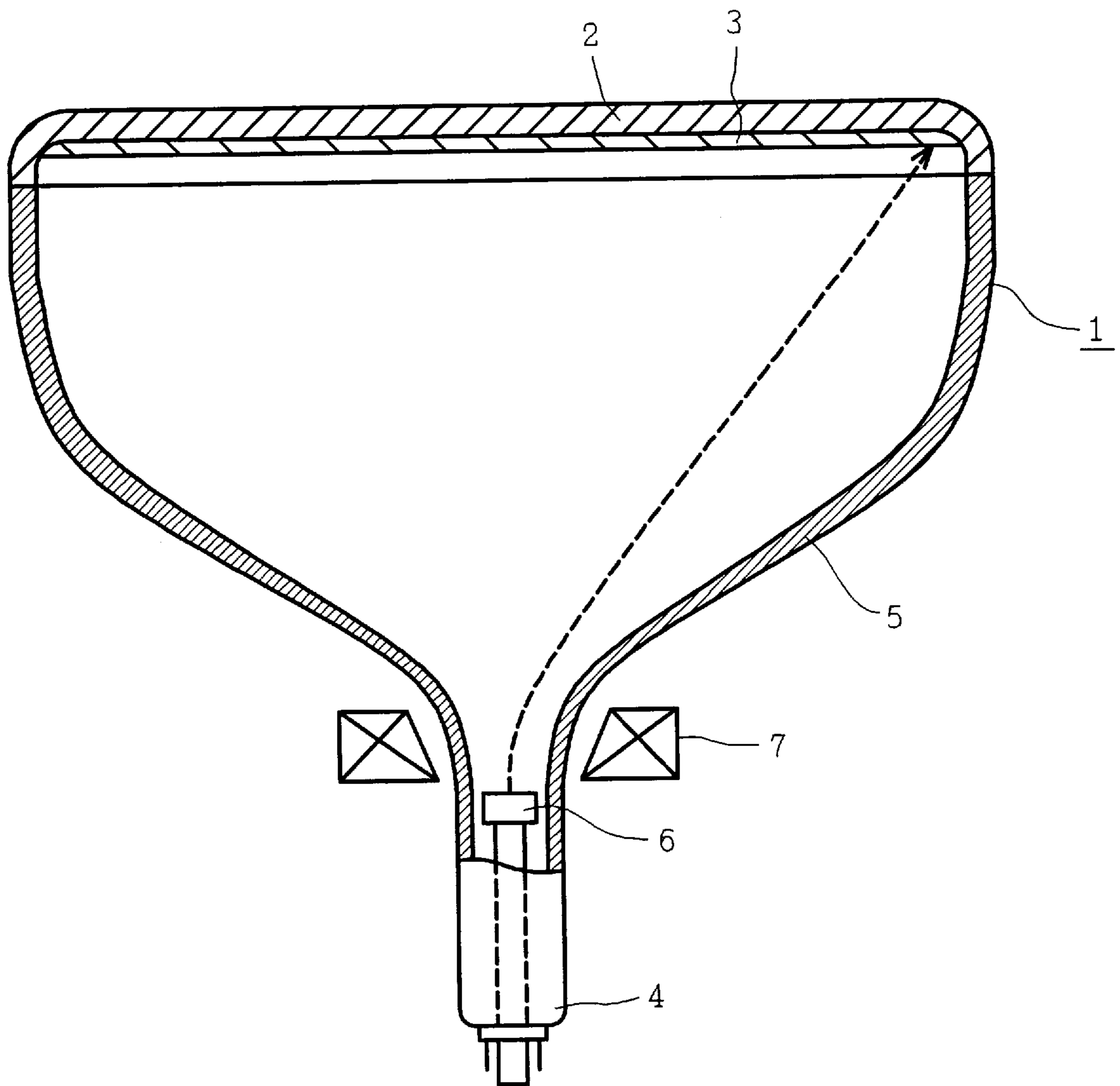
FIG. 7 PRIOR ART
