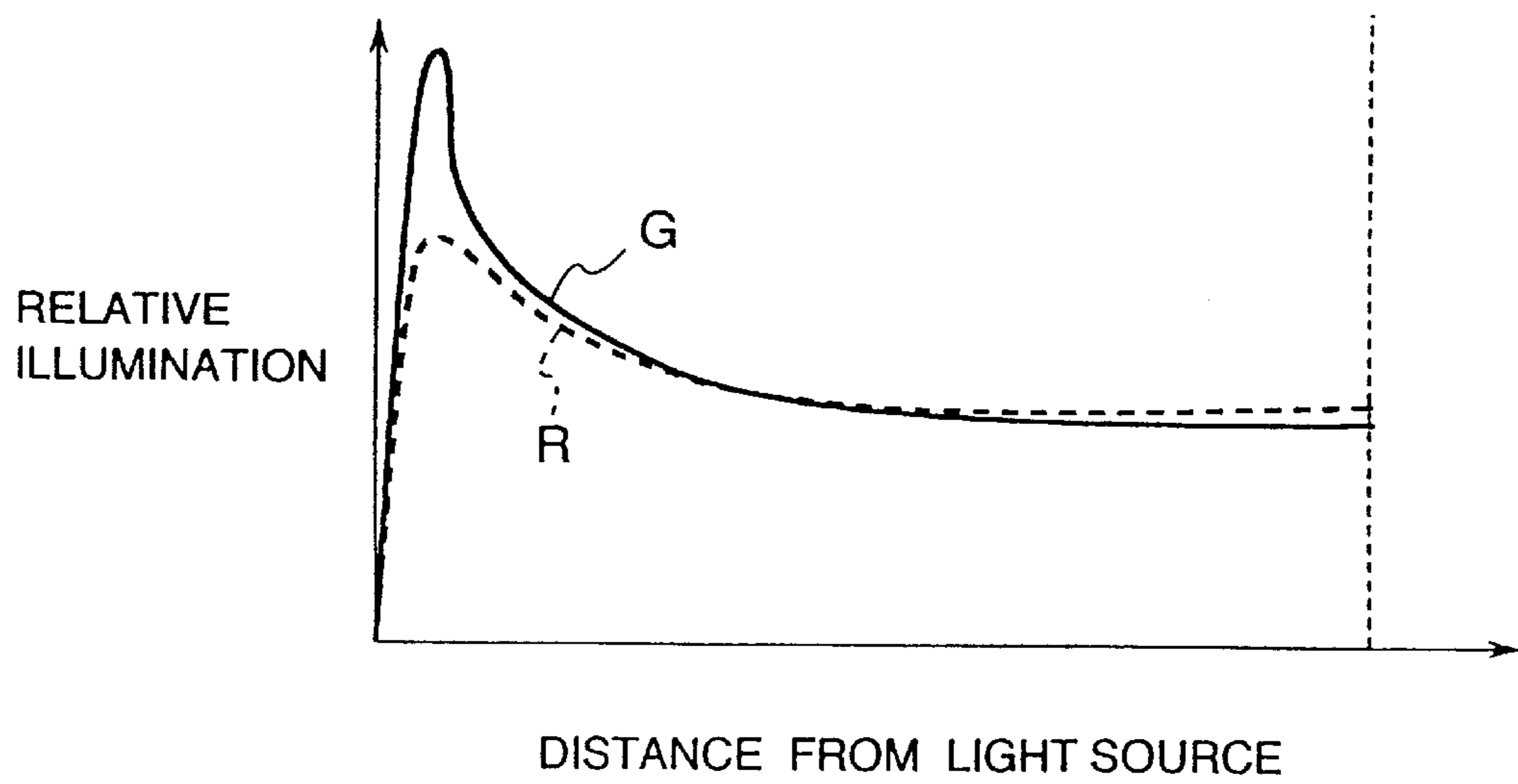
FIG. 1C PRIOR ART
